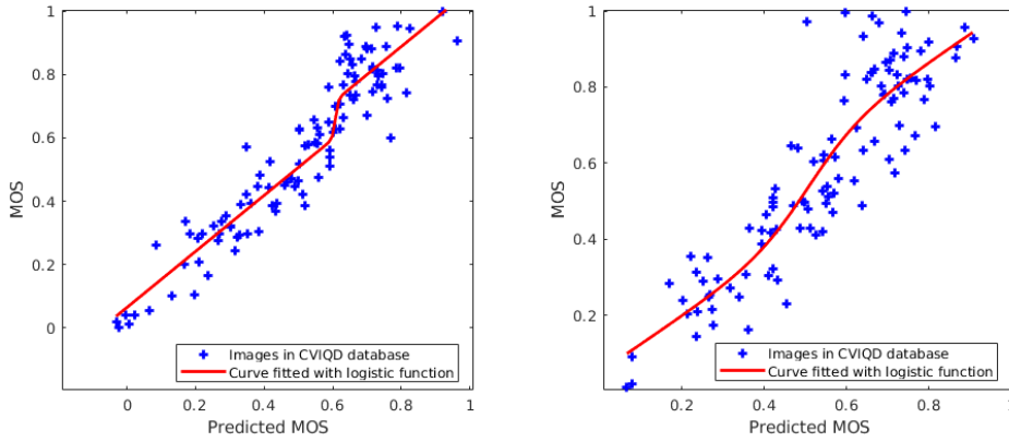
Figure V.5: Scatter plots of predicted quality scores versus MOS of the final model SP360IQA-F-JND (Best performance on the left and worst performance on the right among the VOs).
