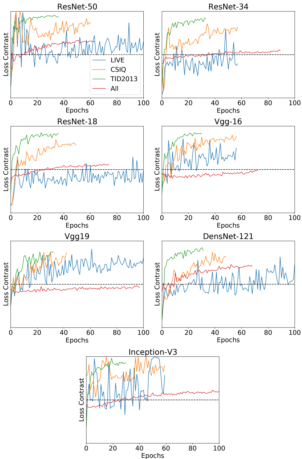
Figure III.10: Contrast (val\_loss - loss) / (val\_loss + loss) between training and validation losses for all models trained on 2D-IQA databases (0 \rightarrow equal loss between training and validation losses). 'All' stands for combined datasets.
