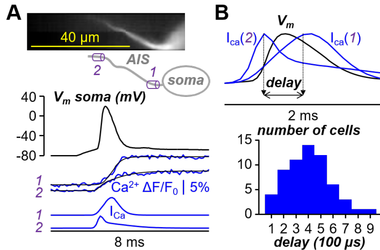
Figure 3.3: Calcium transients in the AIS. A, Top, fluorescence image (OG5N) of the AIS and its reconstruction with a proximal (1) and distal region (2). Bottom, somatic AP and associated \text{Ca}^{2+} transients fitted with a 4-sigmoid (product of four sigmoids) function in 1 and 2; the \text{Ca}^{2+} currents calculated as the time-derivative of the fits are reported below. B, Top, from the experiment in A, \text{Ca}^{2+} currents superimposed to the somatic AP. Bottom, over N = 61 cells tested, distribution of the delay between the distal and the proximal \text{Ca}^{2+} current peaks.
