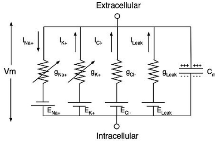
Figure 1.7: Electrical circuit representing a membrane. Where g_{ion} = 1/R_{ion} . g_{Na+} , g_{K+} and g_{Cl-} vary with time and membrane potential, the other components are constant. Adapted from Hodgkin and Huxley (1952a).
