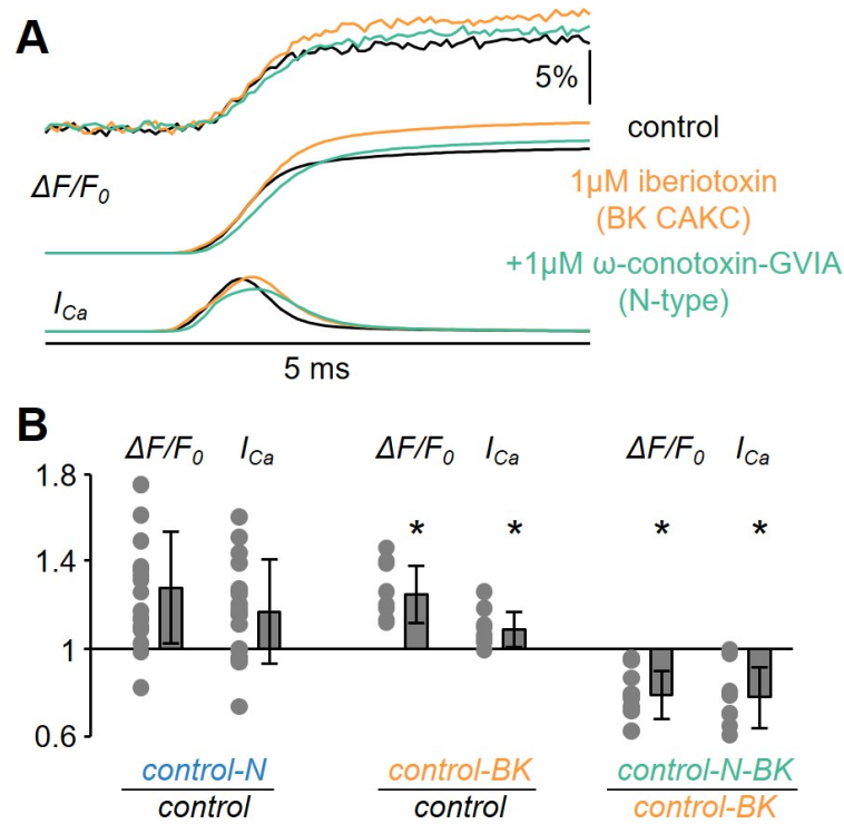
Figure 4.3: Analysis of the blockade of N-type VGCCs after blocking BK CAKCs. A, Representative example of Ca^{2+} transient with 4-sigmoid fit ( \Delta F/F_0 , top traces) and time derivative ( I_{Ca} , bottom traces) in control solution, after local delivery of 1 \mu M of the BK CAKCs inhibitor iberiotoxin and after further delivery of either 1 \mu M of the N-type VGCC inhibitor \omega -conotoxin-GVIA. C, On the left, single values and fractional change with respect to control solution of the maxima of the \Delta F/F_0 and I_{Ca} signals for the blockade of N-type VGCCs (either with \omega -conotoxin-GVIA, N = 18 , \Delta F/F_0 : 1.27 \pm 0.26 , I_{Ca} : 1.17 \pm 0.22 ). On the center, single values and fractional change with respect to control solution of the maxima of the \Delta F/F_0 and I_{Ca} signals for the blockade of BK CAKCs ( N = 9 , \Delta F/F_0 : 1.25 \pm 0.13 , I_{Ca} : 1.09 \pm 0.08 ). On the right, single values and fractional change with respect to the blockade of BK CAKCs only of the maxima of the \Delta F/F_0 and I_{Ca} signals for the combined blockade of N-type VGCCs and BK CAKCs (with \omega -conotoxin-GVIA, N = 9 , \Delta F/F_0 : 0.79 \pm 0.11 , I_{Ca} : 0.78 \pm 0.14 ). “*” indicates that p < 0.01 in paired t-test performed on the signal maxima.
