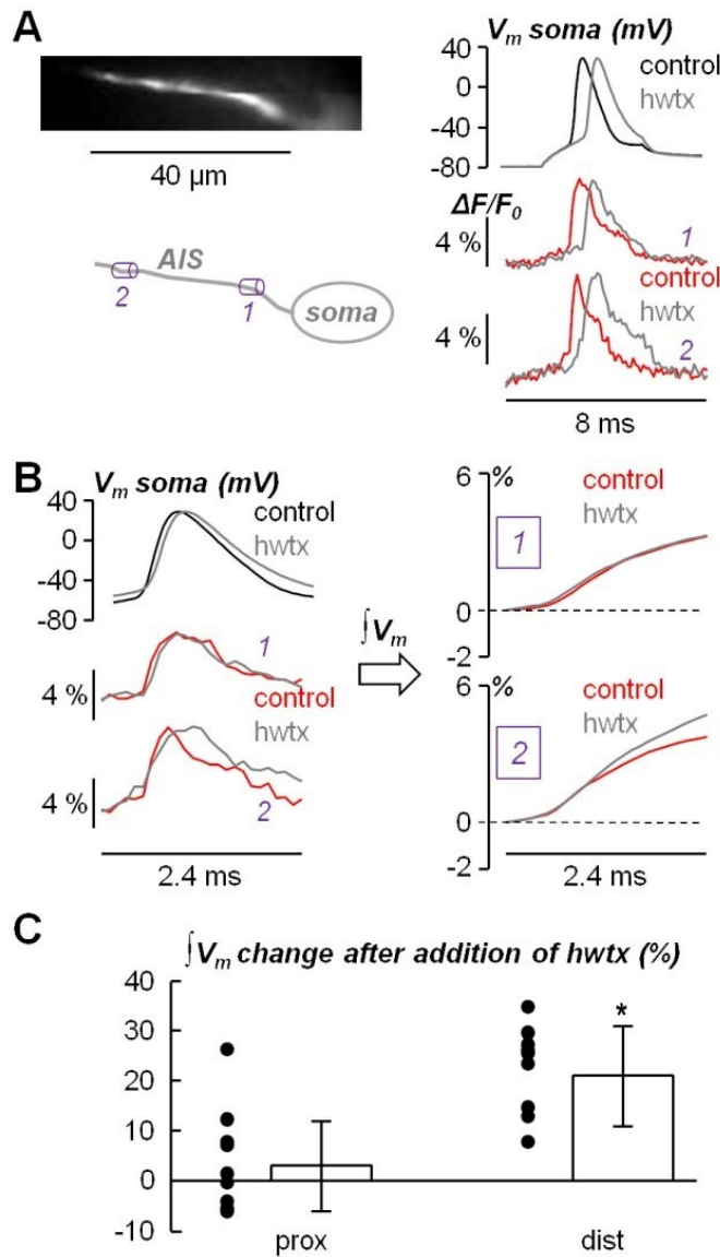
Figure 3.2: Effect of G^1G^4 hwtx (block of Na_v1.2 ) on the AP waveform in the AIS. A, Left, fluorescence image (voltage sensitive dye JPW1114) of the AIS and its reconstruction with a proximal region (1) and a distal region (2) indicated. Right, Somatic AP in control solution and after locally delivering 80 nM of G^1G^4 hwtx (hwtx) (top) and associated V_m transients in 1 and 2. B, Left, somatic and axonal APs at a different time scale (2.4 ms duration) visually indicating a widening of the AP waveform, in the distal position only, after locally delivering G^1G^4 hwtx. Right, quantification of the AP waveform shape by calculation of V_m integral ( \int V_m ) over the 2.4 ms time window comprising the AP signal. C, Single cell values and percentage change ( N=9 cells) of the \int V_m signal maximum after locally delivering G^1G^4 hwtx in proximal regions (mean \pm SD = 3.2 \pm 8.8), and in distal regions (mean \pm SD = 21.3 \pm 10.5). "*" indicates a significant change ( p < 0.01 , paired t-test).
