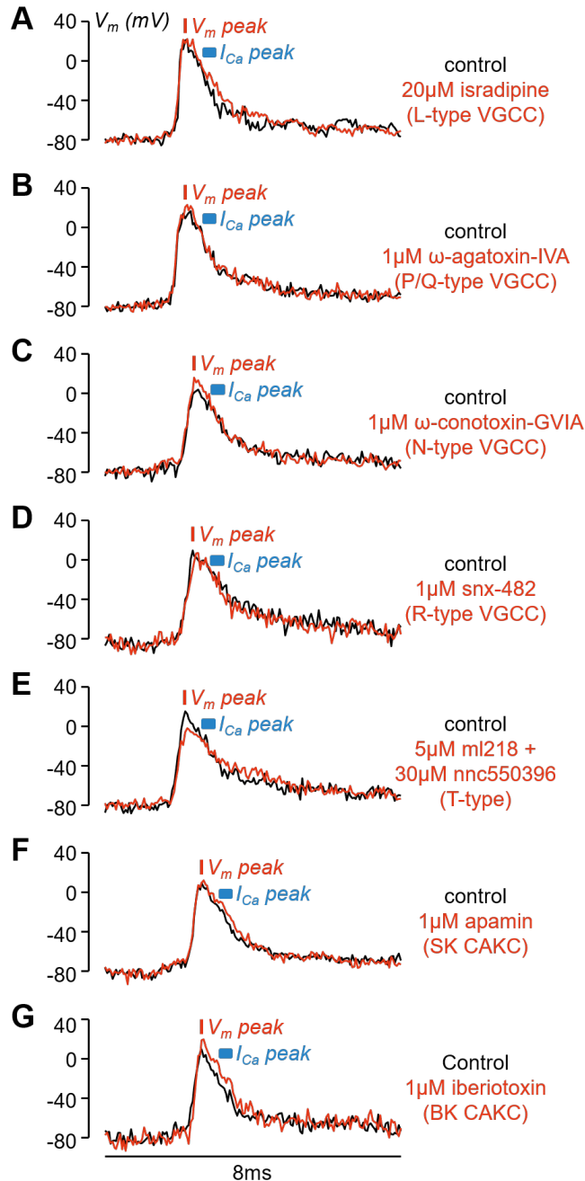
Figure 4.5: Examples of the effects of the diverse VGCC and CAKC blockades on the bAP shape. A, Optical V_m transient from an apical dendrite region ( \sim 100 \mu m from the soma) in a representative L5 pyramidal neuron in control conditions (black trace) and after blocking L-type VGCCs with 20 \mu M isradipine (red trace). B, Representative experiment as in A, but by blocking P/Q-type VGCCs with 1 \mu M \omega -agatoxin-IVA. C, Representative experiment as in A, but by blocking N-type VGCCs with 1 \mu M \omega -conotoxin-GVIA. D, Representative experiment as in A, but by blocking R-type VGCCs with 1 \mu M snx-482. E, Representative experiment as in A, but by blocking T-type VGCCs with 5 \mu M ml218 and 30 \mu M nnc550396. F, Representative experiment as in A, but by blocking SK CAKCs with 1 \mu M apamin. G, Representative experiment as in A, but by blocking BK CAKCs with 1 \mu M iberiotoxin. In each cell the red bar shows the timing of the AP peak and the blue segment the expected range for the peak of the Ca^{2+} current (500-800 \mu s after the AP peak).
