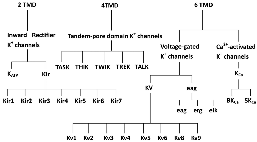
Figure 1.5: Classification of potassium ion channels. TMD, transmembrane domain; K_{ATP} , ATP-sensitive K^+ channel; Kir, inward-rectifier channel; K_v , voltage-gated K^+ channel; EAG, ether-á-go-go channel; K_{Ca} , Ca^{2+} -activated channel; BK_{Ca} , large conductance K_{Ca} channel; SK_{Ca} , small conductance K_{Ca} channel. From Zhong et al. (2013).
