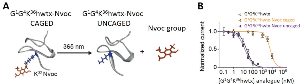
Figure 2.13: Selectivity of \text{G}^1\text{G}^4\text{K}^{36}\text{Huwentoxin-IV-Nvoc} . A, Photolysis of \text{G}^1\text{G}^4\text{K}^{36}\text{Hwtx-Nvoc} by illumination at 365 nm. B, Light-induced inhibition of \text{Na}_v1.6 current by uncaged \text{G}^1\text{G}^4\text{K}^{36}\text{Hwtx-Nvoc} analog (100 nM).
