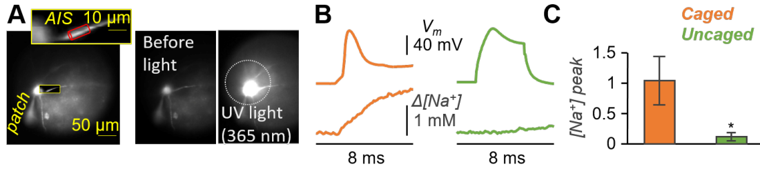
Figure 2.16: Sodium imaging with \text{G}^1\text{G}^4\text{K}^{36}\text{hwtX-Nvoc} . A, left, L5 pyramidal neuron filled with 500 \mu\text{M} of the \text{Na}^+ indicator ING-2; the patch pipette filling the cell is visible; outlined in yellow the AIS area of \Delta[\text{Na}^+] measurement; right, images taken before and during the uncaging pulse of UV light illustrating the area of photolysis. B, left, somatic AP (top) and associated \Delta[\text{Na}^+] signal over the red cylinder depicted in panel A (bottom) in the presence of caged \text{G}^1\text{G}^4\text{K}^{36}\text{hwtX-Nvoc} ; right, after uncaging the toxin, V_m transient depolarizing the cell to the AP peak (top) and associated \Delta[\text{Na}^+] signal (bottom). C, mean \pm SEM ( n = 4 cells) of the \Delta[\text{Na}^+] signal maximum (peak) before and after uncaging the toxin. "*" indicates a significant decrease ( p < 0.01 , paired t-test).
