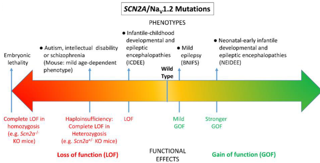
Figure 5.2: Spectrum of mutations and phenotypes for SCN2a /Na v 1.2. A, Mild gain of function induced by SCN2a mutations cause benign neonatal-infantile familial seizures (BNIFS). Larger gain of function mutations cause neonatal-early infantile developmental and epileptic encephalopathies (NEIDEE). Loss of function mutations cause infantile-childhood developmental and epileptic encephalopathies (ICDEE). Haploinsufficiency or complete loss of function in heterozygosis leads to behavioural/cognitive phenotypes without epilepsy such as autism spectrum disorder (ASD), intellectual disability or schizophrenia. Haploinsufficiency in Scn2a +/- mice causes a relatively mild and age-dependent phenotype including short absence-like seizures, autistic/schizophrenic traits and memory dysfunctions. Homozygote Scn2a -/- knock-out mice show embryonic mortality. Figure from Mantegazza et al. (2021).
