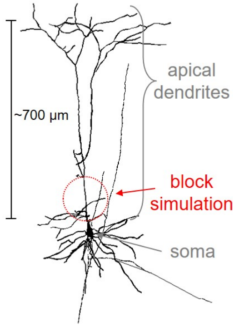
Figure 4.8: Morphology of the layer 5 pyramidal neuron model in NEURON. Soma and apical dendrite are indicated in grey. When simulating a specific channel block we decreased the density of the specific channel with 90%. The area of the simulated spread of the blocker is indicated in red.
