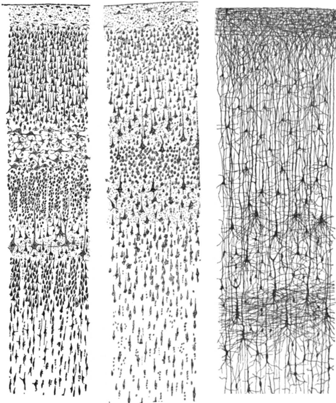
Figure 1.1: Drawing from cortical cells by Ramón y Cajal. Three different drawings side by side from a cross section of the neocortex. At the top layer I, at the bottom layer VI. From Newman et al. 2017
