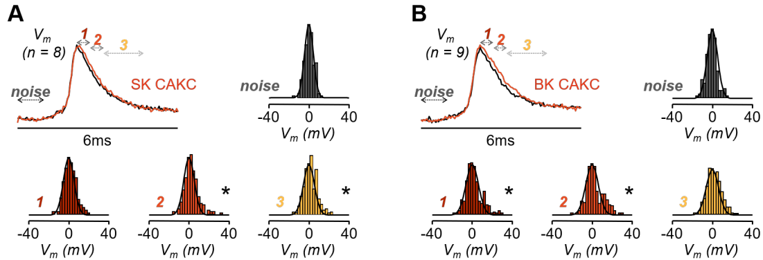
Figure 4.7: Analysis of the effect of the diverse CAKCs on the bAP shape. Same analysis as in figure 4.6, where the signal is divided into bins of 500 \mu s after the voltage peak (1), 500 \mu s around the expected calcium current peak (2), 1500 \mu s after the expected calcium current peak (3) and 1000 \mu s noise. A, Averaged signals aligned to the AP peak from N = 8 cells in control conditions (black trace) and after blocking SK CAKCs (red trace) and histograms of the sample differences in the illustrated four time windows; normal distributions with mean and standard deviations calculated from the points are reported (red plots) for comparison with the histograms. B, Same as in A, but in 9 cells where BK CAKs were blocked. “*” indicates that the distribution deviates from normality ( p < 0.01 , Lilliefors test).
