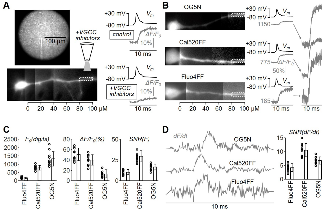
Figure 2.10: Performance of Fluo4FF, OG5N and Cal520FF for ultrafast \text{Ca}^{2+} imaging and optical recording of \text{Ca}^{2+} currents. A, Image of a brain (cortical) slice with patched L5 pyramidal neuron. On the bottom, a fluorescence image of a neuron loaded with 2 mM OG5N with a region of interest (white-dotted rectangle) indicated; a pipette locally delivering a cocktail of VGCC inhibitors (see main text) is drawn to indicate its position. On the right: somatic V_m with evoked AP and associated \text{Ca}^{2+} - \Delta F/F_0 signal in control condition and after locally delivering the VGCC inhibitors showing the block of the \text{Ca}^{2+} transient and no effect on the somatic AP. B, Left: fluorescence images of L5 pyramidal neurons loaded with 2 mM of either Fluo4FF (bottom), Cal520FF (middle) or OG5N (top); the white-dotted rectangles outline the regions (80–100 \mu\text{m} from the soma) from where fluorescence was averaged. Centre: \Delta F/F_0 signals (grey) associated with an AP (black); the camera digits corresponding to F_0 are indicated. Right: the normalised \Delta F/F_0 signals showing the different S/N. C, Left: F_0 values (digits) in 10 cells for each indicator and mean \pm SD for Fluo4FF (174 \pm 48), Cal520FF (780 \pm 139) and OG5N (1325 \pm 425). Centre: maximum \Delta F/F_0 (%) values in the 10 cells and mean \pm SD for Fluo4FF (51 \pm 12), Cal520FF (40 \pm 10) and OG5N (13 \pm 8). Right: \Delta F/F_0 S/N values in the 10 cells and mean \pm SD for Fluo4FF (10.3 \pm 3.0), Cal520FF (29.5 \pm 6.6) and OG5N (16.5 \pm 3.5). D, Left: normalised time-derivative of F after smoothing ( dF/dt ) in the three cells of panel A. Right: dF/dt S/N values in the 10 cells and mean \pm SD for Fluo4FF (4.2 \pm 1.4), Cal520FF (10.5 \pm 2.4) and OG5N (6.8 \pm 1.3). All data are from averages of 9 trials (Figure from (Blömer et al. 2021b))
