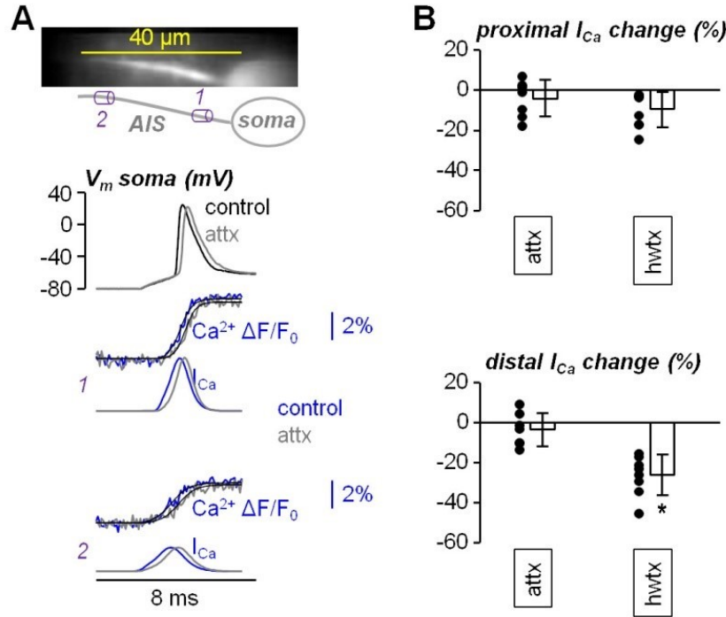
Figure 3.11: Analysis of the effect of attx on the \text{Ca}^{2+} influx in the AIS. A, Top, \text{Ca}^{2+} fluorescence image (OG5N) of the AIS and its reconstruction with a proximal region (1) and a distal (2) region indicated. Bottom, somatic AP and associated \text{Ca}^{2+} transients and currents in 1 and 2 in control solution and after locally delivering 800 nM attx. B, Top, single values and percentage change of the proximal \text{Ca}^{2+} current peak after addition of attx (N = 7 cells, mean \pm SD = -4.5 \pm 9.2 ). Right, in the same cells, single values and percentage change of the distal \text{Ca}^{2+} current peak after addition of attx (mean \pm SD = -3.6 \pm 8.3 ); the values and statistics of the equivalent experiments with \text{G}^1\text{G}^4\text{hwtx} (hwtx) (figure 3.3A) are reported for comparison; "*" indicates a significant change ( p < 0.01 , paired t-test).
