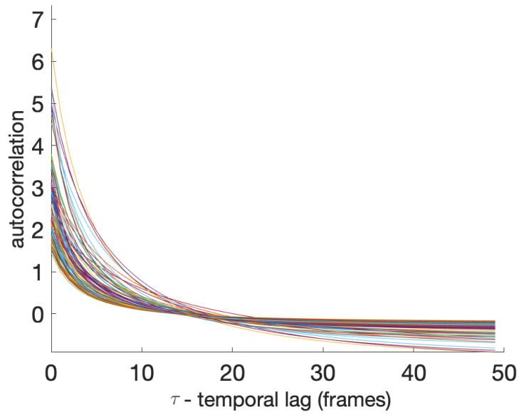
Figure 2.9 – Influence of model parameters on the autocorrelation function for model G_2 . Each curve illustrates the simulation of model G_2 for a pair of values (D, \sigma_{\text{PSF}}^2) , all other parameters being fixed to the default values.
