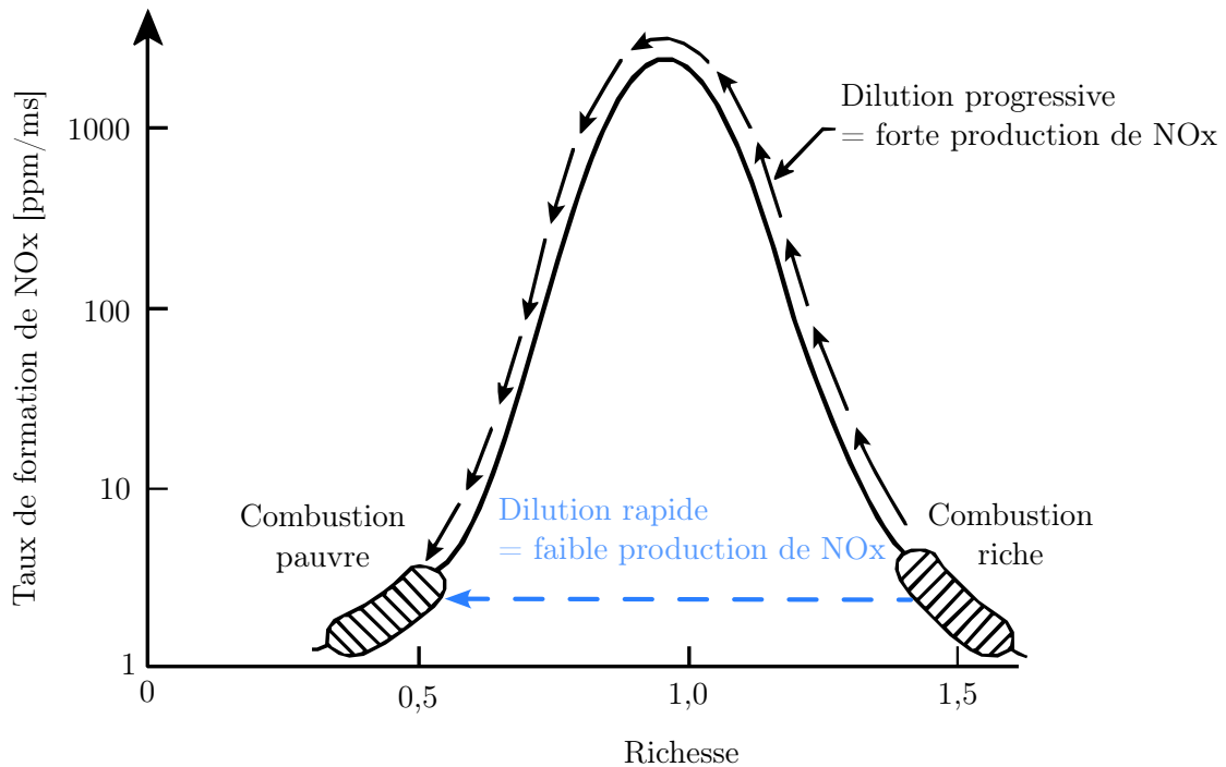
FIGURE 1.2 – Principe de la combustion RQL [18]
