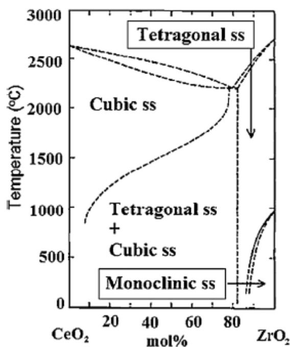
FIGURE 2: PHASE DIAGRAM OF \text{CeO}_2 - \text{ZrO}_2 [26]
