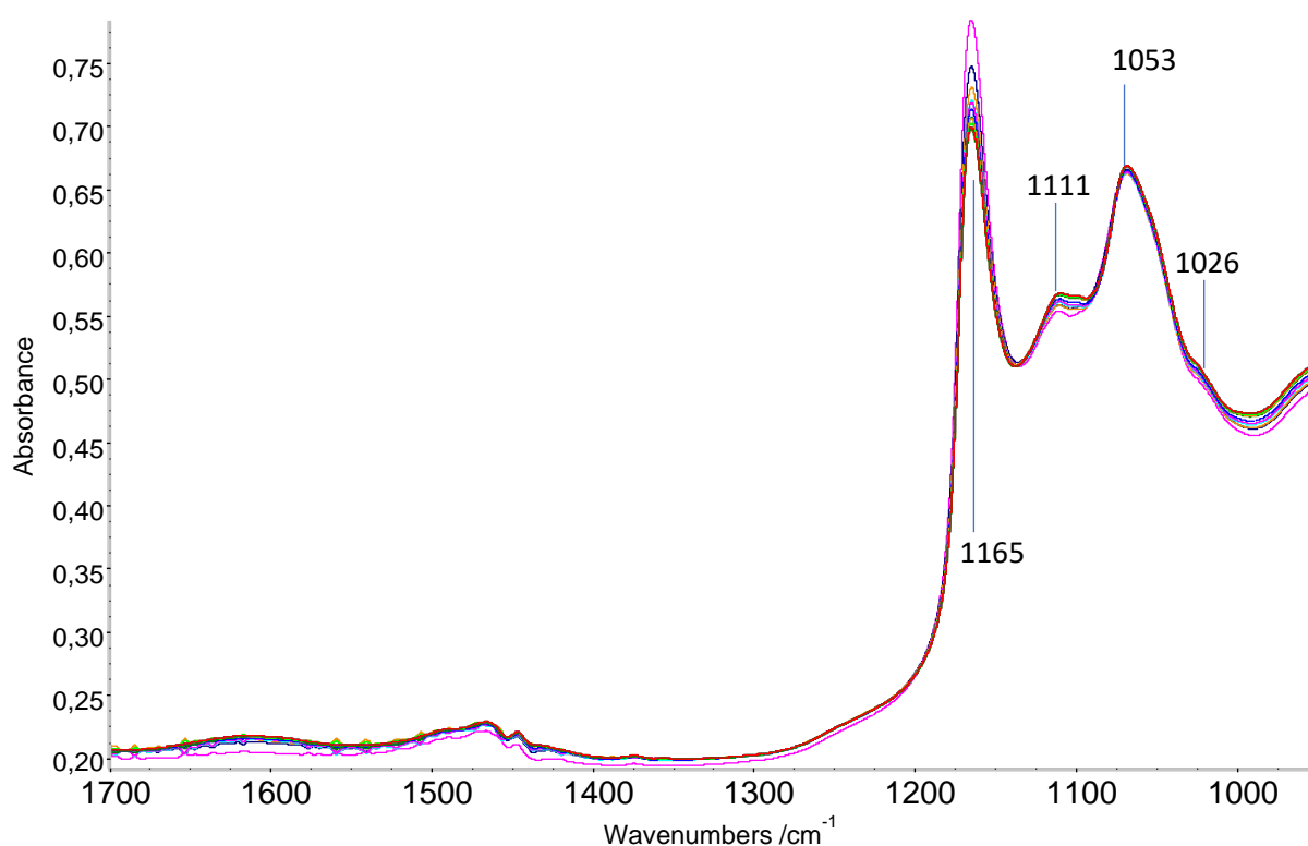
Figure SI 4 : Evolution of the species formed over Pre-reduced CZ(0-100) covered with methoxys and after introduction of a small O_2 equilibrium pressure followed by IR at room temperature.
