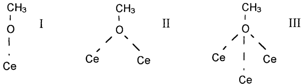
FIGURE 7 DIFFERENT TYPES OF METHOXY SPECIES FORMING ON THE SURFACE OF CERIA AFTER METHANOL ADSORPTION
