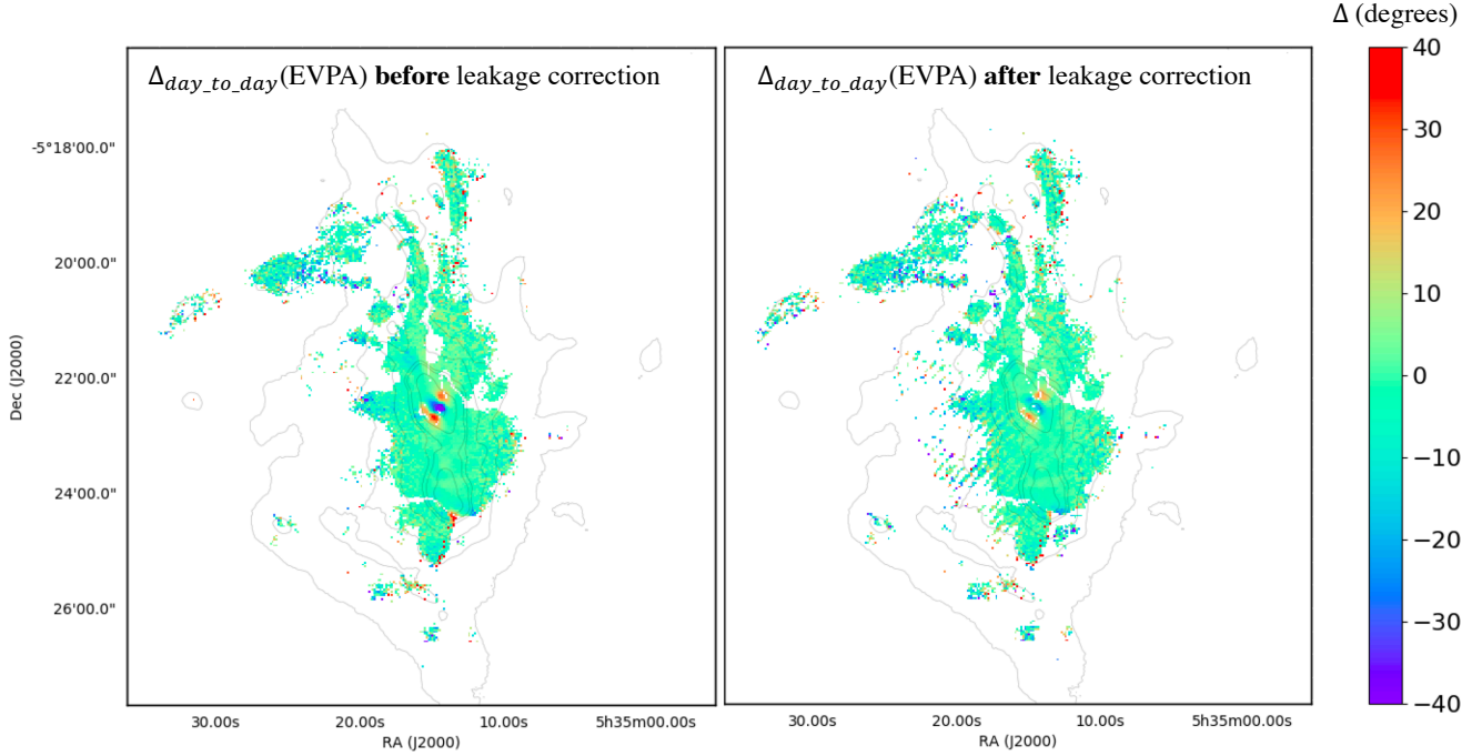
Figure 4.29: The left map shows the difference in polarization angles before applying the leakage correction. The weakly polarized Orion-KL is affected by the leakage and makes \Delta_{day-to-day} significantly different from one day to another (these data were taken four days apart). The data used here were taken under different weather conditions, elevation, and focus positions. Uranus observations were carried out before each OMC-1 observation. The right panel shows \Delta_{day-to-day} after leakage correction. Here we corrected each data set by a suitable leakage.
