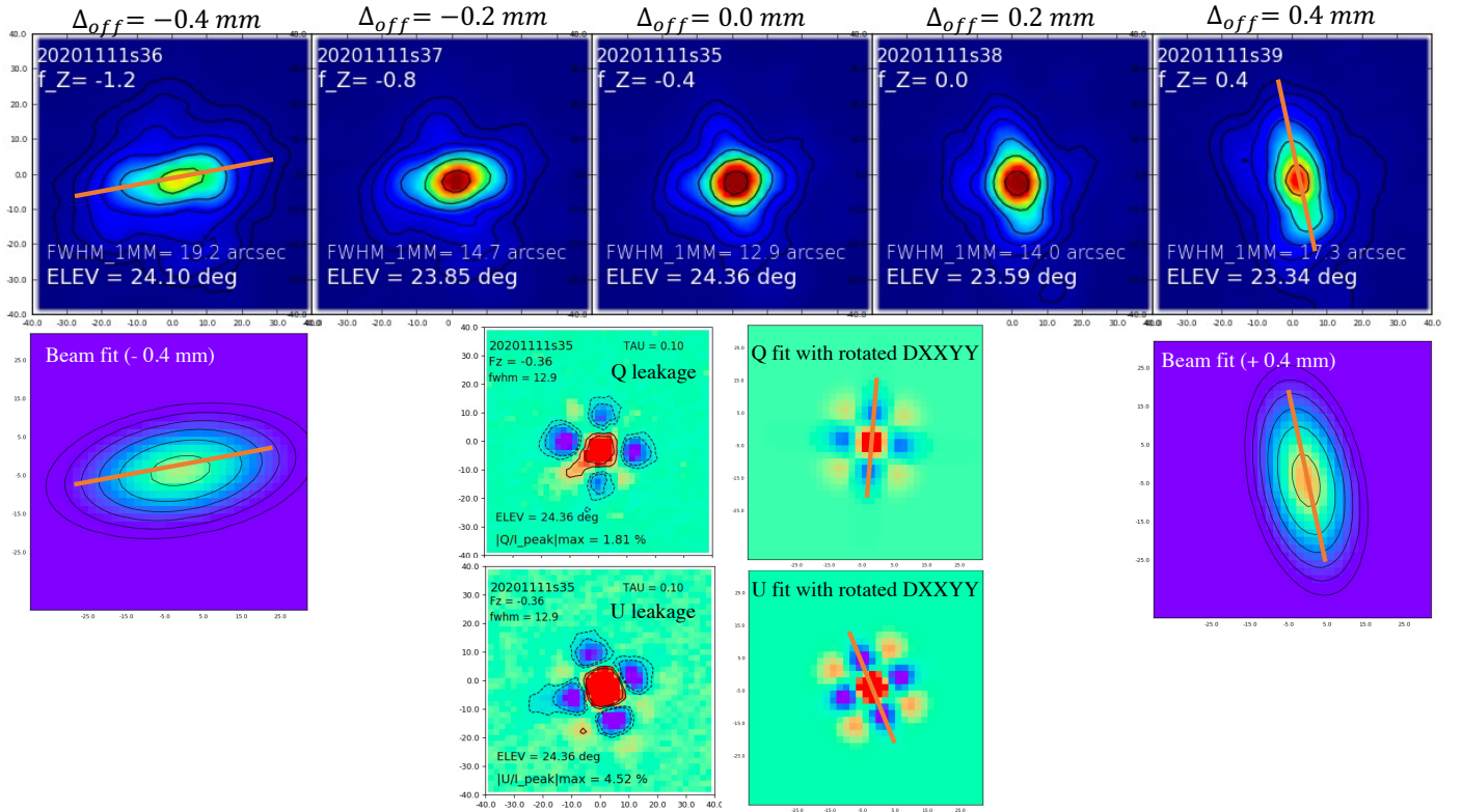
Figure 4.14: Top row : Examples of Stokes I images (in Nasmyth coordinates) obtained during a focus sequence on Uranus. The central image shows the beam observed at the best focus position ( \Delta_{off} = 0.0 ). Note how the beam (in I) becomes elongated along two orthogonal directions at the two extreme focus offset positions ( \Delta_{off} = \pm 0.4 mm). Bottom left and right panels : Elliptical Gaussian fits to the elongated beam shapes observed \Delta_{off} = \pm 0.4 mm, defining the orientation of the astigmatism effect. Central panels at the bottom : Cloverleaf leakage patterns observed in Q and U at the best focus position \Delta_{off} = 0.0 on the left, and simple fits to these cloverleaf patterns using a rotated version of the fourth-order derivative of a Gaussian beam \frac{\partial^4 B_I}{\partial x^2 \partial y^2} (cf. Fig. 4.11) on the right.
