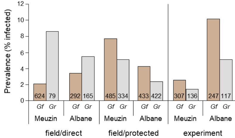
Figure 1 - Prevalence levels for Gammarus fossarum (Gf) and G. roeseli (Gr) in the two populations, for all experiments (field/direct: prevalence in natura; field/protected: prevalence in gammarids kept in the laboratory, i.e. protected from predation; experiment: experimental infection). Numbers in bars are sample size.
