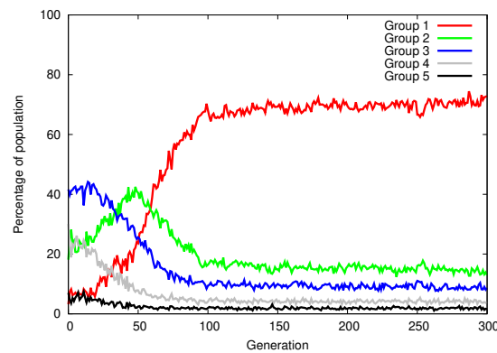
Figure 7.9: Classification using Lehmer code with adaptation
