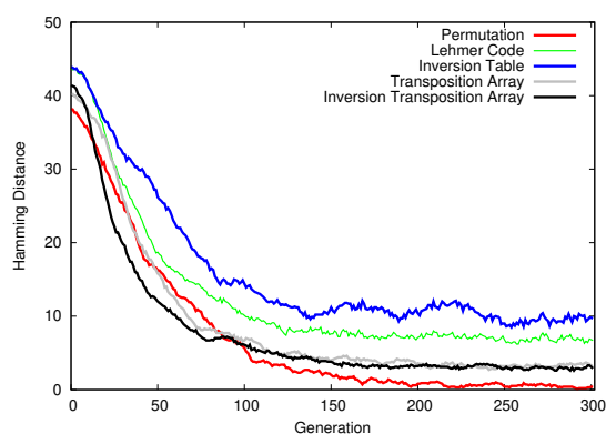
Figure 6.6: Hamming Distance for att48
