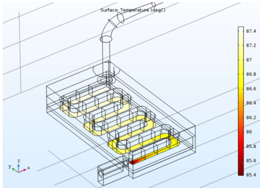
Figure S4.5. The simulated bottom surface temperature of the u-shape tunnel in the fouling rig.
