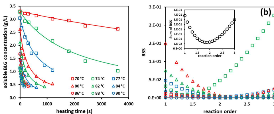
Figure 3.2. (a) Evolution of soluble BLG concentration against heating time at elevated heating temperatures (shown in legend) for a 0.5 wt% WPI solution containing 50 ppm \text{Ca}^{2+} . (b) Corresponding residual sum of squares (RSS) obtained at different heating temperatures fitted by equation 3.2. Inset shows the sum of RSS obtained using values from all heating temperatures at all calcium concentrations tested.
