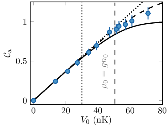
Figure 6.15: Corrected contrast C_a = n_1^c/n_0 induced by a periodic potential of period \lambda = 4 \mu\text{m} as a function of the potential depth V_0 (blue points). We obtain depletions larger than 1 for large potential depths because the contribution of higher harmonics on the density profiles are filtered out by the absorption imaging system. The solid black line is the result of Gross-Pitaevskii simulations without spatial filtering of the density profiles. As expected, the depletion saturates to one. The dashed black line is the result of Gross-Pitaevskii simulations where the density profile is filtered and we extract the contribution of the fundamental mode only, as for the experimental data. The dotted black line is the perturbative model Eq. (6.16) used to calibrate the potential V_0 and the correction factor r . This calibration was performed on potential values up to V_0 < 0.6 \mu_0 with the same mean density n_0 . The limit of the calibration regime is represented by the vertical grey dotted line. The grey vertical dashed line indicates the value of the chemical potential \mu_0 of the atoms without modulation and with the same mean density n_0 . Errorbars are standard deviations and horizontal errorbars are smaller than the point size. Data extracted from a preliminary analysis.
