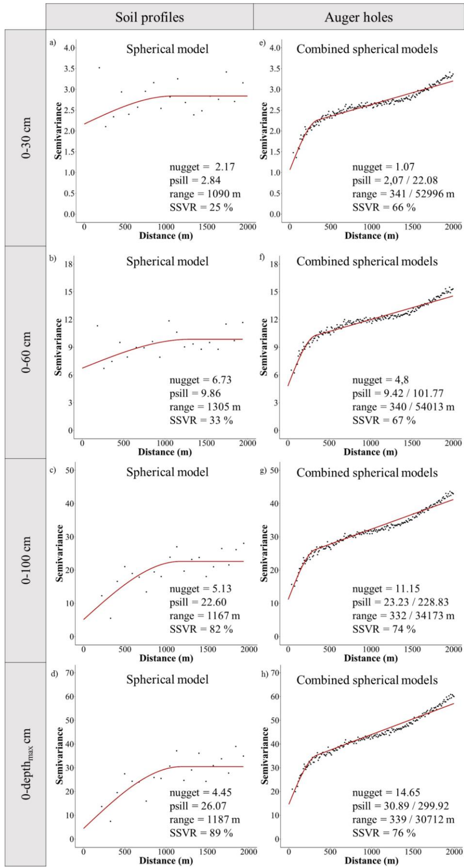
Figure 5.7. Empirical variograms computed for SAWC using 69 soil profiles at a) 30 cm, b) 60 cm , c) 100 cm and d) depth max , and, using 2781 auger hole observations at e) 30 cm , f) 60 cm , g) 100 cm and h) depth max , and their theoretical variograms.
