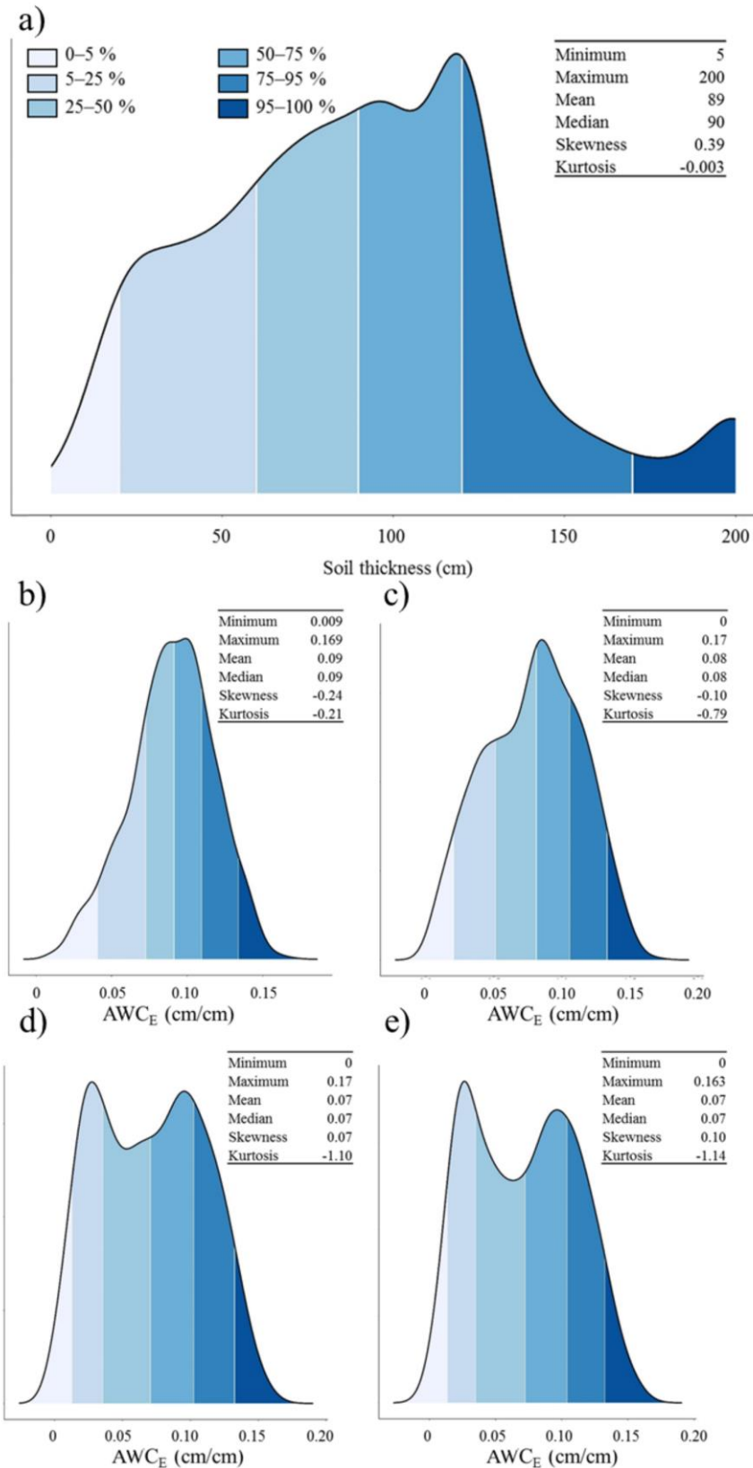
Figure 4.3. Distributions of the soil input variables; a) soil thickness, b) elementary available water capacity (AWC E ) of the 0-30 cm soil layer, c) elementary available water capacity of the 30-60 cm soil layer, d) elementary available water capacity of the 60-100 cm soil layer and e) elementary available water capacity of the 100-200 cm soil layer
