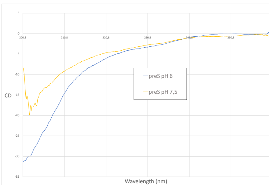
Figure 88. CD curves of preS in 20 mM PO 4 50 mM NaCl, 1X protease inhibitor (preS buffer) at two different pH.
