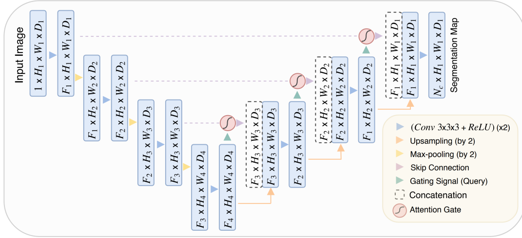
Figure 4.16: Architecture of attention U-Net. Attention gates filter the features propagated through the skip connections. Feature selection in the attention gates is achieved by the use of contextual information (gating) extracted in coarser scales. Credit: [131]
