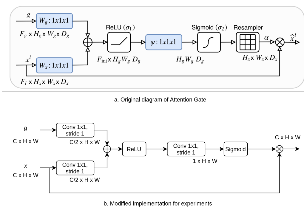
Figure 5.6: Diagrams of the original and the modified Attention Gate. The modified implementation removes the upsampling from Attention Gate as the gating signal and input features should have the dimension. Credit of diagram a: [131].
