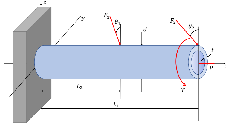
FIGURE 7.4: Illustration of the cantilever tube.
