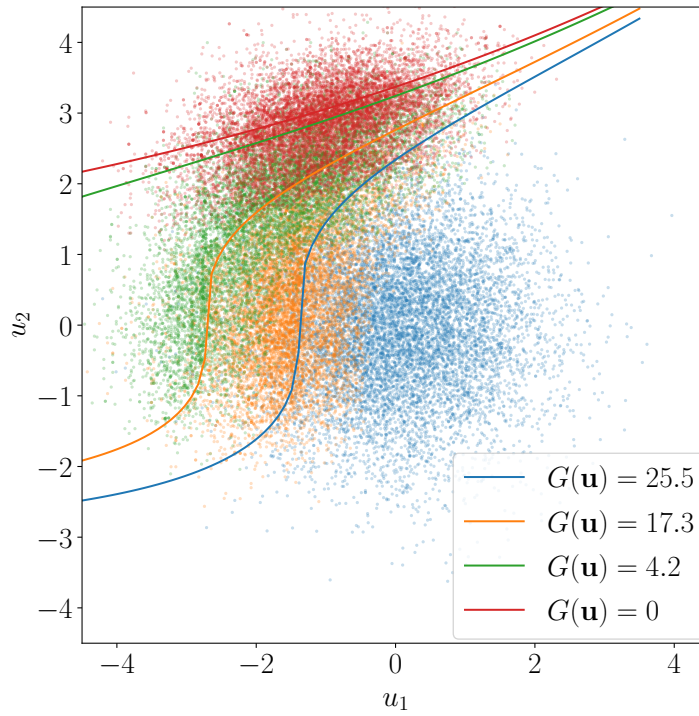
FIGURE 2.4: Graphical representation of the subset simulation procedure.
