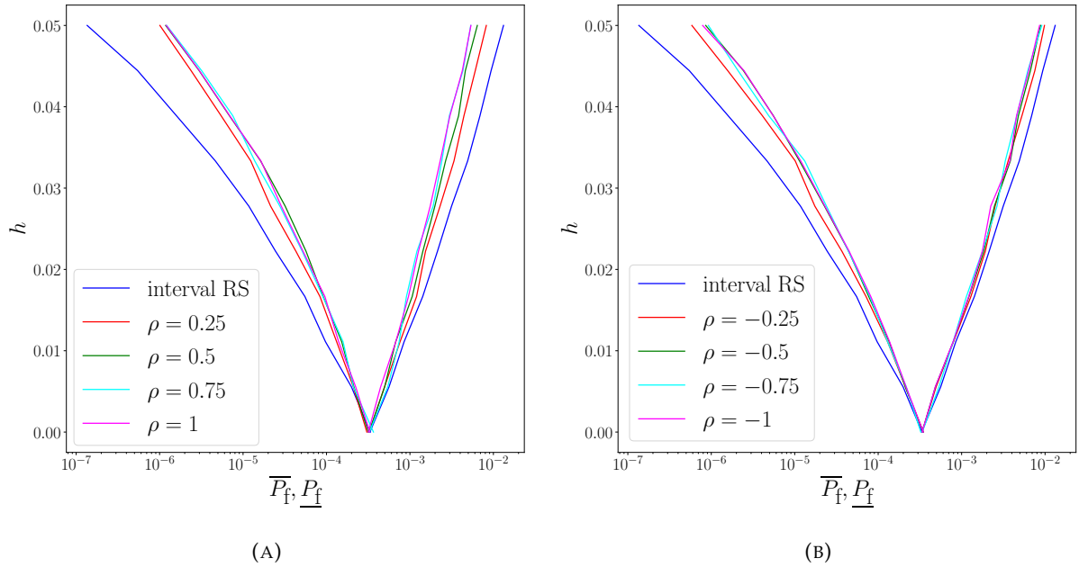
FIGURE 5.14: M_2 comparison for positive coefficients of correlation (A) and M_2 comparison for negative coefficients of correlation (B).
