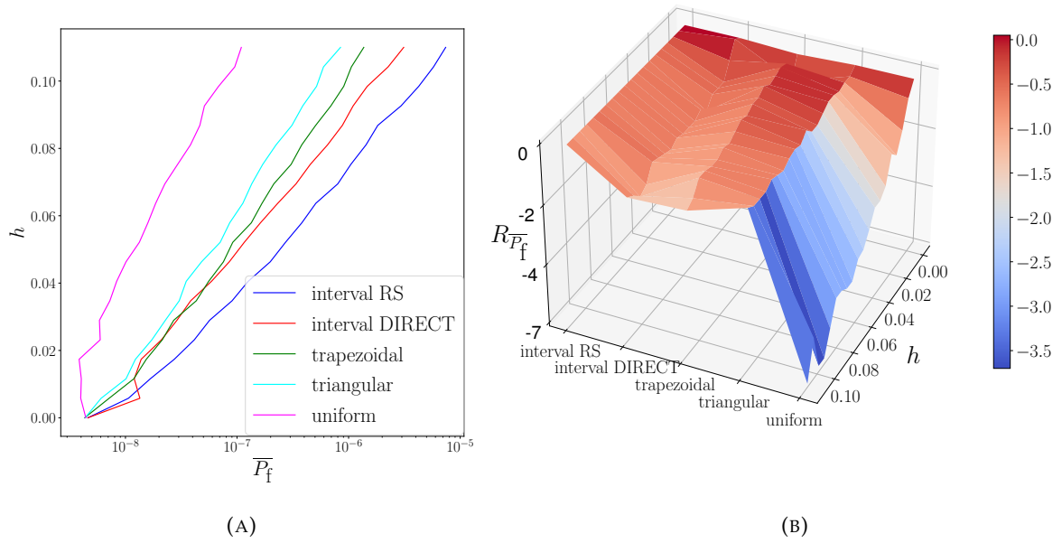
FIGURE 5.16: Robustness curves (A) and VoI metric (B) considering the M_1 group for the penstock use-case.
