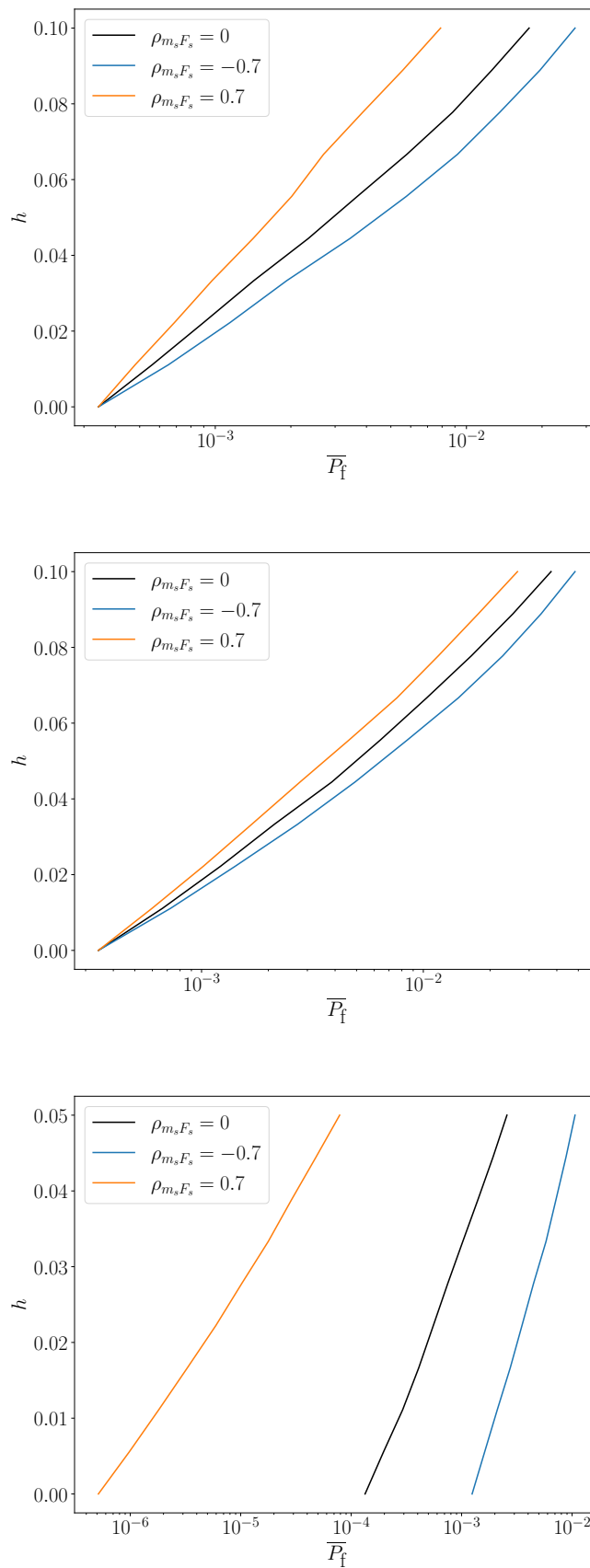
FIGURE C.2: Robustness curves considering dependency with a triangular distribution (top), a trapezoidal distribution (middle) and a p-box representation (bottom).
