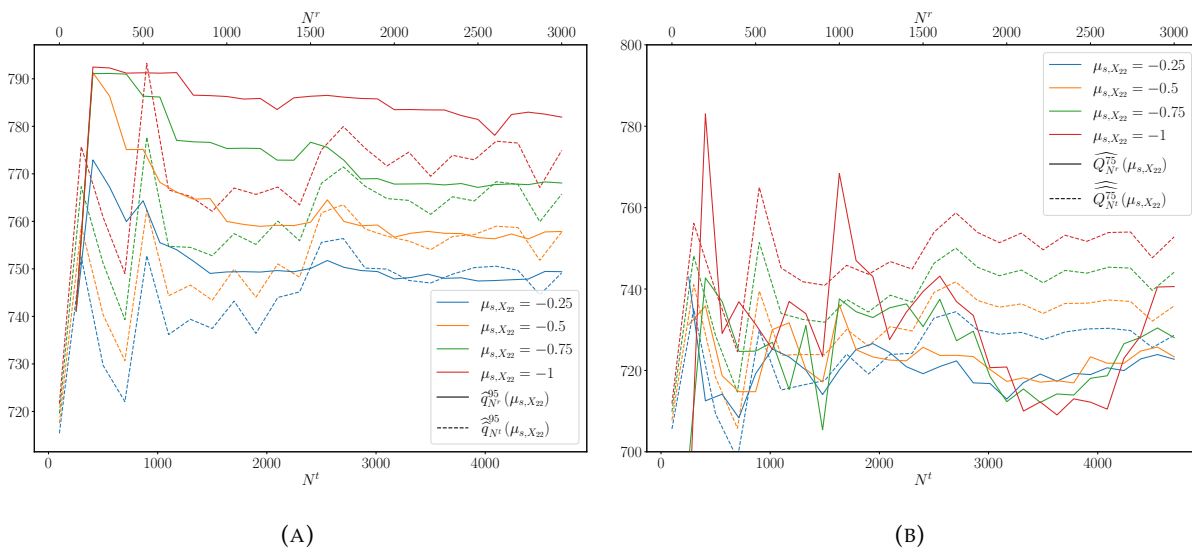
FIGURE 7.11: Convergence of the RIS estimator (solid lines) and the ANN estimator (dotted lines) on the quantile (A) and the superquantile (B) at four different values of \mu_s related to X_{22} .
