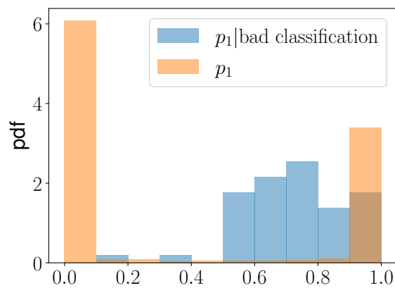
FIGURE 6.21: The pdf of the probability output p_1 of ANN 1 compared to its pdf conditioned to bad classifications for \theta^{(2)} .
