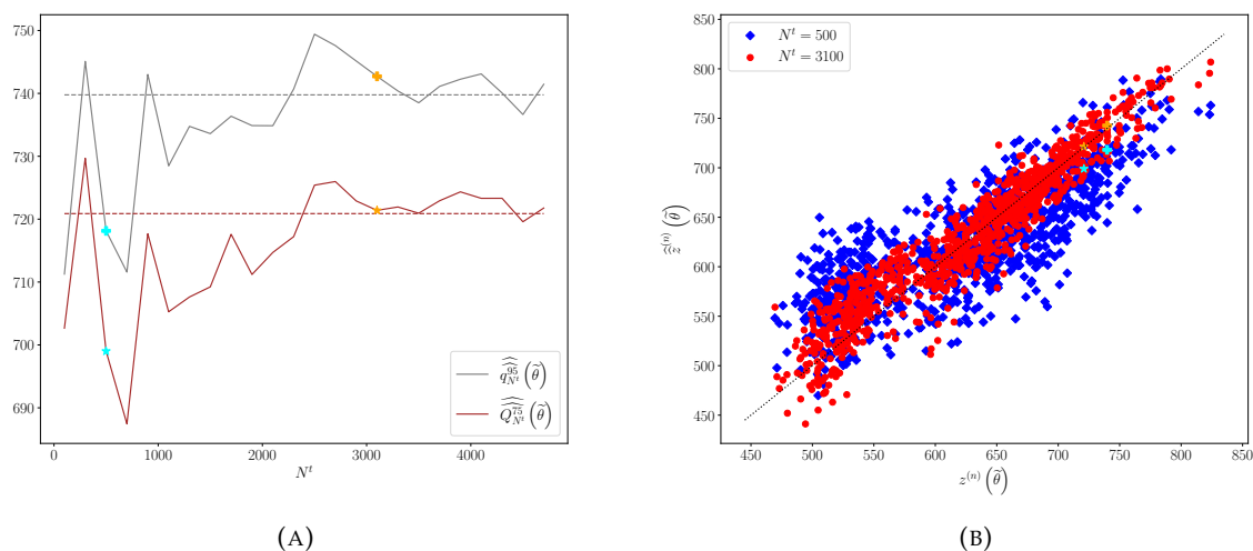
FIGURE 7.10: Convergence of the ANN estimator at the nominal configuration (A) and scatter plot obtained from the ANN on the 1000 MC samples.
