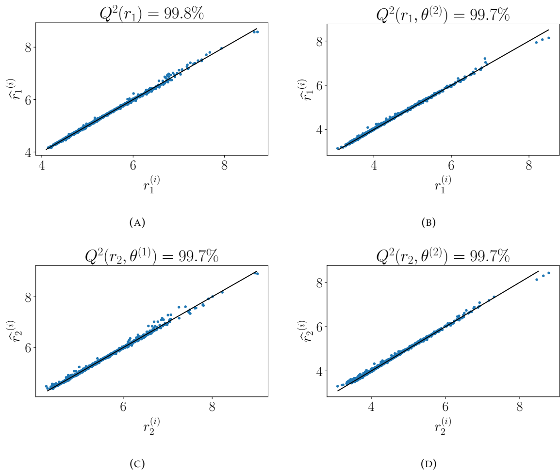
FIGURE 6.18: Comparison between the values of r_1^{(i)} and r_2^{(i)} from A_{E_3} and from the ANN at \theta^{(1)} (A,C) and \theta^{(2)} (B,D).
