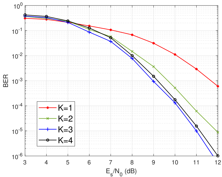
Figure 3.4 – BER of differential detection for the CPM scheme 3REC with h = 0.75 for different values of delay K
