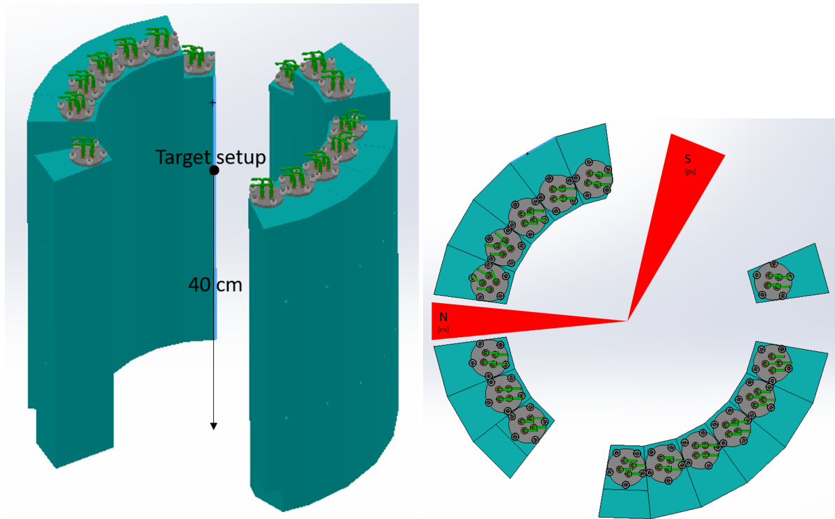
Figure 3.8: CAD representations of the neutron detector design used during the LULI2000 experiment. The right image is a top view while the left one is more from the side.
