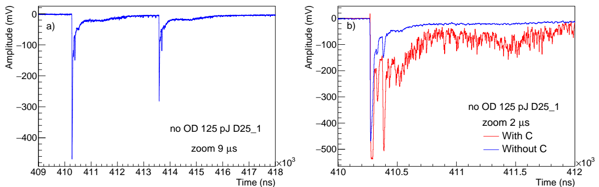
Figure 4.37: Zooms on a raw trace from the up PMT of detector unit 25 without the two last capacitances when receiving two 650 nm laser pulses with an energy of 125 pJ each with a 3.3 \mu s delay between them. a) shows a zoom on a 9 \mu s time window and b) shows a comparison between the cases with and without the capacitances on a 2 \mu s time window zoom.
