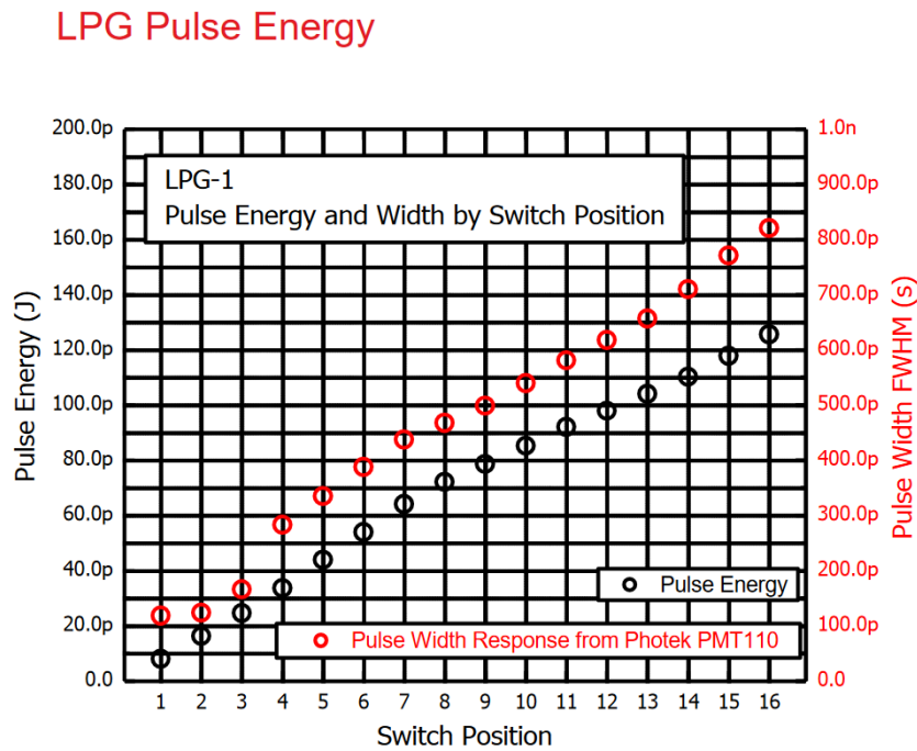
Figure 4.29: Width and energy of the pulses generated by the Photek LPG-650 laser according to the switch position.
