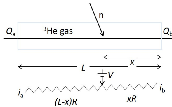
Figure 2.1: Representation of a ^3\text{He} gas proportional counter and sketch of its equivalent electronic circuit (120)
