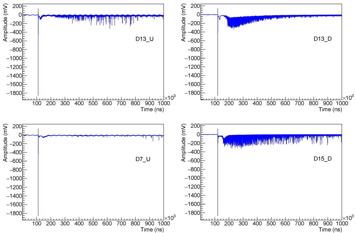
Figure 3.17: Examples of traces obtained from different detector units and PMTs during shot 28. During this shot, the proton energy cutoff was 16.31 MeV and a 1 \mu\text{m} solid vanadium target was in place.
