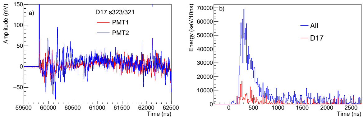
Figure 4.40: a) Signal obtained from detector unit 17 for shot 323 when subtracting the signal from shot 321 which is hence considered as a baseline. The primary target was a 2\ \mu\text{m} thick Al target for both shots and a 1 mm thick LiF neutron converter was additionally present during shot 323. b) Energy deposited in all the scintillators (blue) and in the scintillator of detector unit 17 (red) according to the time, according to Geant4 simulations using an isotropic neutron source with an energy spectrum calculated using a proton spectrum obtained at the LULI2000 facility and TALYS data considering a 1 mm thick LiF neutron converter.
