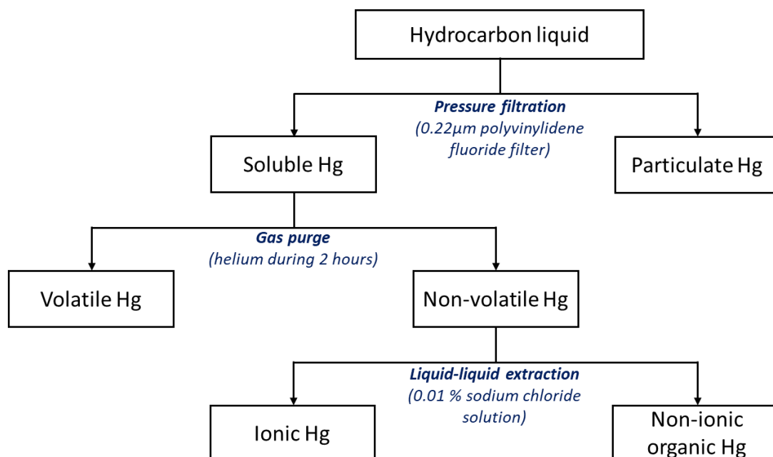
Figure 3. Diagram of mercury speciation analysis in liquid hydrocarbon by UOP Method 938-10 (adapted with permission from ref 5).
