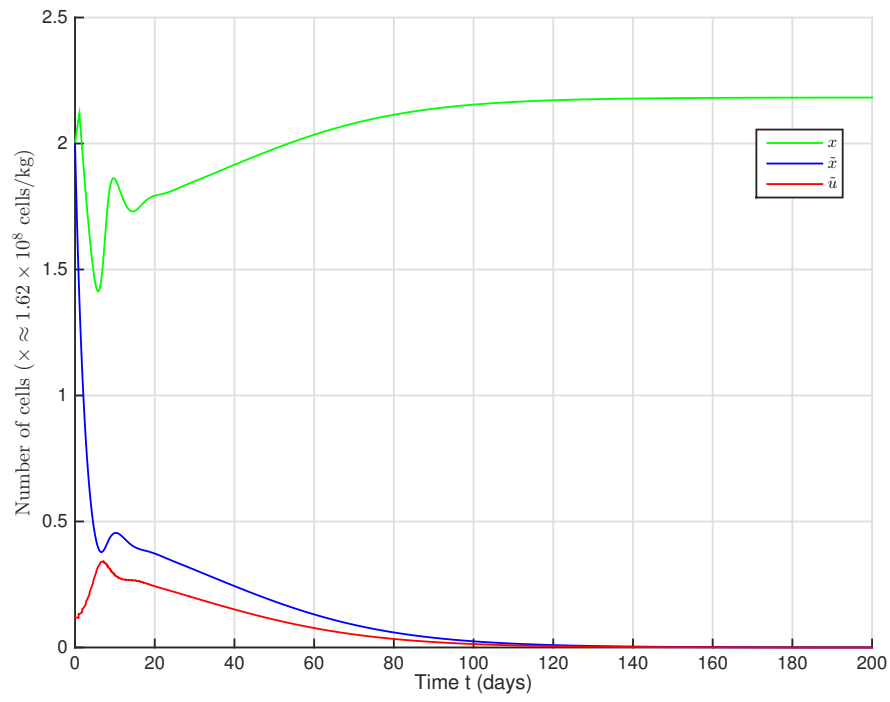
Fig. 6.7 Convergence to \mathfrak{E} .
