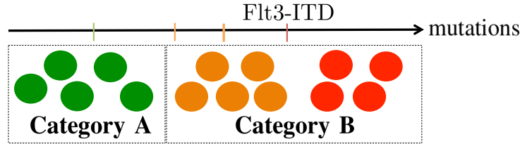
Fig. 6.1 Category A: healthy stem cells. Category B: unhealthy stem cells. The latter class (B) has a first mutation in some genes encoding enzymes in epigenetics (e.g. TET2, DNMT3A [74, 239]), that increases the self-renewing activity of the affected cells. A more serious pathological situation arises when a second mutation, affecting this time the pathways regulating the differentiation process such as NPM1 or transcription factors, appears on some of the cells. The superposition of these two events yields a blockade in differentiation (the subpopulation in orange color). Finally, a subsequent mutation impairing proliferation control (e.g. FLT3) appears in a subpopulation of cells that have already accumulated one or more of the previously mentioned mutations. The latter event activates an uncontrolled overproliferation of a subpopulation of cells, CSCs (in red), and thereby causes AML [137].
