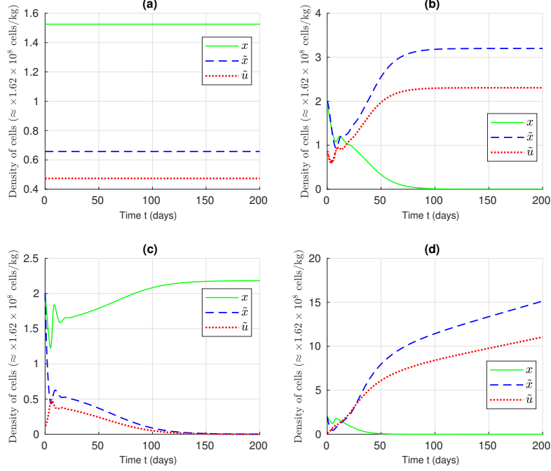
Figure 4: (a) Trajectories of the model whose parameters are given in Example 1, when they started on the Dormancy steady state \mathfrak{D} , where \bar{x}_e = 0.6573 , \bar{u}_e = 0.4737 and x_e = 1.5255 . We mention that in this case, numerical simulations show that \mathfrak{D} is unstable, i.e. for arbitrary small perturbation on the initial conditions, trajectories do not converge towards \mathfrak{D} . (b) Trajectories of the model whose parameters are given in Example 1, when they started from the initial conditions given by: \varphi_x(t) = \varphi_{\bar{x}}(t) = 2 , for all t \in [-\tau, 0] , and \varphi_{\bar{u}}(t) = 1 , for all t \in [-\bar{\tau}, 0] . The steady states \mathfrak{D} and \mathfrak{E} both exist in this case, however, we notice that the trajectories rather converge to another equilibrium point, that seems stable, and which is given by (3.1998, 2.3060, 0) . (c) All the model parameters and the initial conditions are similar to (b) , except the initial condition for \bar{u} which is now given by: \varphi_{\bar{u}}(t) = 0.1 , for all t \in [-\bar{\tau}, 0] . In this case, the trajectories converge to \mathfrak{E} = (0, 0, 2.1826) . (d) Now, we modify the value of \tilde{K} , that we increase to 0.6680, and we observe that for any initial conditions the trajectories \bar{x} \rightarrow +\infty and \bar{u} \rightarrow +\infty , when t goes to +\infty .
