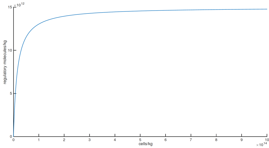
Fig. 4.7 The density of the regulatory molecules is limited, while the cell population continue to grow. Illustration of the function \psi_{a_0} , when a_0 = 15 \times 10^{12} .
