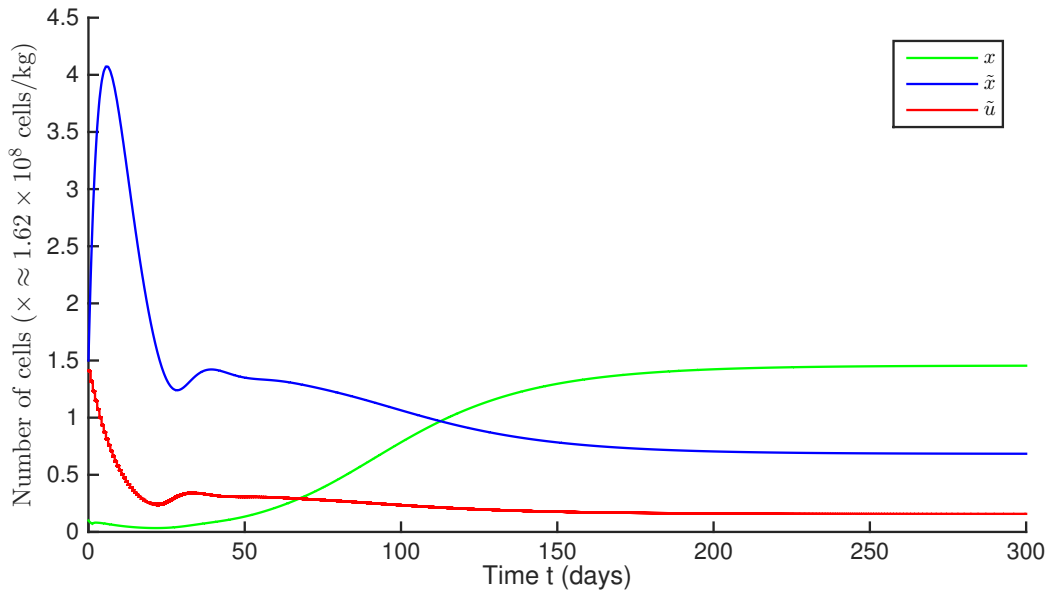
Fig. 6.11 Convergence to the dormancy steady state \mathfrak{D} .
