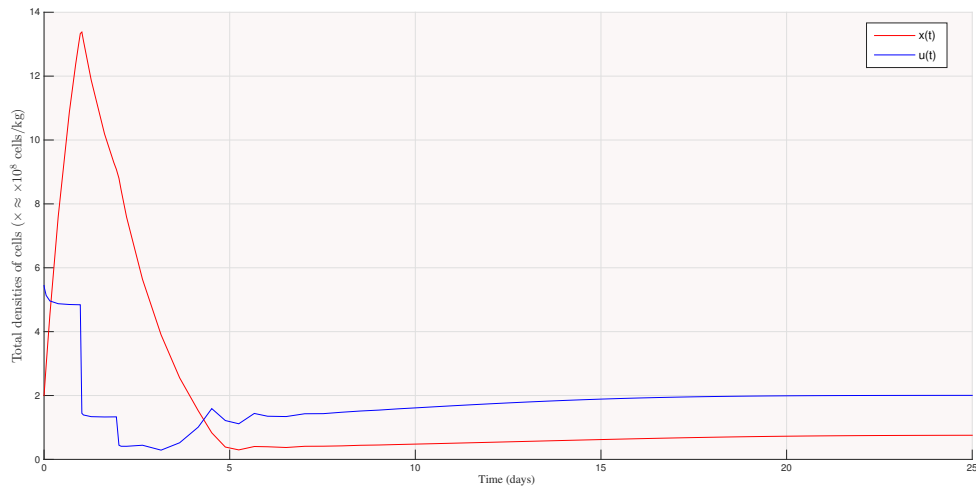
Fig. 5.10 The trajectories of the differential-difference nonlinear system (6.8), for the model paramaters given in Example 8.
