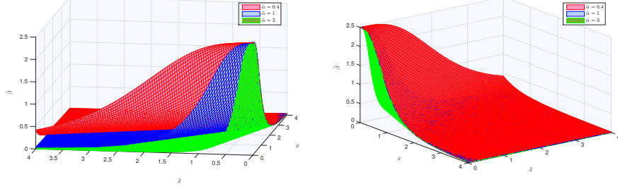
Figure 3: Illustrative example of variations of a typical \tilde{\beta} -surface with respect to \tilde{x} and x , for different values of \tilde{\alpha} (i.e. in the three possible situations: \tilde{\alpha} > 1 , \tilde{\alpha} = 1 , and \tilde{\alpha} < 1 ).
