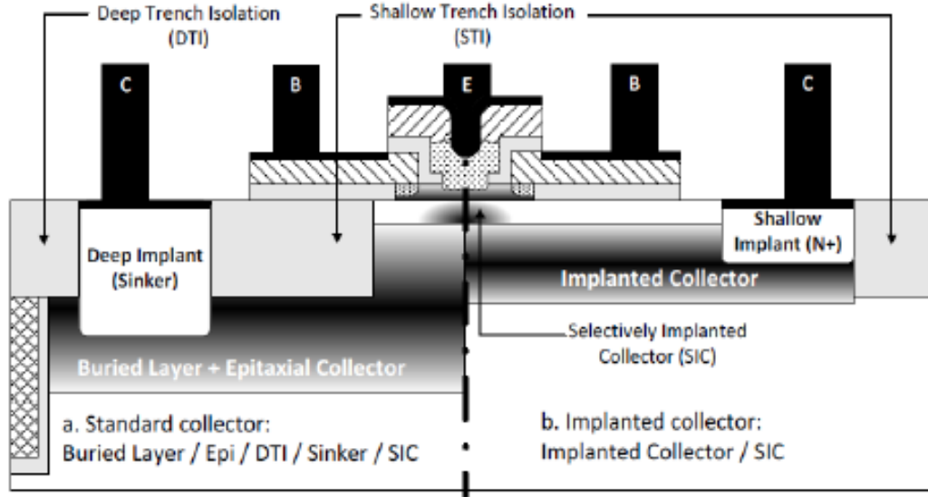
Figure I.14 | Comparison between DPSA-SEG HBTs featuring buried layer (left) or fully implanted (right) collector. Pictures from [8].
