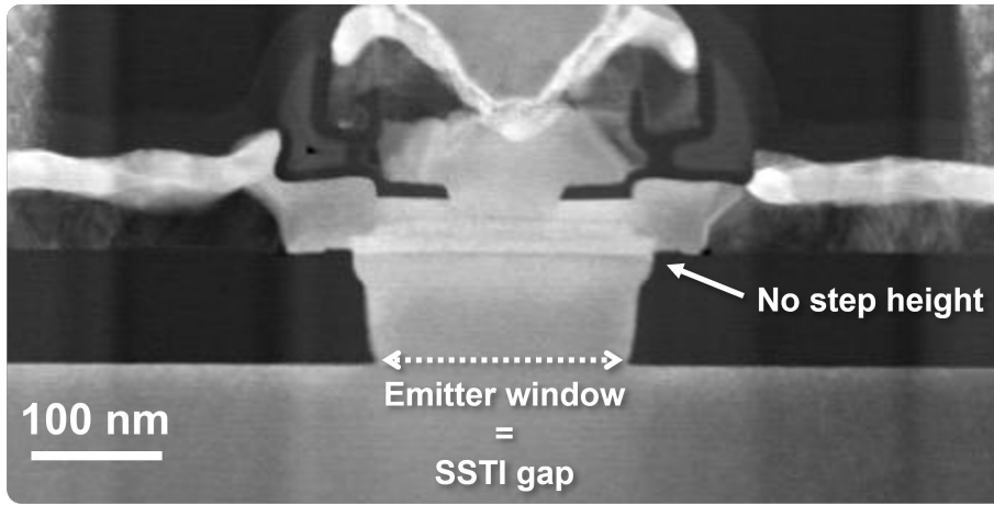
Figure II.12 | TEM cross-section detailing the improvements obtained with a single-shaped SSI.
