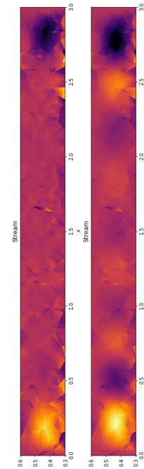
Figure 3.4: Corresponding stream function.
