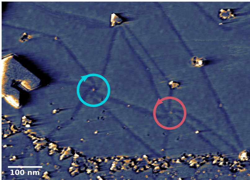
Figure 4.7: STM imaging ( V_b, I_t ) = (-300mV, 250pA) of a small lattice of domain walls featuring clockwise (cyan) and anticlockwise (magenta) rotating swirl relaxation patterns on intercalated bilayer graphene on SiC.
