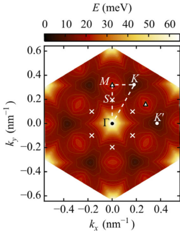
Figure 1.11: Colormap in the mBZ of the first conduction band for a 1.2^\circ TBLG. The K and K' points at the corners of the mBZ show local minima that correspond to the Dirac-like features originating from the folding of Dirac cone K_{\xi,1} and Dirac cone K_{\xi,2} , \xi = \pm 1 . Saddle points are indicated at the vHs energy at the S points. Adapted from [8].
