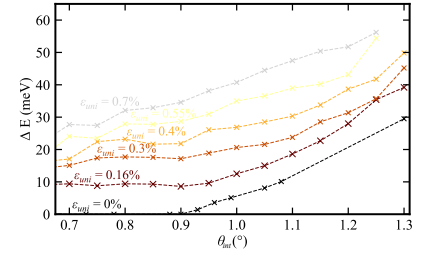
Figure 3.16: The spacing of van Hove singularities extracted from the DOS calculated using commensurate structures that include strain is plotted as a function of twist angle. Each color represents a different value of uniaxial strain, written on the left. In these calculations relying on the model presented in section 1.3.1, the magic angle is lower than 1.1^\circ .
