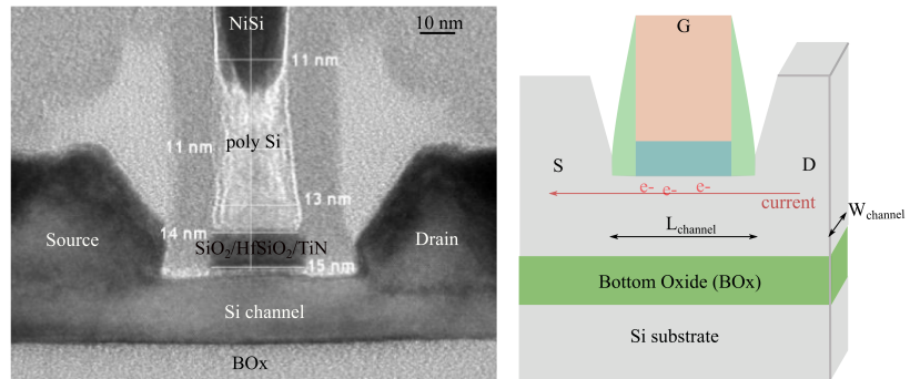
Figure 5.11: Left : TEM cut of a typical NMOS (n-doped MOSFET). Right : Sketch of a typical NMOS. The NMOS we measured had a channel length L = 0.1\mu\text{m} and width W = 0.06\mu\text{m} .
