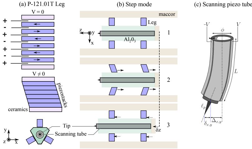
Figure 5.6: (a) Sketch of shear piezostacks as a function of voltage. (b) Sketch of the coarse motor in inertial mode. Z approach is achieved by applying an alternance of quick (2) and a slow (3) voltage ramps on the piezostacks.
