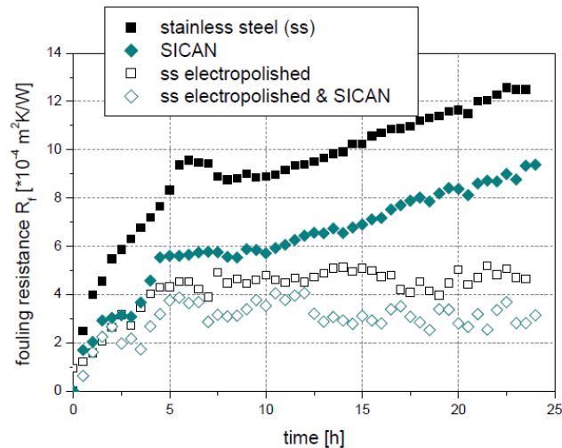
Figure 8. Impact of surface roughness and polar component on fouling resistance [92]
