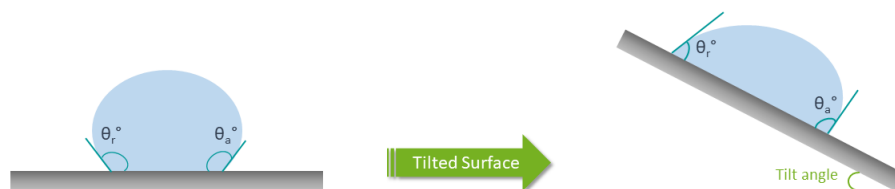
Figure 106. Diagram of the assessment of CAH by the tilting method.
