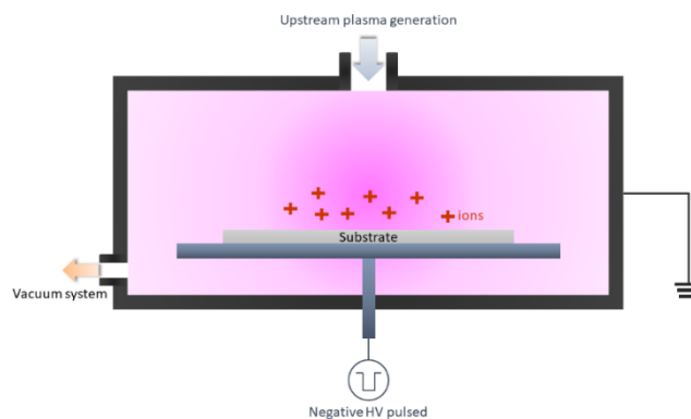
Figure 13. Schematic diagram of turbulent ion implantation process
