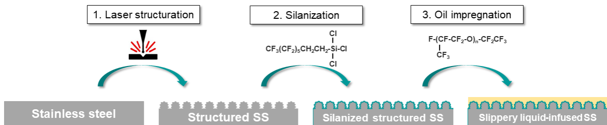
Figure 73. SLIPS-like surfaces process fabrication workflow.
