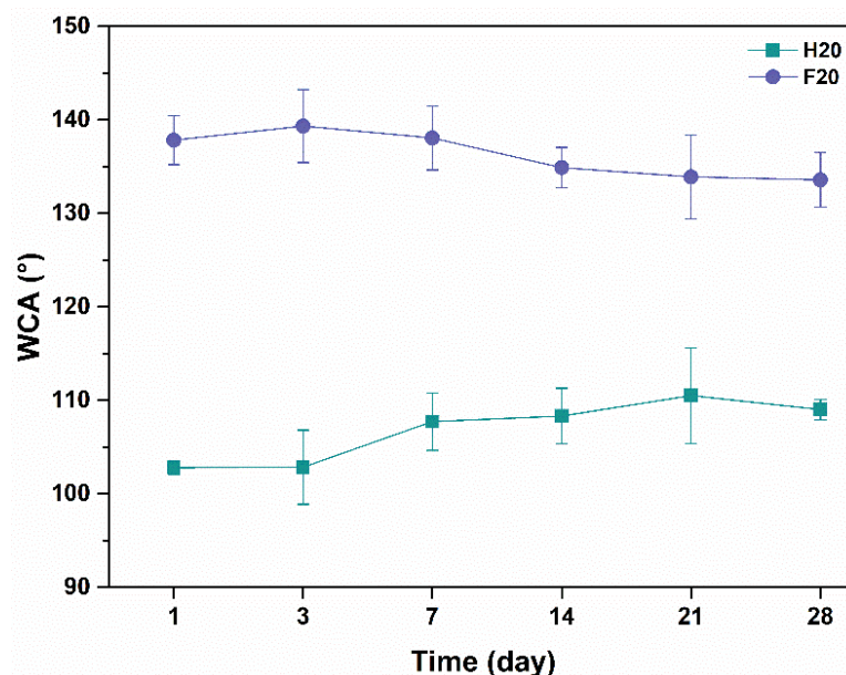
Figure 54. Assessment of plasma coatings ageing in air for 28 days.
