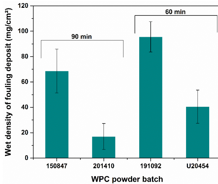
Figure 31. Comparison of WPC powder batches as the function of the density of fouling deposit
