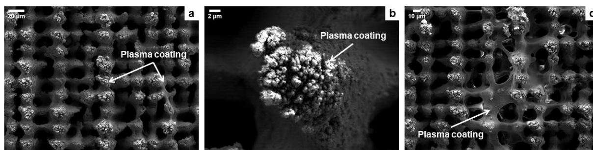
Figure 94. SEM images of the HMDSO layer onto structured stainless steel (a, b and c)
