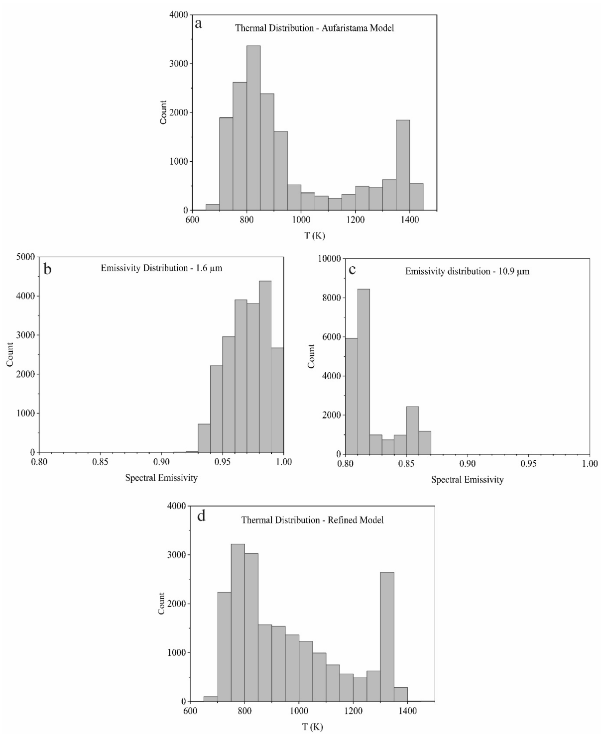
Figure 5-4: Results from AUFARISTAMA and the refined models. a) Temperature distribution of AUFARISTAMA model. b,c) Emissivity distribution for 1.6 μm SWIR and 10.9 μm TIR bands, respectively. d) Temperature distribution of the refined model from this study.
