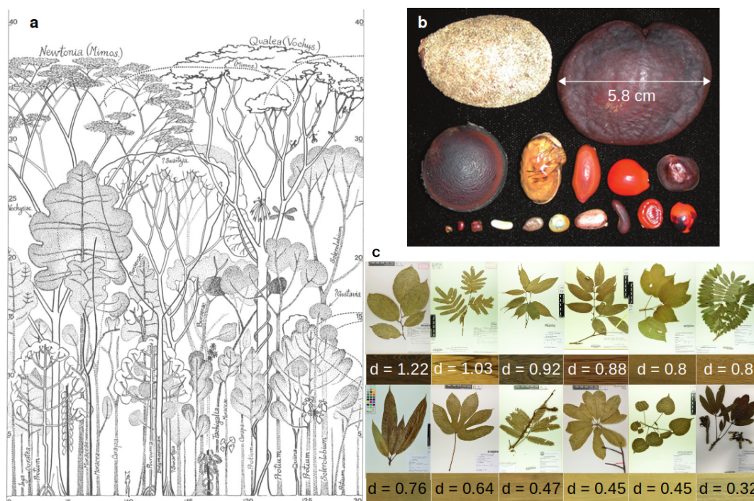
Figure 13: Morphological diversity of tree species illustrating strong differences between species. a. Diversity of tree species architecture and height in a tropical forest. Coordinates are in m. Copyright Hallé et al. (1978) . b. Diversity of seed size and shape from 17 tree species of the Fabaceae family in the Peruvian Amazon. Copyright Muller-Landau (2003) . c. Diversity of leaf size and shape (herbarium of Cayenne) and of wood aspect (reflecting wood characteristics) and density (CIRAD’s xylotheque) for 12 tree species in French Guiana. Species from top left to bottom right are Bocoa prouacensis , Zygia racemosa , Vouacapoua americana , Eperua falcata , Bagassa guianensis , Hymenolobium excelsum , Mangifera indica , Sterculia pruriens , Parkia nitida , Couroupita guianensis , Hura crepitans , and Ceiba pentandra . Black bars next to herbarium samples indicate the scale (10 cm). Copyrights Gonzalez et al. (2021) and Normand et al. (2017) .
