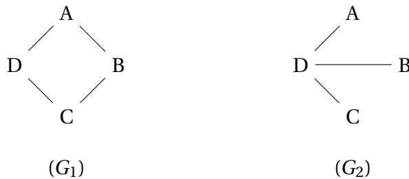
Figure 1.1: A traceable (resp. non-traceable) graph G_1 (resp. G_2 ).
