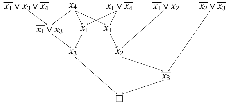
Figure 6.5: Adapting a resolution refutation to a tree-like resolution refutation
