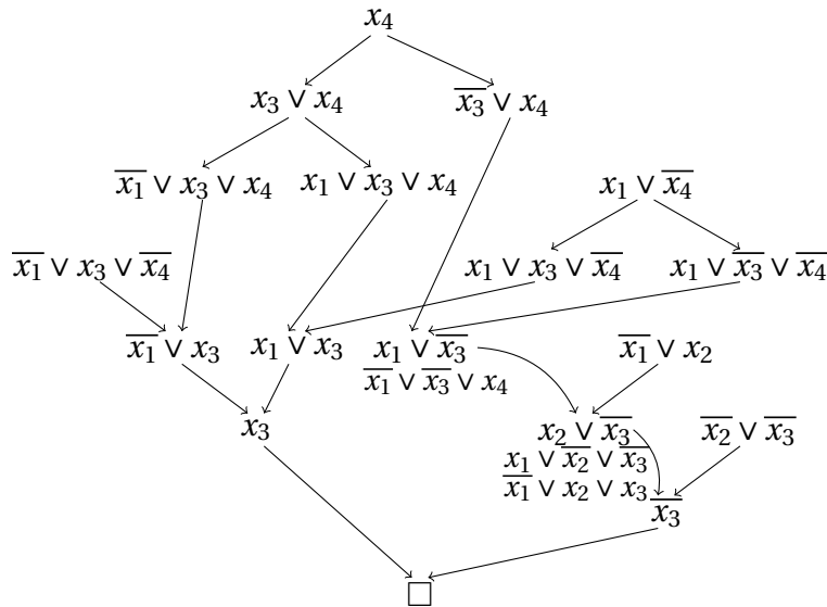
Figure 6.6: Adapting an unrestricted resolution refutation to a max-refutation
