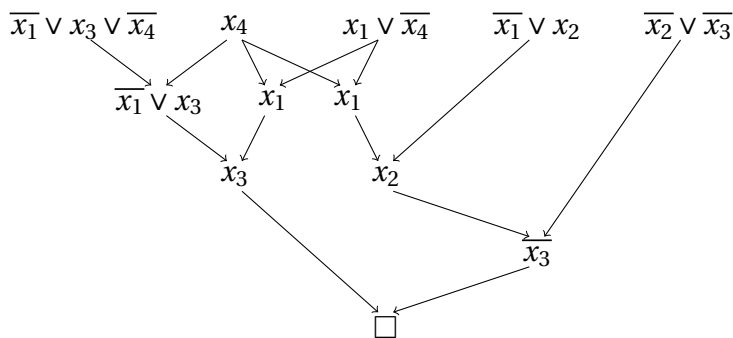
Figure 6.5: Adapting a resolution refutation to a tree-like resolution refutation
