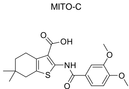
2-[(3,4-Dimethoxybenzoyl)amino]-6,6-dimethyl-5,7-dihydro-4H-benzothiophene-3-carboxylic acid
