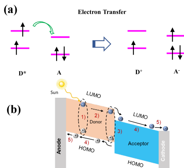
Figure 2.12 (a) Electron transfer from an excited donor molecule ( D^* ) to a neutral acceptor (A). The asterisk denotes excited state. The arrows represent simultaneous rearrangement of the electronic configuration. (b) Energy level diagram of donor and acceptor materials in an organic solar cell: the five steps of photovoltaic effect are represented by numbers and detailed above.
