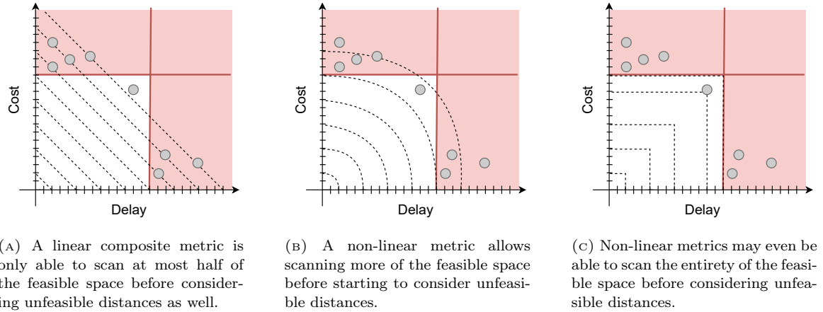
FIGURE 3.8: Figures illustrating how non-linear distance allow to search the feasible space.
