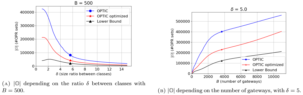
FIGURE 5.5: Evolution of |O| depending on various factors.
