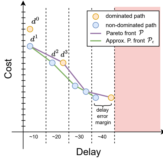
FIGURE 3.9: Reducing the precision of the delay only (while remaining exact on the cost) still allows to bound the number of non-dominated paths
