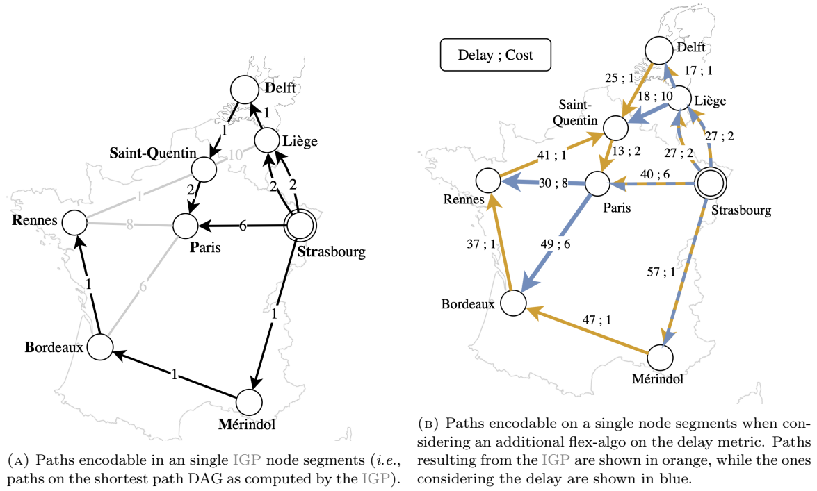
FIGURE 2.13: Comparison of path encodable in a single segment with and without the use of a custom flex-algo.
