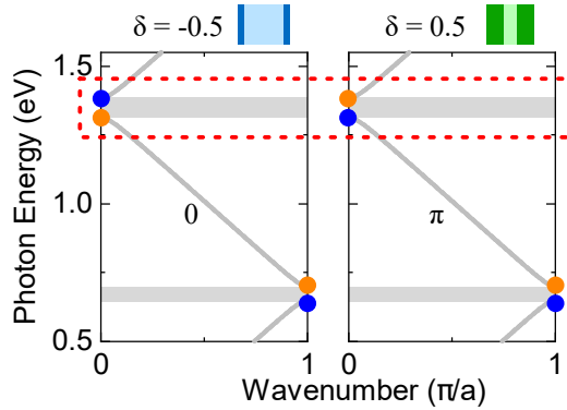
Figure 3.15: Optical dispersion relation of two superlattices with \delta = -0.5 and \delta = 0.5 . The schematic of the unit cells of each superlattice is represented in insets. The two dispersion relations present inverted Bloch mode symmetries around the bandgap at the Brillouin zone center. The dashed red box indicates the bandgap over which the band inversion takes place. The mode symmetries are indicated with orange (symmetric) and blue (anti-symmetric) dots. The Zak phase of the second band is indicated.
