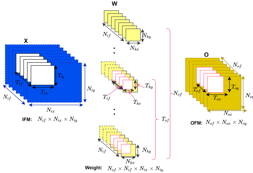
Figure 8.6: Convolution layer with loop tiling of the input, output and weight 'pixels' or 'feature maps'.
