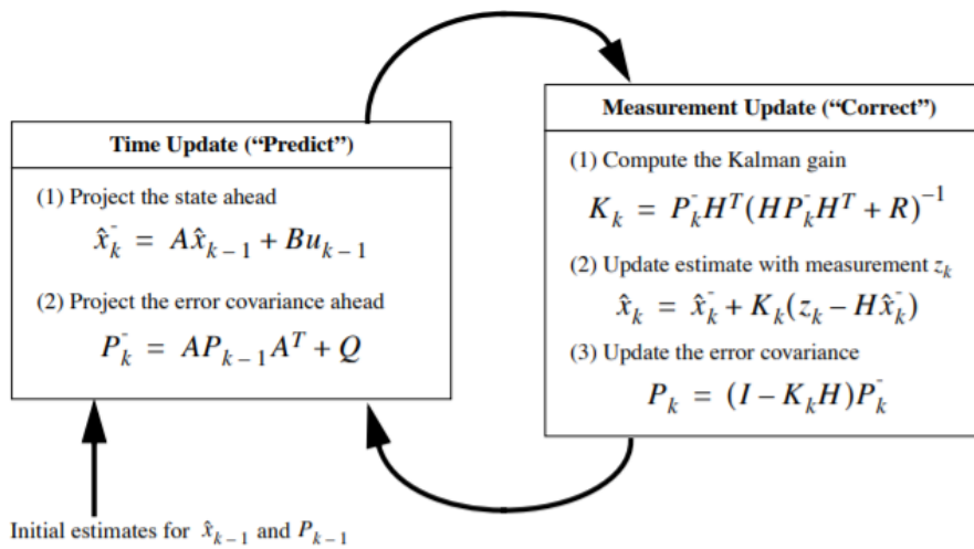
Figure 3.12: A complete picture of the operation of the Kalman filter illustrated mathematically
