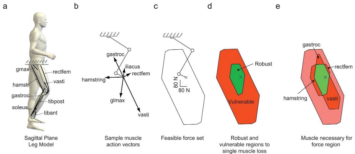
Figure 18: Illustration of the mechanical constraints that can limit the muscle redundancy. A represents the model considered with 14 muscles groups (only 8 are represented for a clarity purpose). B represents the force vector of each muscle group. C represents the feasible force set generated by these vectors. D displays the regions that are robust or vulnerable to the loss of any muscle. E displays the regions vulnerable to the loss of only one muscle. Gastric, gastrocnemii ; gmax, gluteus maximus ; rectfem, rectus femoris ; tibant, tibialis anterior ; tibpost, tibialis posterior ; vasti, vastii . From Kutch & Valero-Cuevas (2011).
