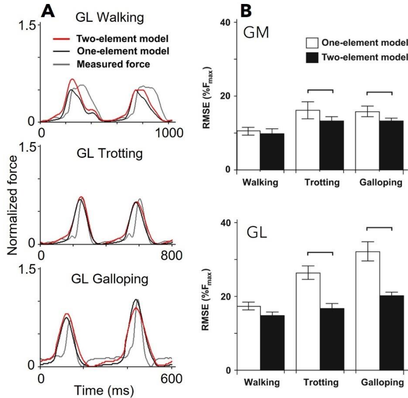
Figure 15: Comparison of predicted force from a Hill-type model to measured force using buckle-type force transducer in goat. A represents the force profiles of the gastrocnemius lateralis (GL) measured using buckle-type force transducer (grey), estimated from a conventional Hill-type model (one-element model; black) or estimated from a Hill-type model that accounts for slow and fast motor units (two-element model; red). B represents the root mean square error (RMSE) between the measured force and the estimated force from the Hill-type models for the gastrocnemius medialis (GM) and GL. From Lee and al. (2013).
