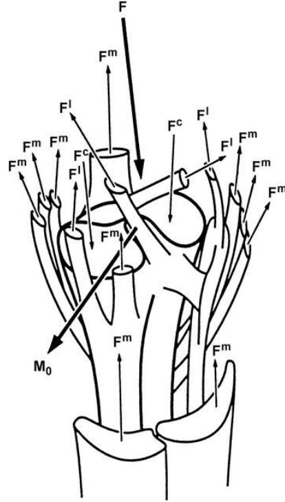
Figure 17: Illustration of the different forces acting on the human knee. Muscle force ( F^m ), ligament force ( F^l ) and bony contact force ( F^c ) influence the joint moment ( M_0 ). From Herzog et al. (2017) based on Crowninshield and Brand (1981a).
