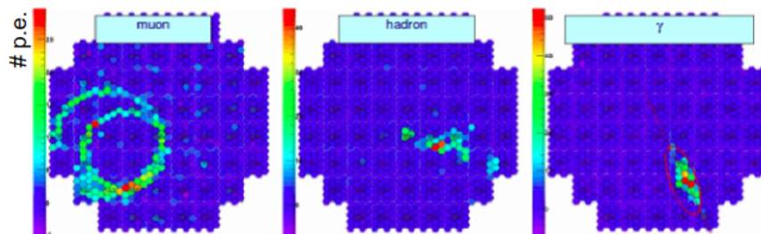
Figure 2.4: Images of atmospheric showers in the camera. From left to right, showers induced by a muon, a hadron and a photon are shown, respectively.
