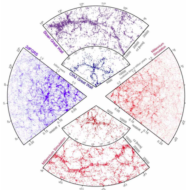
Figure 3.4: The left panel shows the map of a part of the 2dF Galaxy Redshift Survey. The top one shows a part of the Sloan Digital Sky Survey. Maps obtained for the corresponding portions of the sky with the Millennium simulations are shown in the right and bottom panels. Figure extracted from Ref. [340].
