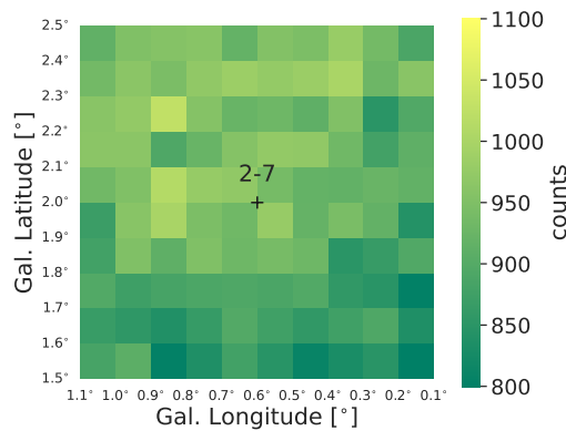
Figure 6.10: Map of the measured events from background for the squared region of side 1^\circ side and with squared pixels of 0.1^\circ \times 0.1^\circ taken around the IGS pointing position 2-7.
