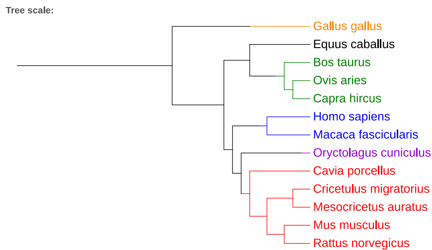
Figure 11 Species tree generated with PhyloT. Representation in ITOL IgG/Fc R tree. Fasta sequences aligned using ClustalW with standard settings for slow/accurate alignment of Protein sequences. Species trees were generated using the PhyML Bootstrap method.
