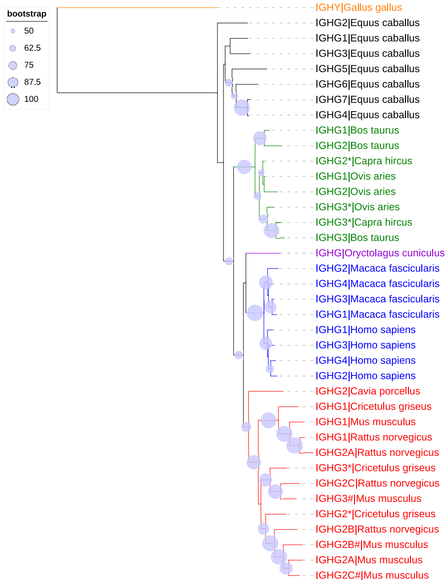
Figure 12 Phylogenetic analyses of selected mammalian IgG and chicken IgY. Protein sequences were aligned using ClustalW with standard settings for slow/accurate alignment of Protein sequences. Trees were generated using the PhyML Bootstrap method. Alignments were done on the whole constant region sequence, including CH1, hinge, CH2, CH3 (and CH4 for Gallus). * Indicates hypothetical/predicted protein, # indicates truncated sequences after CH3 domain.
