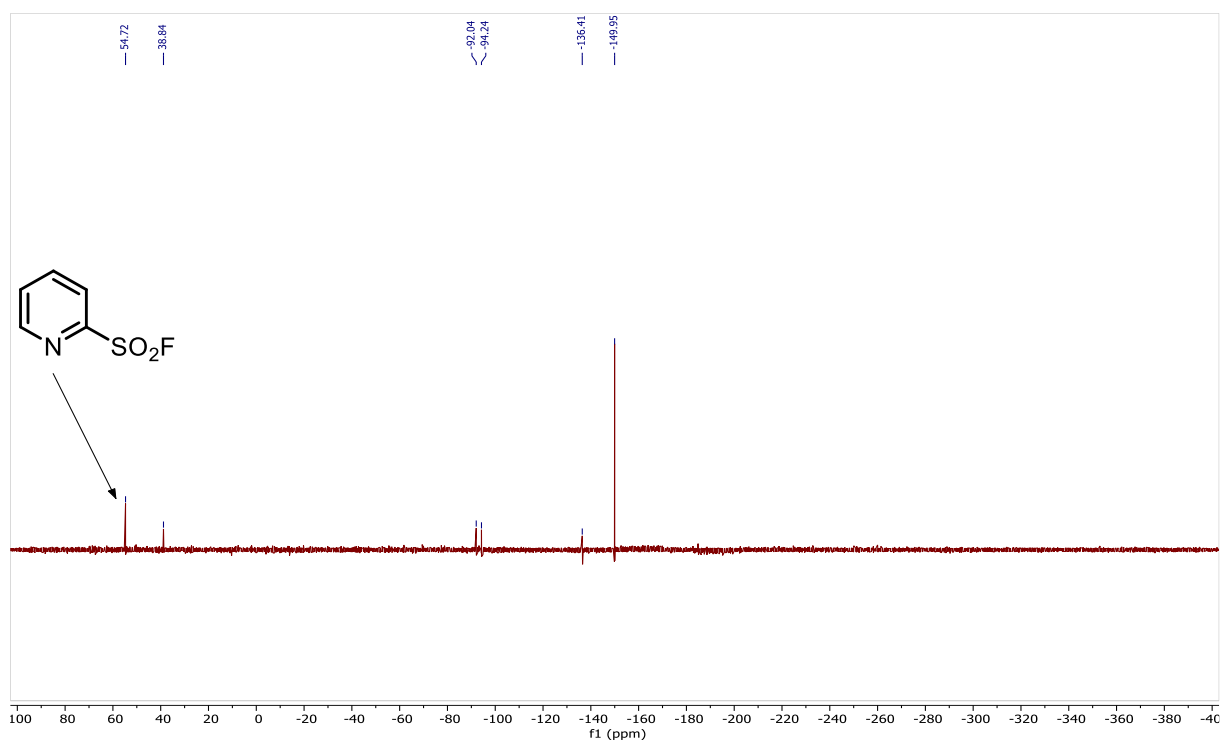
^{19}\text{F} NMR spectrum of reaction B after 2 h.
