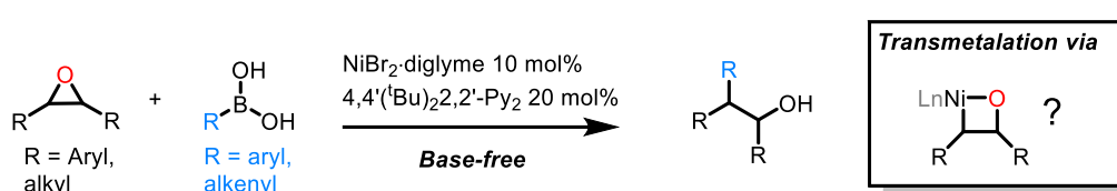
Figure I.19: Base-free Suzuki coupling of epoxides – undisclosed mechanism
