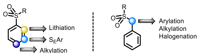
Figure I.56: Sulfones as a synthetic handle for various transformations
