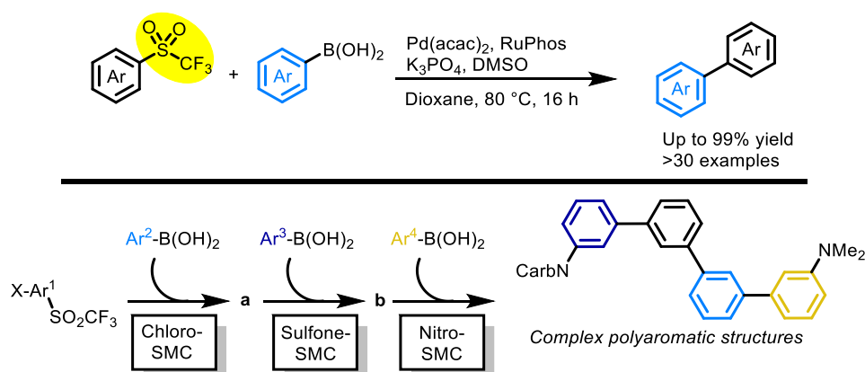
Figure I.59: Our work on the coupling of aryl sulfones
