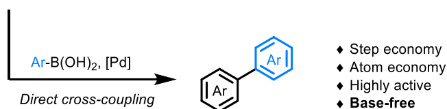
Figure I.35: Coupling of halides vs direct coupling of diazoniums
