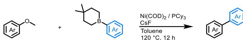
Figure I.45: Nickel-catalyzed Suzuki cross-coupling on methyl ethers
