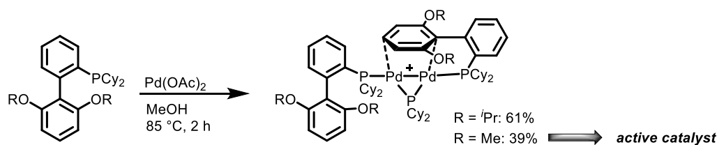
Figure I.28: Bedford's work on the facile formation of unusual complexes from Buchwald ligands and Pd(OAc) 2
