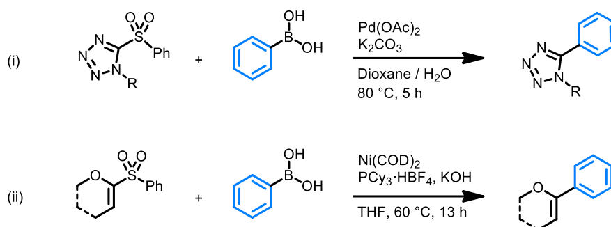
Figure I.58: Coupling of tetrazolic and \alpha -oxo vinyl sulfones
