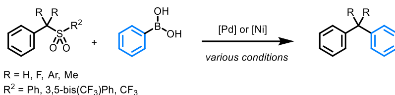
Figure I.57: Crudden's work on benzylic sulfones
