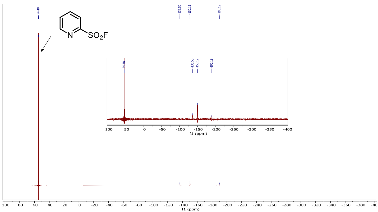
^{19}\text{F} NMR spectrum of reaction A after 8 h.
