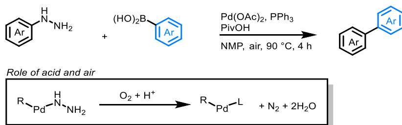
Figure I.48: Suzuki coupling requiring acid and oxygen: aryl hydrazines
