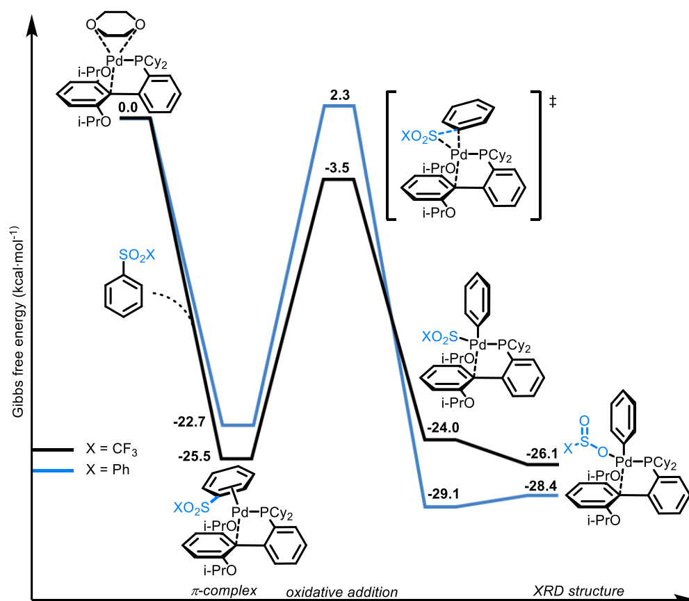
Figure II.4: Calculated Gibbs energies for the oxidative addition of sulfones to monoligated Pd 0 (RuPhos)
