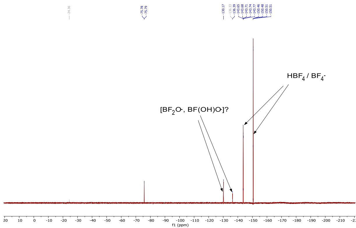
^{19}\text{F} NMR of the \text{D}_2\text{O} phase
