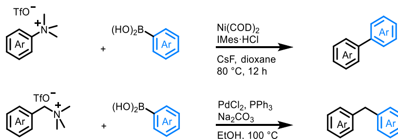
Figure I.47: Suzuki coupling of aryl and benzylic trimethyl ammoniums
