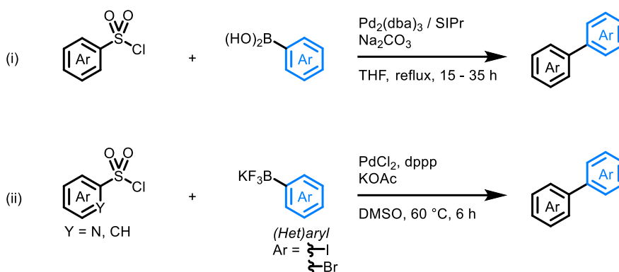
Figure I.53: The Suzuki coupling of sulfonyl chlorides: orthogonality to iodides and bromides
