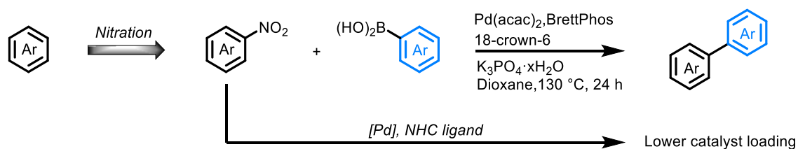
Figure I.49: The Suzuki coupling of nitroarenes
