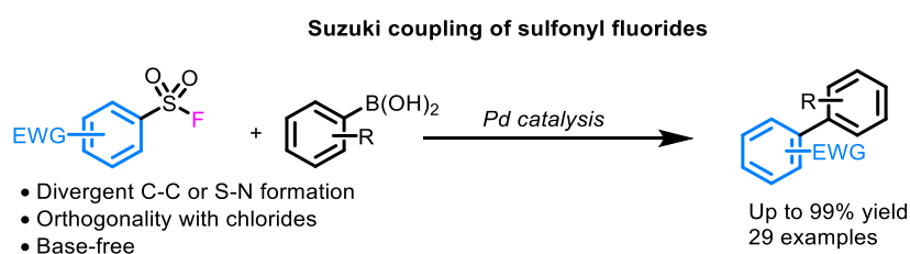
Figure IV.4: Summary of the coupling of sulfonyl fluorides
