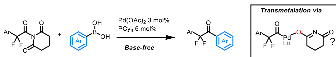
Figure I.20: Base-free Suzuki coupling of fluoroacetamides
