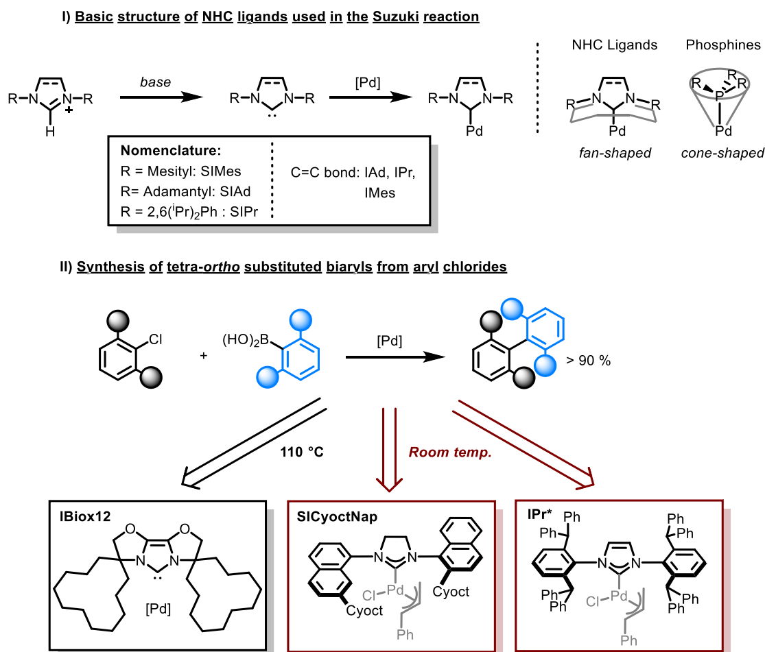
Figure I.31: Basic structure of NHC ligands and examples of challenging reactions
