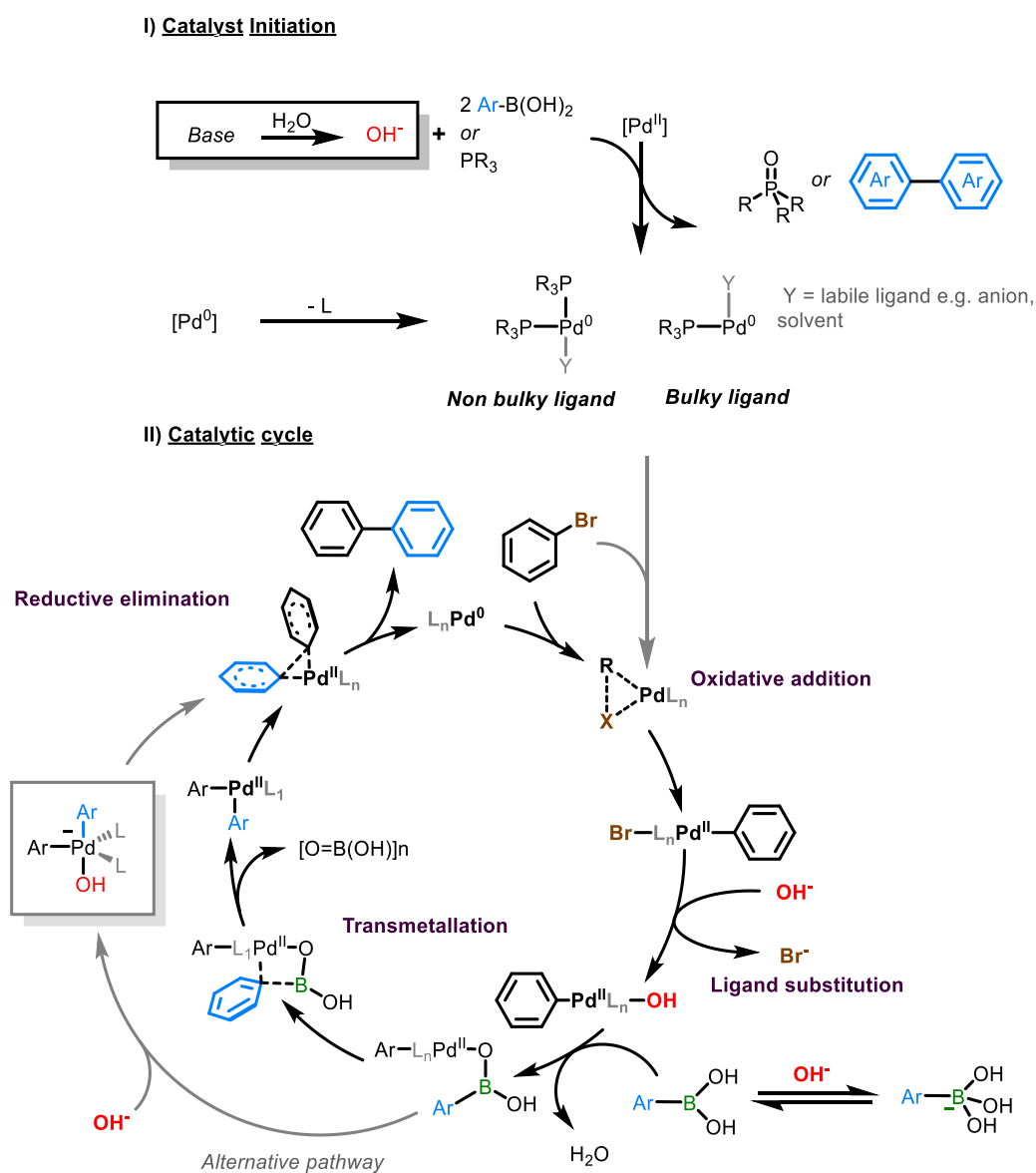
Figure I.23: A more accurate representation of the Suzuki cross-coupling mechanism summarizing the previous discussion. The hydroxide ion can be substituted for a fluoride ion.
