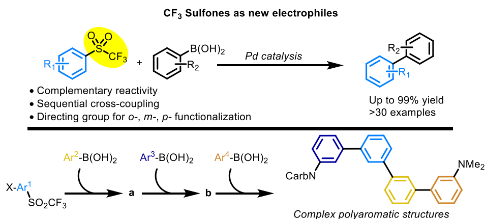
Figure IV.2: Summary of the work on the coupling of sulfones
