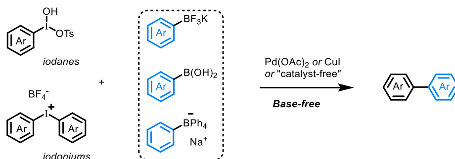
Figure I.17: Base-free cross-coupling of diazoniums and hypervalent iodine (III) compounds – transmetalation via cationic complex
