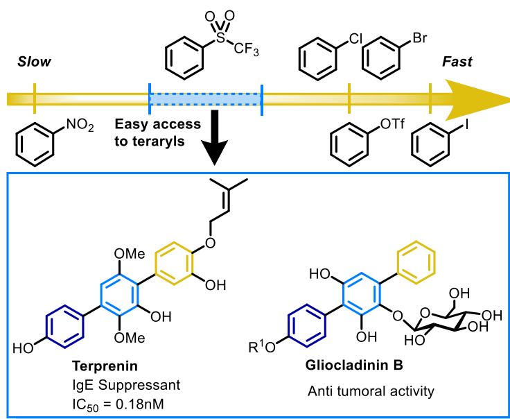
Figure II.9: Order of reactivity of aryl sulfones in the Suzuki reaction, facilitating access to terphenyls
