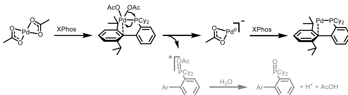
Figure I.29: Mechanism of reduction of Pd(OAc) 2 through oxidation of Buchwald ligand XPhos
