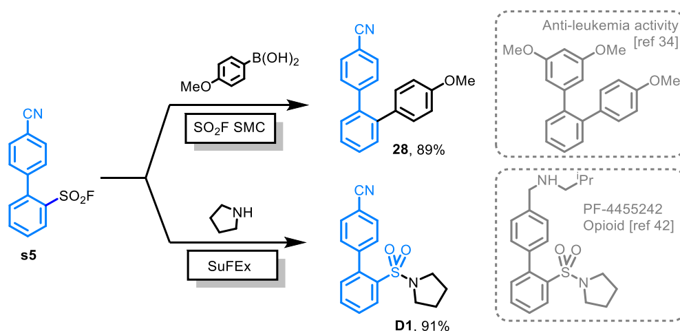
Figure IV.3: Divergent synthesis from sulfonyl fluorides, highlighting the usefulness of the present method
