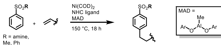
Figure II.6: Aryl sulfones are a robust directing group for all three positions of an arene
