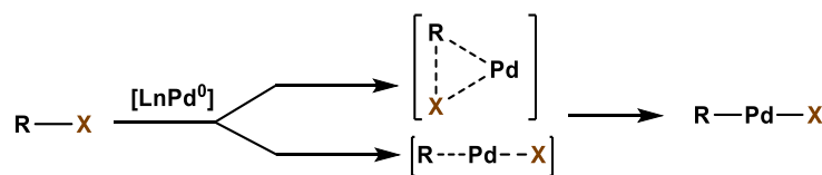
Figure I.5: Concerted pathway for oxidative addition
