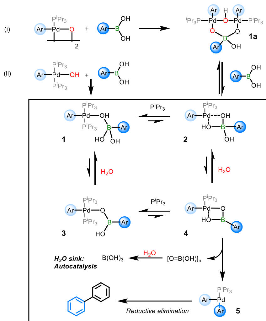
Figure I.15: Denmark's elucidated transmetalation mechanism
