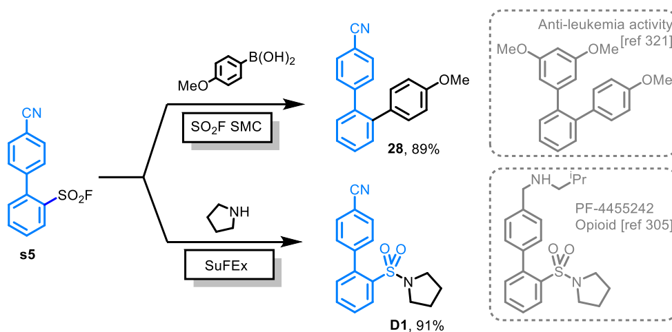
Figure III.6: Divergent synthesis from sulfonyl fluorides illustrating the complementarity between SuFEx chemistry and the Suzuki coupling
