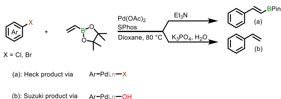
Figure I.13: Divergent cross-coupling exploiting on the different transmetalation rates
