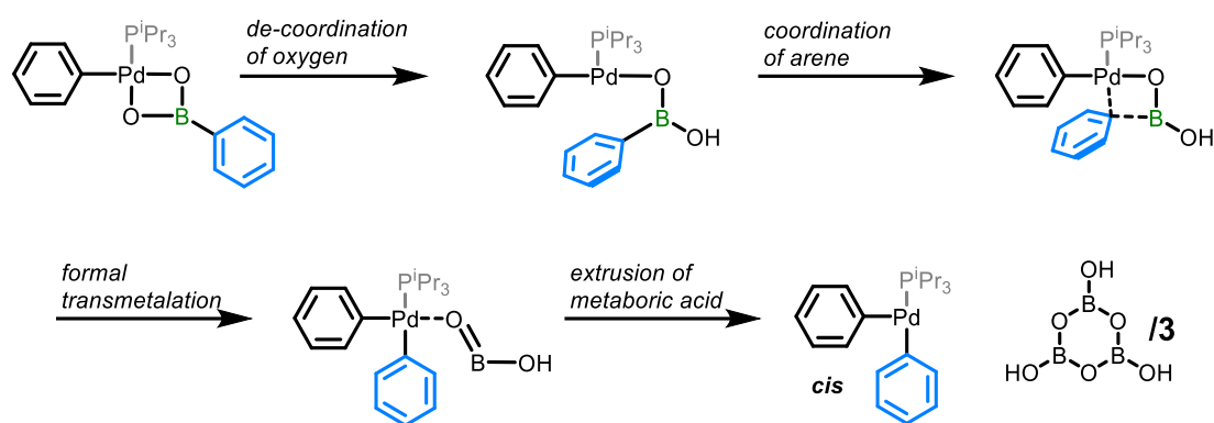
Figure I.16: Transmetalation via 6-B-3 intermediate (in presence of excess phosphine). The same steps have been located via DFT for the mechanism via the 8-B-4 intermediate.
