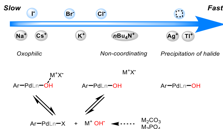
Figure I.14: Relative rate of transmetalation: inhibitory effects of base cation and halide
