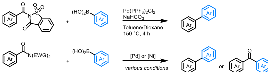
Figure I.46: Twisted amides in the Suzuki reaction
