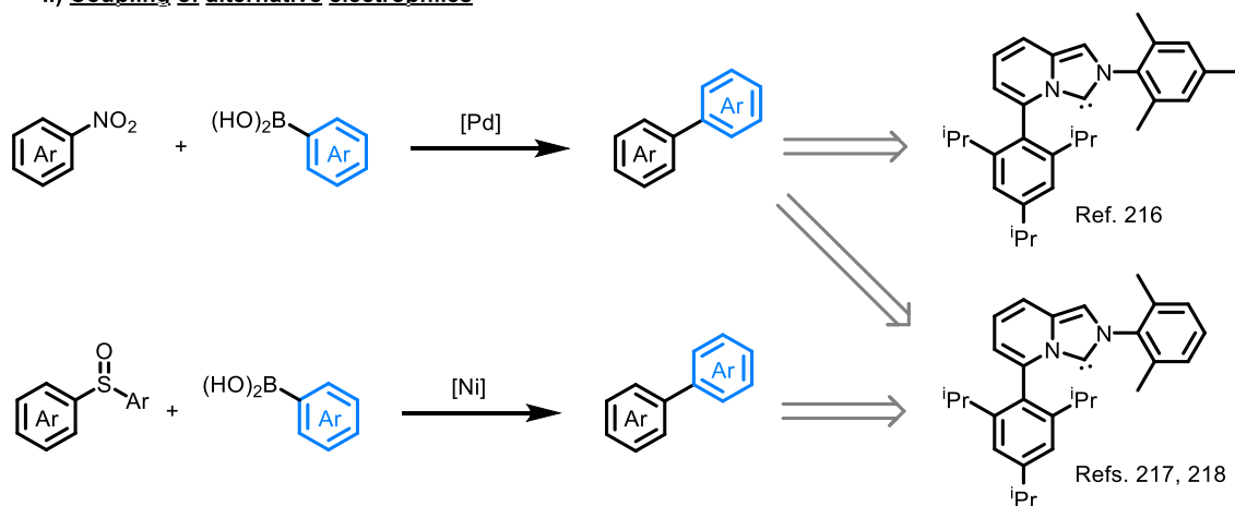
Figure I.32: Biaryl NHC ligands analogous to Buchwald ligands and their uses
