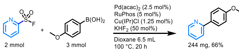
Figure III.4: Large-scale coupling of PyFluor
