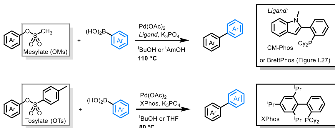
Figure I.40: Selected examples of methodologies for the Suzuki coupling of mesylates and tosylates
