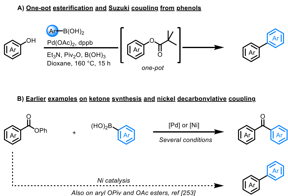
Figure I.43: Suzuki couplings on aryl esters
