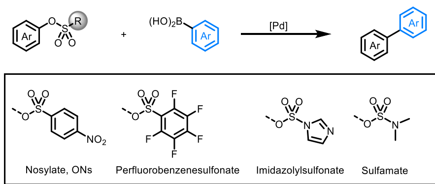
Figure I.41: Other sulfonyl-based electrophiles in the Suzuki reaction
