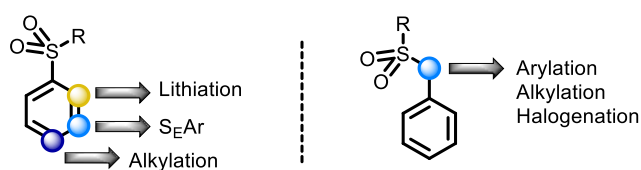
Figure IV.1: Sulfones as a synthetic handle for various transformations
