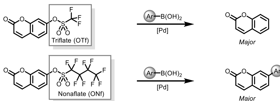
Figure I.38: Nonaflate and its higher stability compared to triflates.
