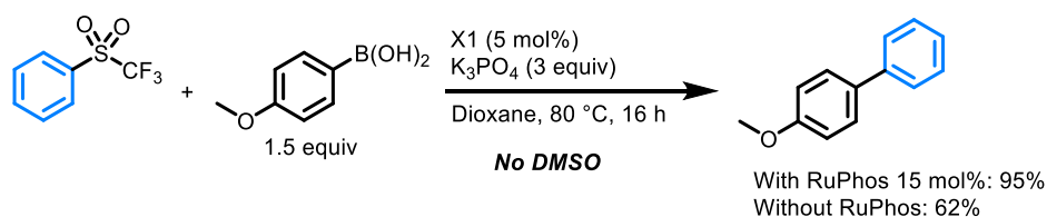
Figure II.3: Mechanistic experiments with intermediate X1
