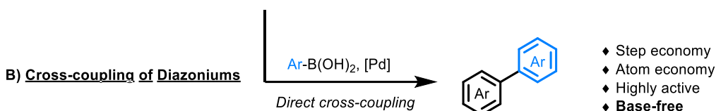
Figure I.35: Coupling of halides vs direct coupling of diazoniums
