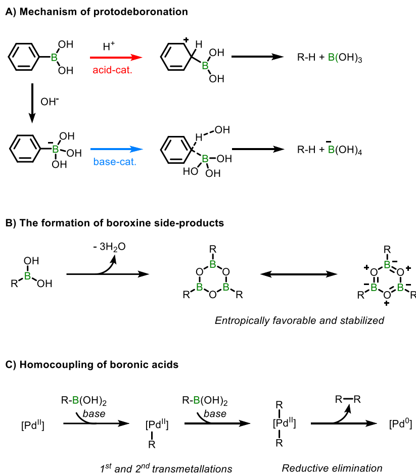
Figure I.3: Main side reactions related to boronic acids
