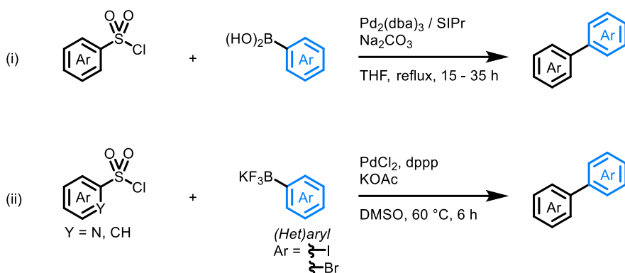
Figure I.53: The Suzuki coupling of sulfonyl chlorides: orthogonality to iodides and bromides
