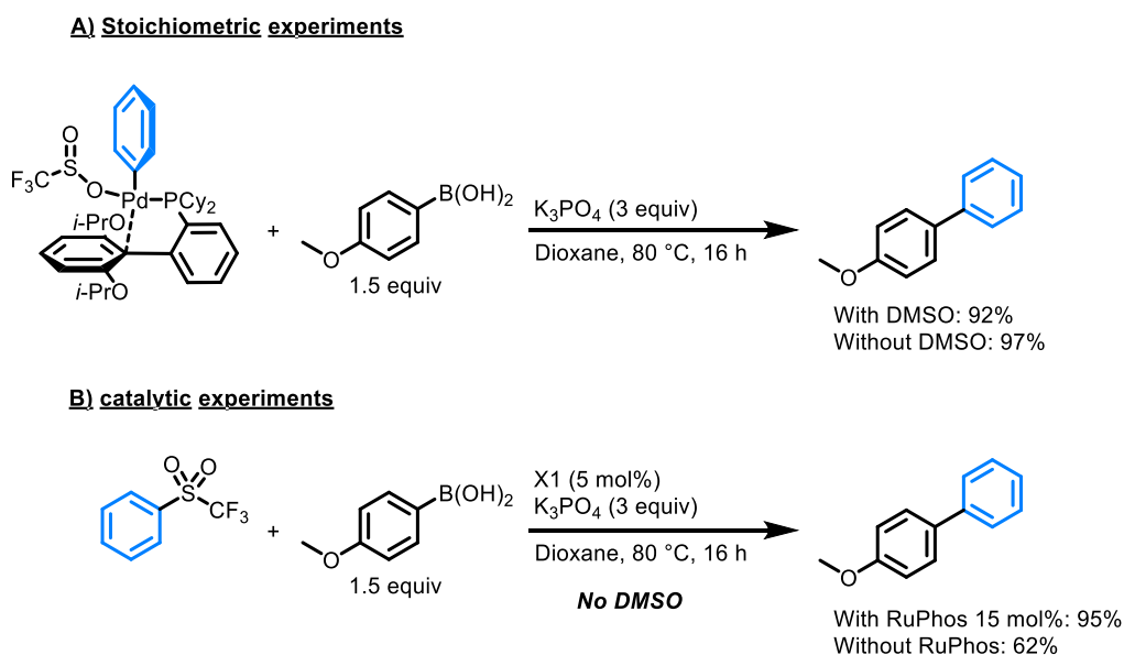
Figure II.3: Mechanistic experiments with intermediate X1
