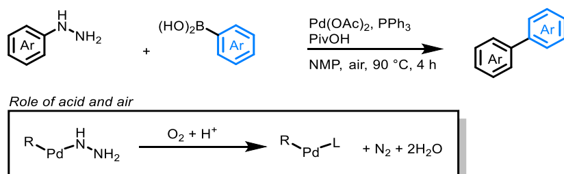
Figure I.48: Suzuki coupling requiring acid and oxygen: aryl hydrazines
