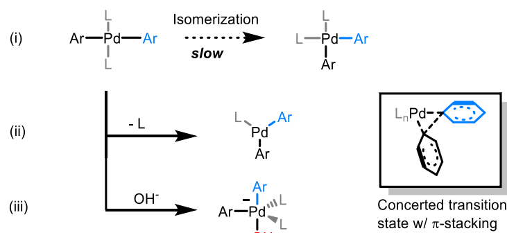
Figure I.22: Different pathways for accessing the reductive elimination transition step
