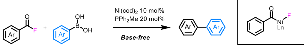
Figure I.18: Base-free couplings exploiting fluoride leaving groups to form reactive palladium fluoride complexes
