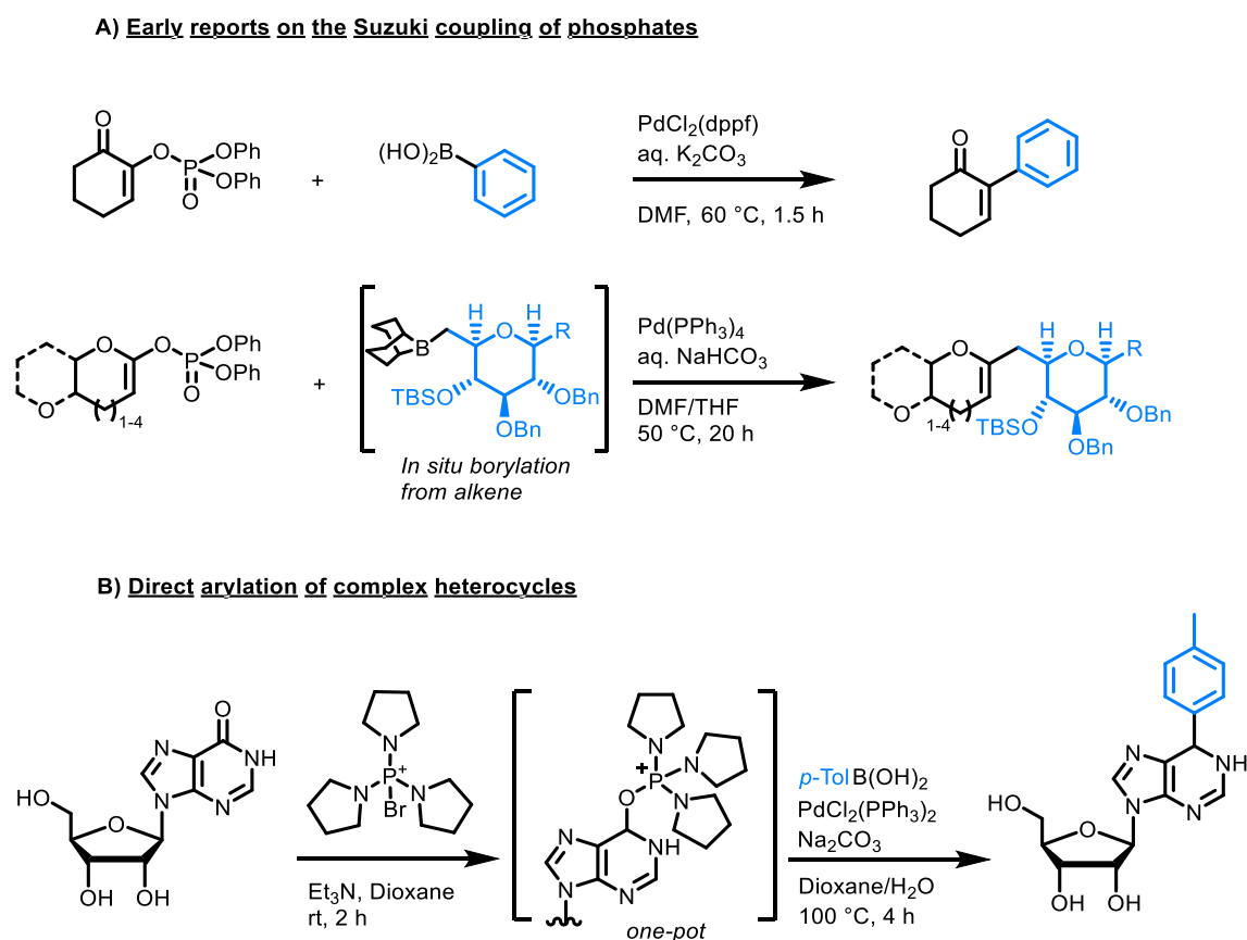
Figure I.42: Examples of Suzuki couplings on vinyl phosphates and phosphoniums
