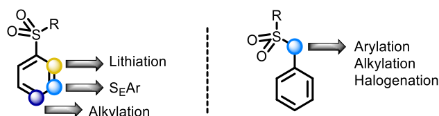
Figure I.56: Sulfones as a synthetic handle for various transformations
