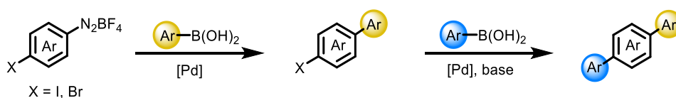
Figure I.36: High coupling activity of diazoniums
