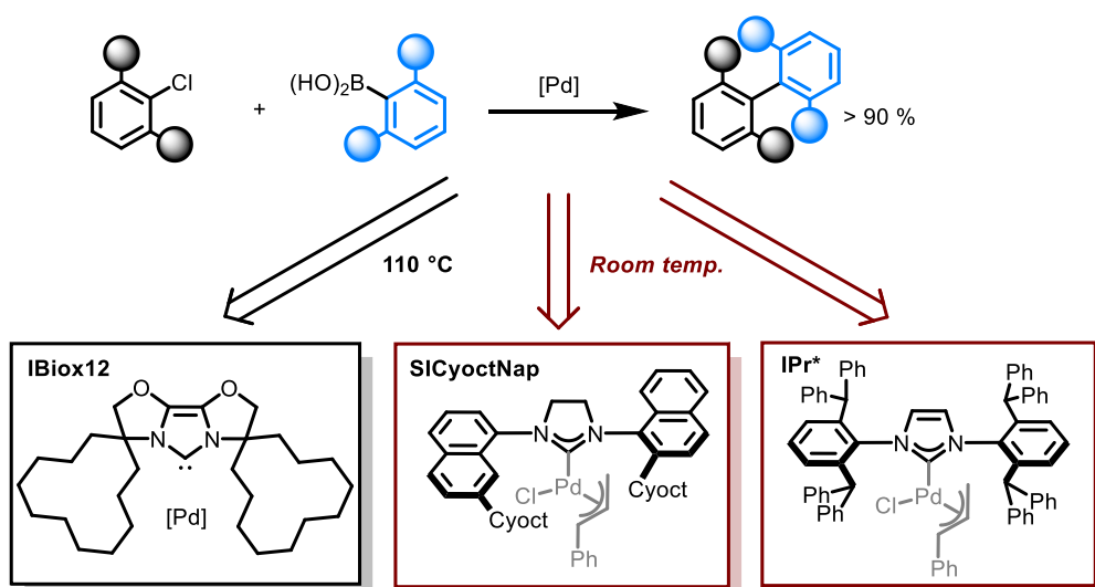
Figure I.31: Basic structure of NHC ligands and examples of challenging reactions
