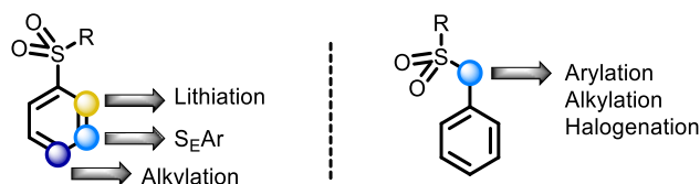
Figure II.1: Sulfones as a synthetic handle for various transformations
