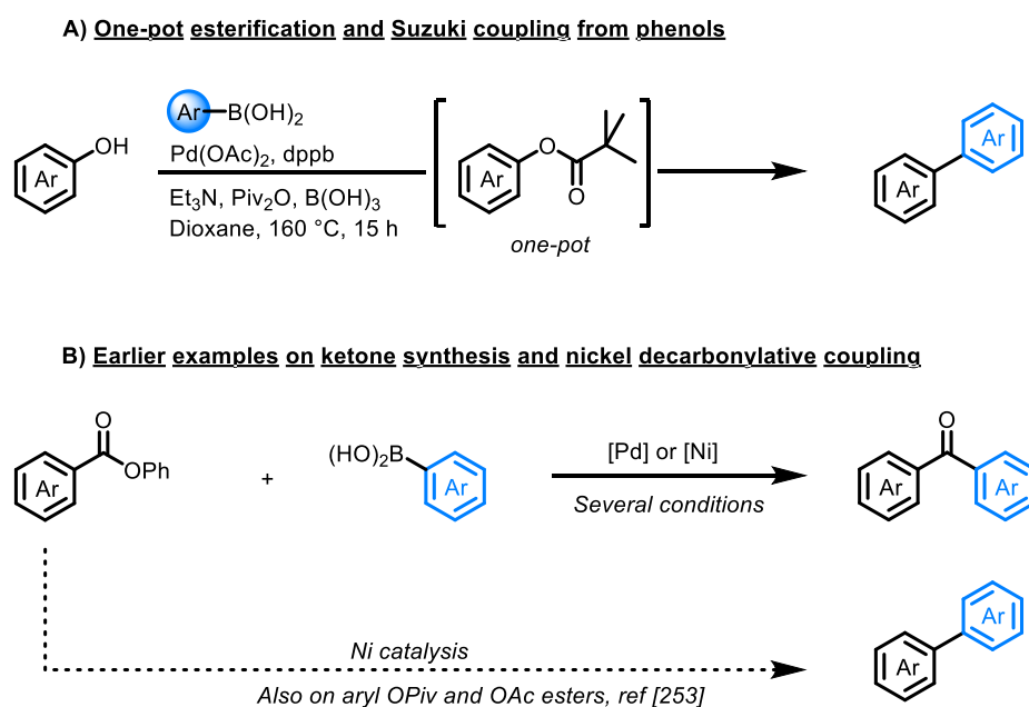
Figure I.43: Suzuki couplings on aryl esters
