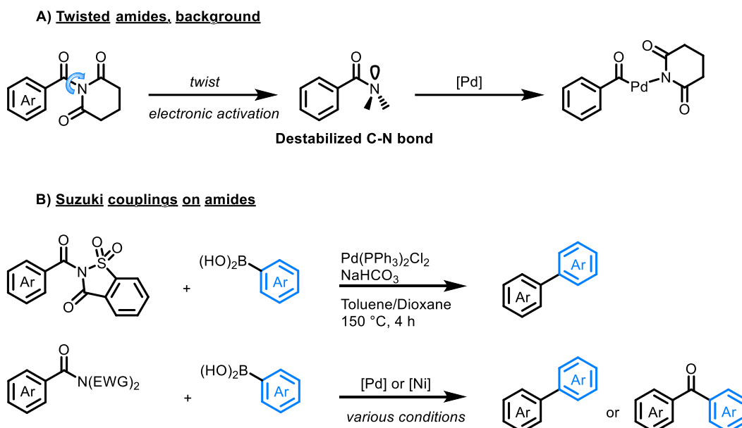
Figure I.46: Twisted amides in the Suzuki reaction
