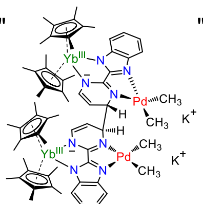
\text{Yb}(\text{bimpym})\text{Pd}
