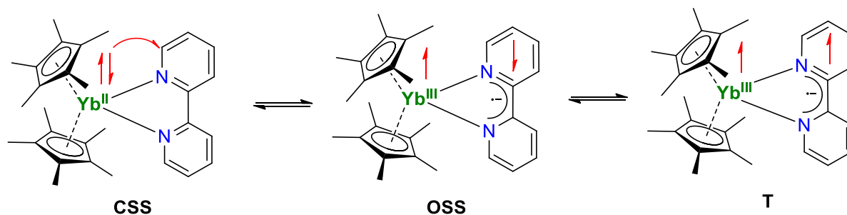
Scheme 8: Representation of the possible electronic configurations of the Yb -bipy system.
