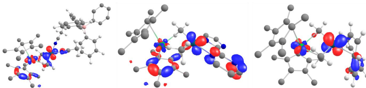
Figure 3.39: Examples of CASSCF orbitals of the YbPdL series, presenting involvement of other fragments of the molecules, other than the metal centres.
