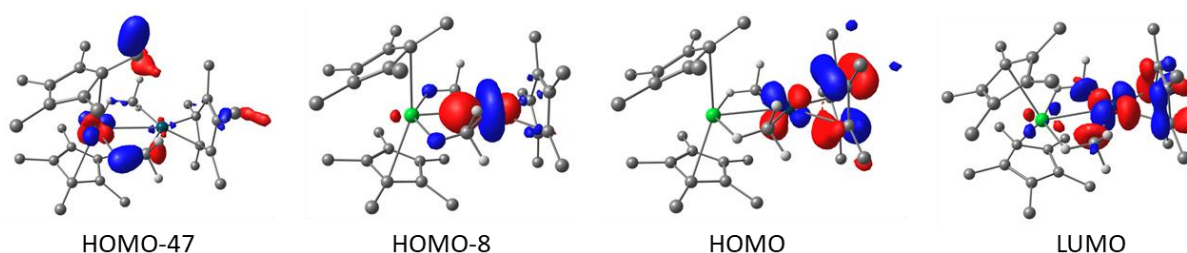
Figure 3.30: Main orbitals at the DFT level for 2.2 in the doublet configuration.
