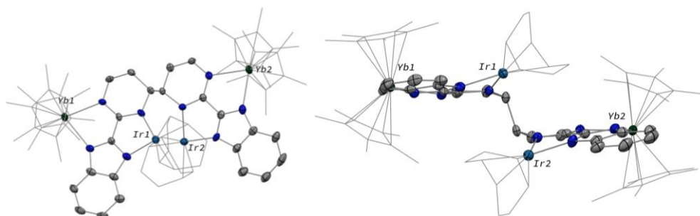
Figure 2.2 : ORTEP of 2.1 . The Cp* co-ligands are displayed in wireframe to avoid clutter.
