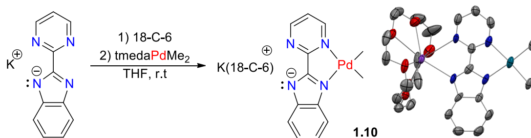
Scheme 1.13: Synthesis and ORTEP of 1.10 . The hydrogen atoms and the solvent molecules have been omitted for clarity.
