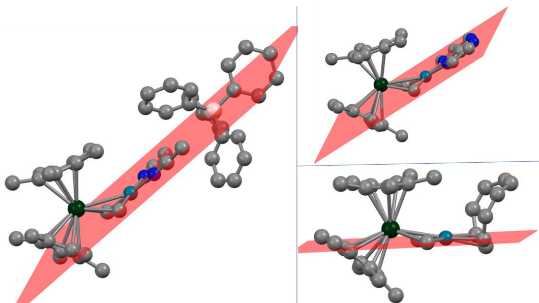
Figure 3.38: Computed structures of YbPdL , where L is the anion replacing Cp*. The plane determined by the Pd substituents is calculated (shown in red) to highlight the relative orientation with respect to the Yb centre. Left: YbPdBPh 4 ; top right: YbPd(impym) ; bottom right: YbPdCnt .
