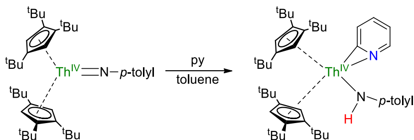
Scheme 3.6: C-H activation of pyridine by a Th imido complex. 49
