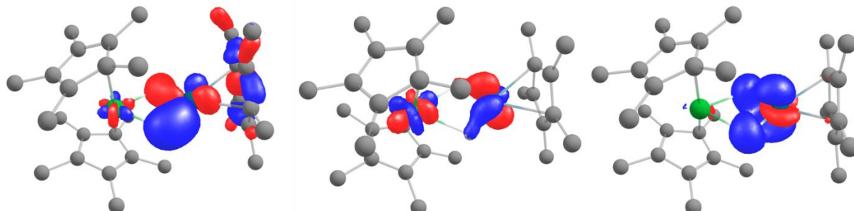
Figure 3.37: Main CASSCF orbitals of YbH 2 Pd , highlighting the orbitals involving the bridging hydrides.
