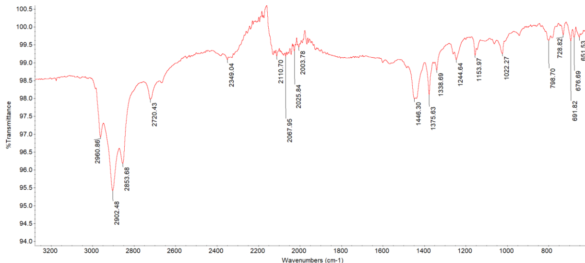
Figure 2.15: IR spectrum of 2.2 . The main bands are indexed.
