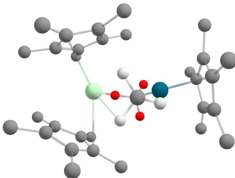
Figure 3.44: Structure of NdPd , oriented in a Newman-like projection. The H atoms belonging to the masked C atom are shown in red.
