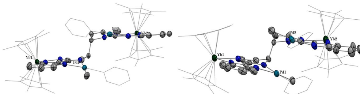
Figure 2.19: ORTEPs of 2.4 and 2.5 . The Cp* co-ligands and the pyridine moieties are set in wireframe to avoid clutter.
