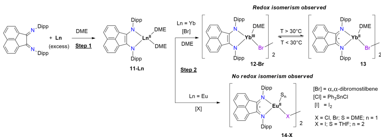
Scheme 5: Lanthanide-dependent redox isomerism in the Ln-bian system. 125–127
