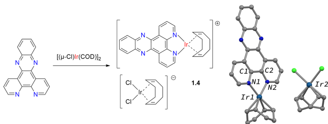
Scheme 1.6: Synthesis of 1.4 and its ORTEP.
