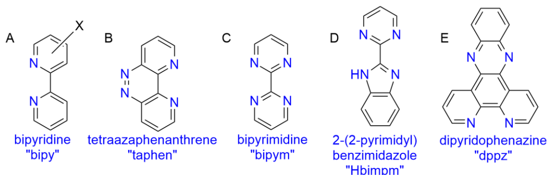
Scheme 1.1: Selection of RALs used in organolanthanide chemistry.
