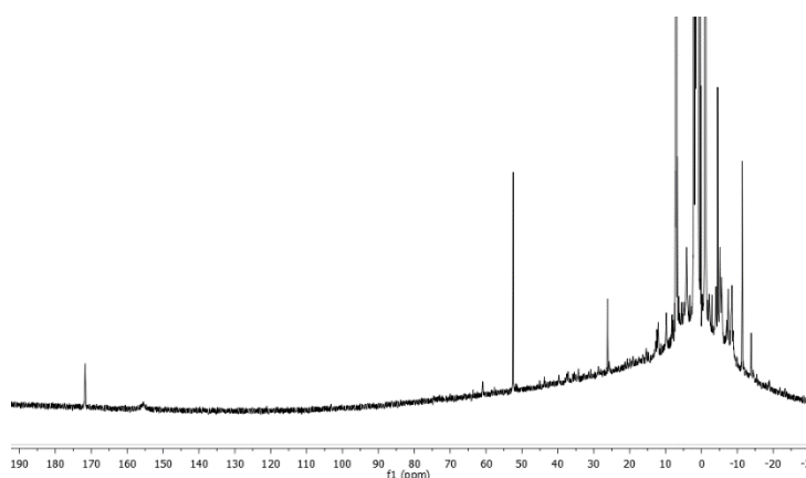
Figure 2.33: ^1\text{H} NMR of the reaction between yttrabocene and a Pd(bimpym) precursor that contains lutidine.
