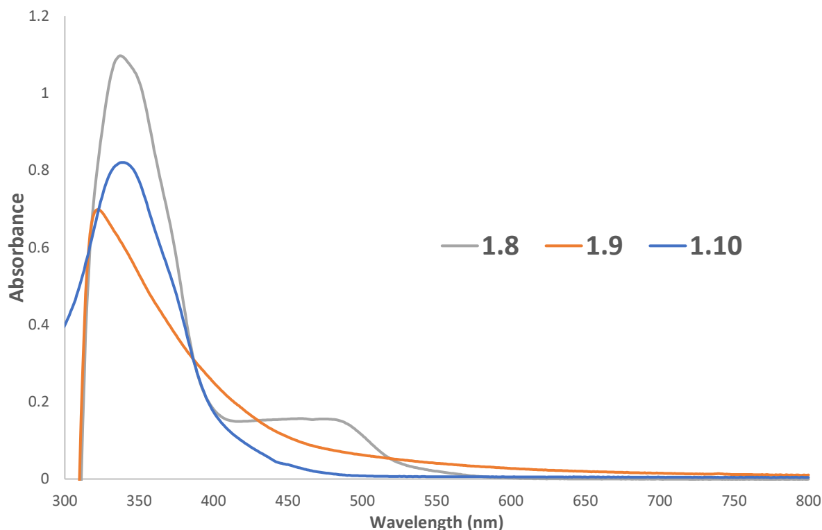
Figure 1.7: UV-Visible spectrum of Kbimpym -based complexes in THF.
