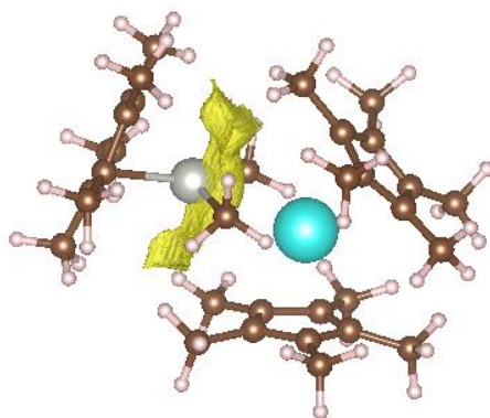
Figure 3.34: ELF valence basin interposed between the Yb and the Pd centres, found for 2.2 .
