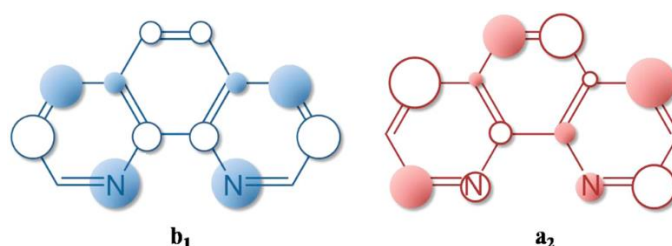
Figure 6: Representations of the LUMO ( b_1 symmetry) and LUMO+1 ( a_2 symmetry) orbitals. Adapted from ref 151.
