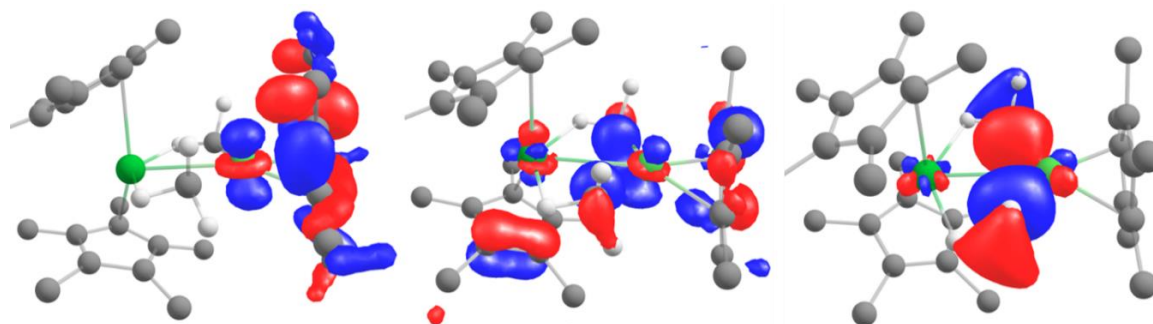
Figure 3.41: Preview of some of the more salient CASSCF orbitals of YbNi .
