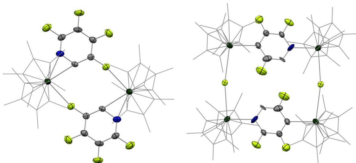
Figure 2.38: ORTEP of C-F activation-induced multimetallic complexes based on pentafluoropyridine 2.10 and 2.11 .
