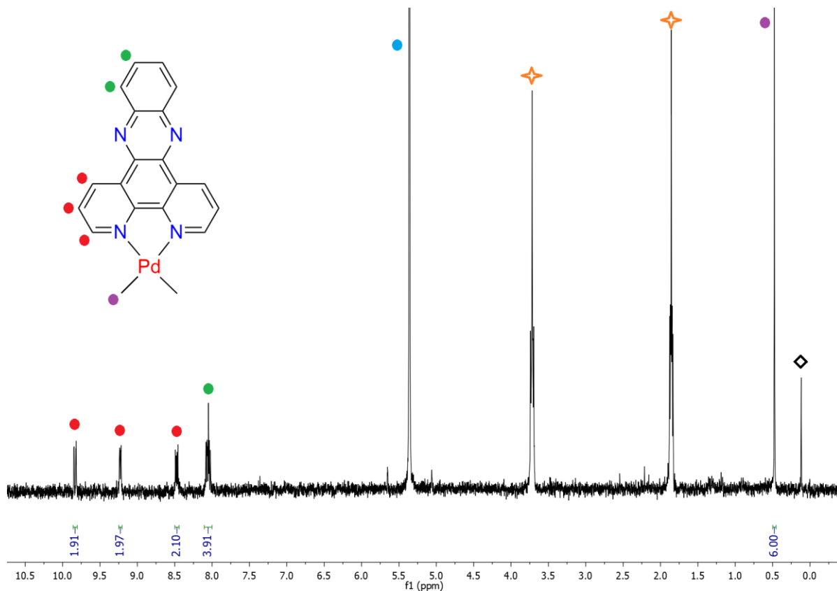
Figure 1.2: ^1\text{H} NMR in \text{CD}_2\text{Cl}_2 of 1.2 . The blue dot indicates the solvent peak, the orange four-pointed star – residual THF, black lozenge – silicone grease.
