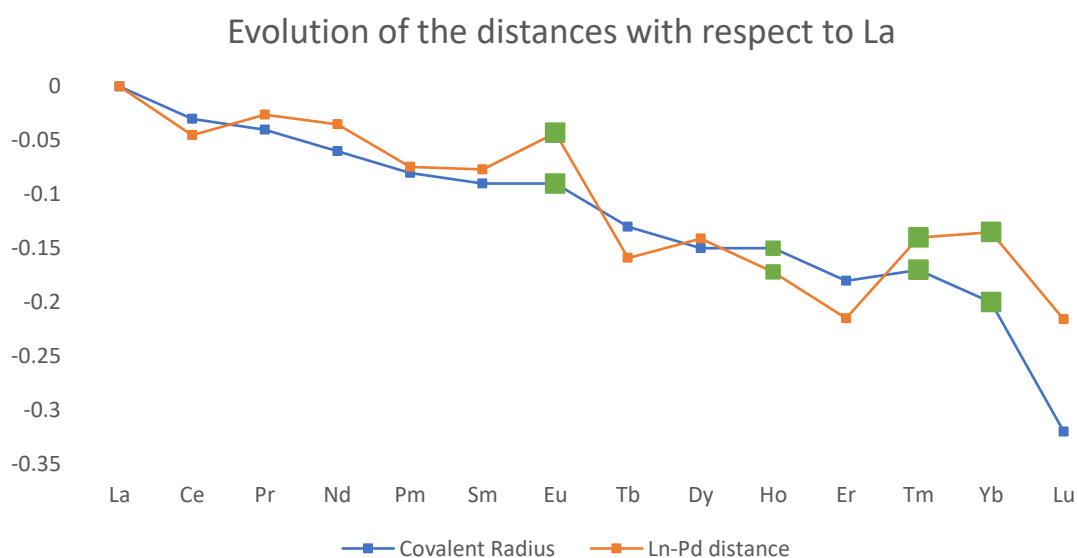
Figure 3.48: Evolution of the Ln-Pd distances, compared to the covalent radii of the lanthanide series. 88 Gd was excluded, due to the dubious optimisation. The complexes where there were 4f-Pd 4d interactions were found are designated by the green squares. The size of the square gives a measure of the strength of the interaction.
