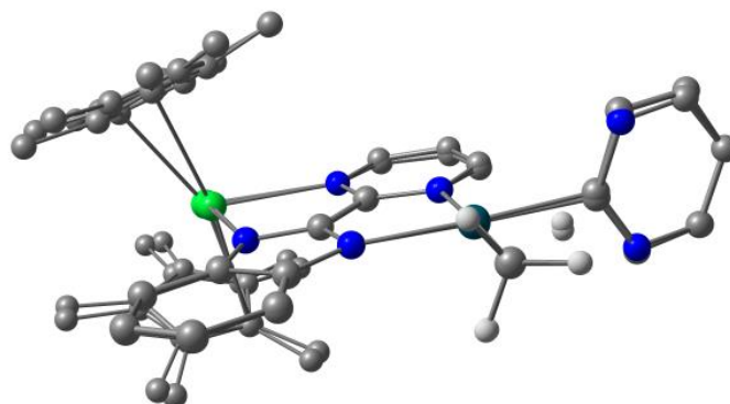
Figure 3.21: Overlay of Yb-TS and Sm-TS . The majority of H atoms are hidden in the interest of clarity.
