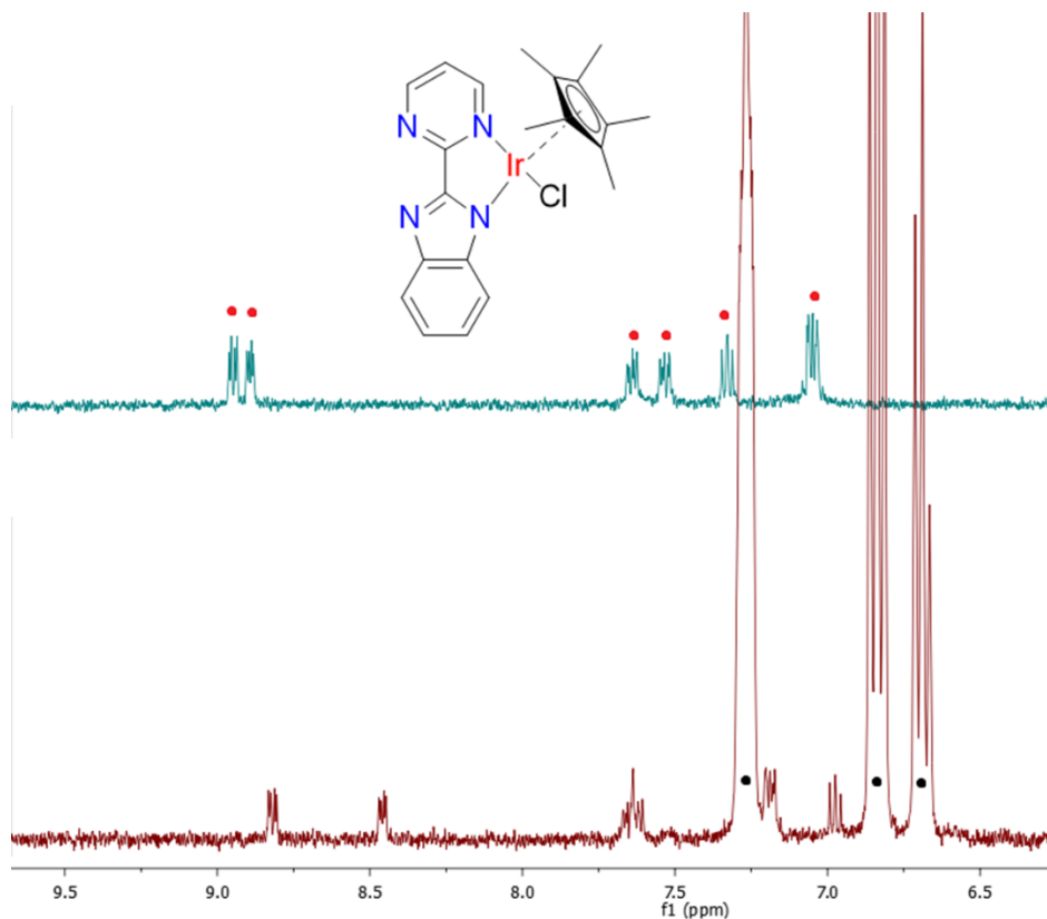
Figure 1.16: 1 H NMR in THF-d 8 of 1.18 (above, red dots) and after reaction with NaBPh 4 (below, black dots indicate reagent signals) – aromatic region.
