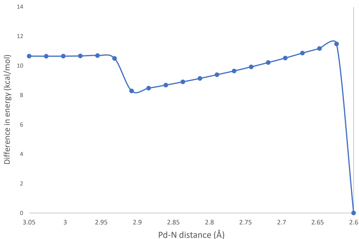
Figure 3.5: Evolution of the relative energy of the configurations examined throughout the second relaxed surface scan, in the 2.60-3.05 Å range. The configuration at d(\text{Pd-N}) = 2.60 Å is the most stable and is taken as the reference ( E=0 ). The line serves merely as a visual guide.
