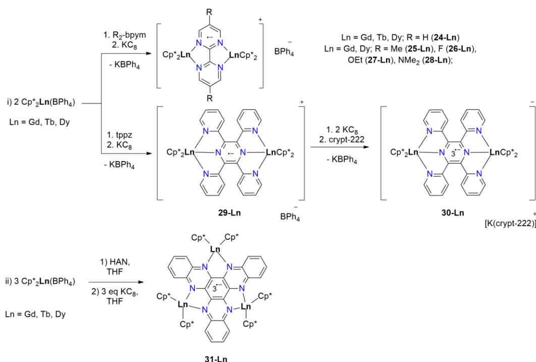
Scheme 12: Synthesis of bi- and trimetallic radical ligand systems. 153–156 "HAN" = hexaazatrinaphthylene.
