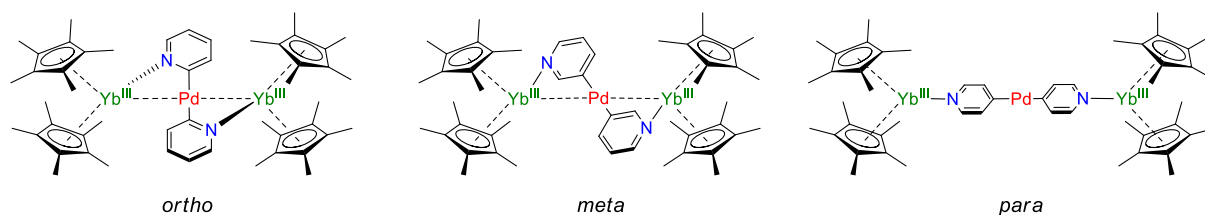
Scheme 3.7: Complex 2.6 and putative homologues, where the C-H activation occur in the meta or para positions.
