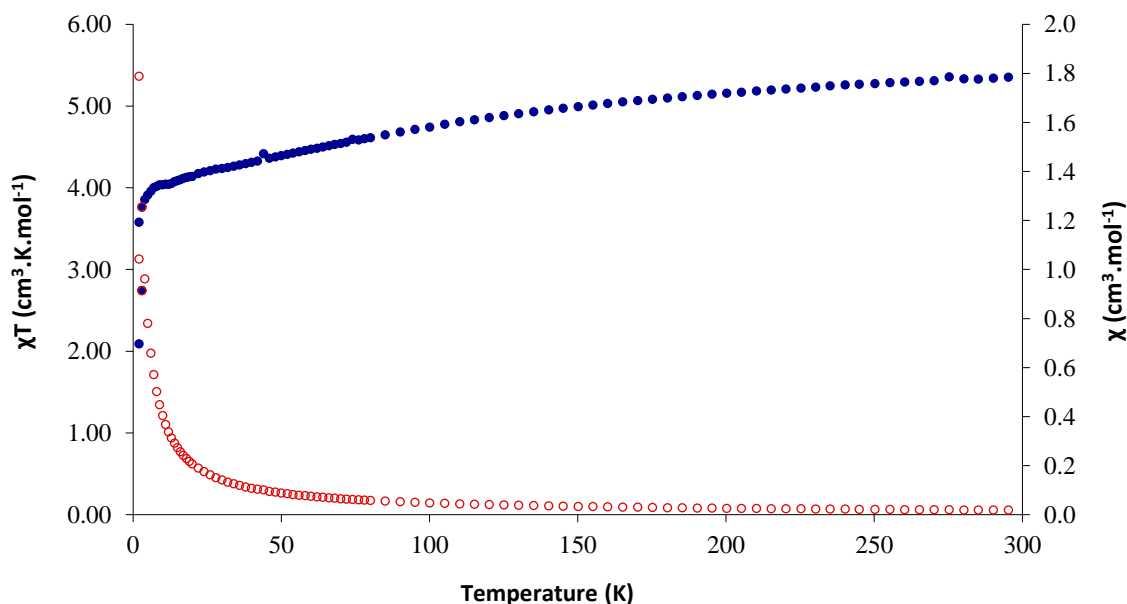
Figure 2.29: Magnetic susceptibility (unfilled red dots) and the \chi T product (filled blue dots) for 2.6 .
