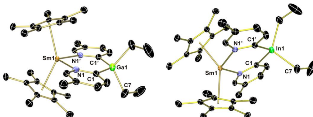
Figure 2.25: ORTEP of a structurally similar Ln III -TM(pyr) complex, reprinted from the given reference. 51
