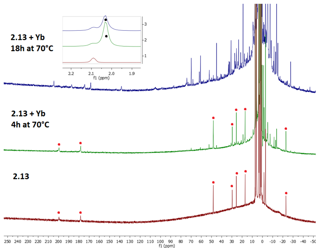
Figure 2.44: ^1\text{H} NMR of 2.13 in \text{tol-d}_8 and the evolution when excess ytterbocene is added and the mixture is kept at 70^\circ\text{C} . The red dots indicate the bimpym peaks of the product, the black dot indicates the \text{Cp}^* signal of ytterbocene.
