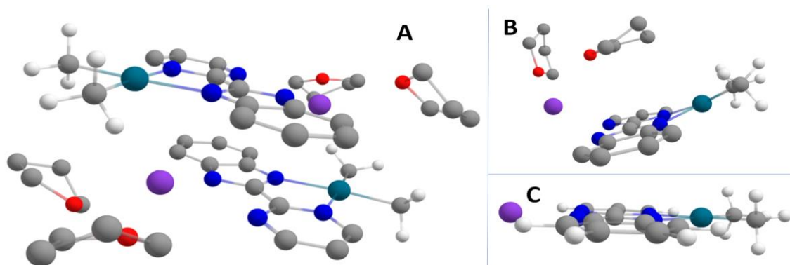
Figure 1.5: Structure of 1.9 , computed in different configurations at the ZORA1 level of theory.
