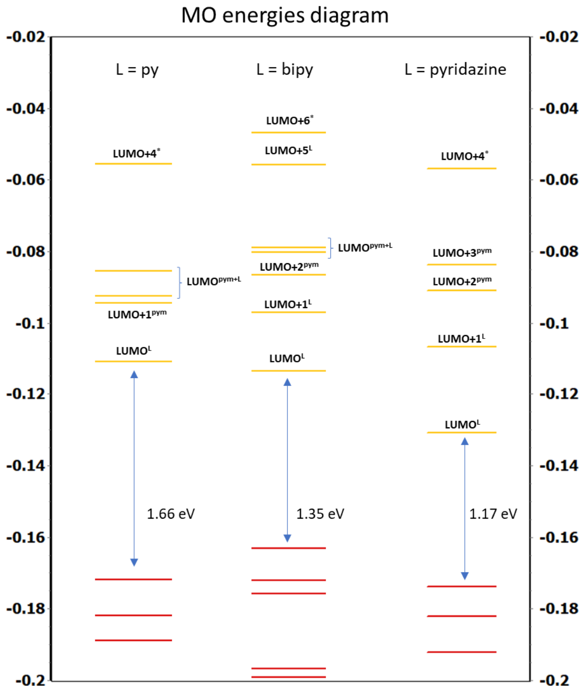
Figure 1.13: MO energy diagram (in Eh) for 1.12 and the corresponding pyridazine and bipy analogues, computed at the ZORA1 level of theory. The red and yellow dashes indicate occupied and vacant orbitals, respectively.
