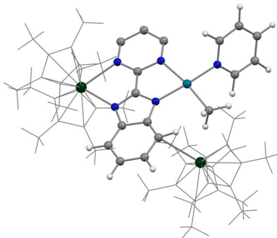
Figure 3.25: Structure of 1.12-Yb 2 ' , computed at the ZORA1 level of theory. The Cp* are set in wireframe and most of the H atoms are hidden for clarity.
