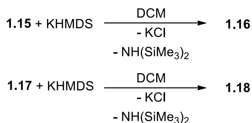
Scheme 1.21: Deprotonation attempts of Hbimpym -based complexes.
