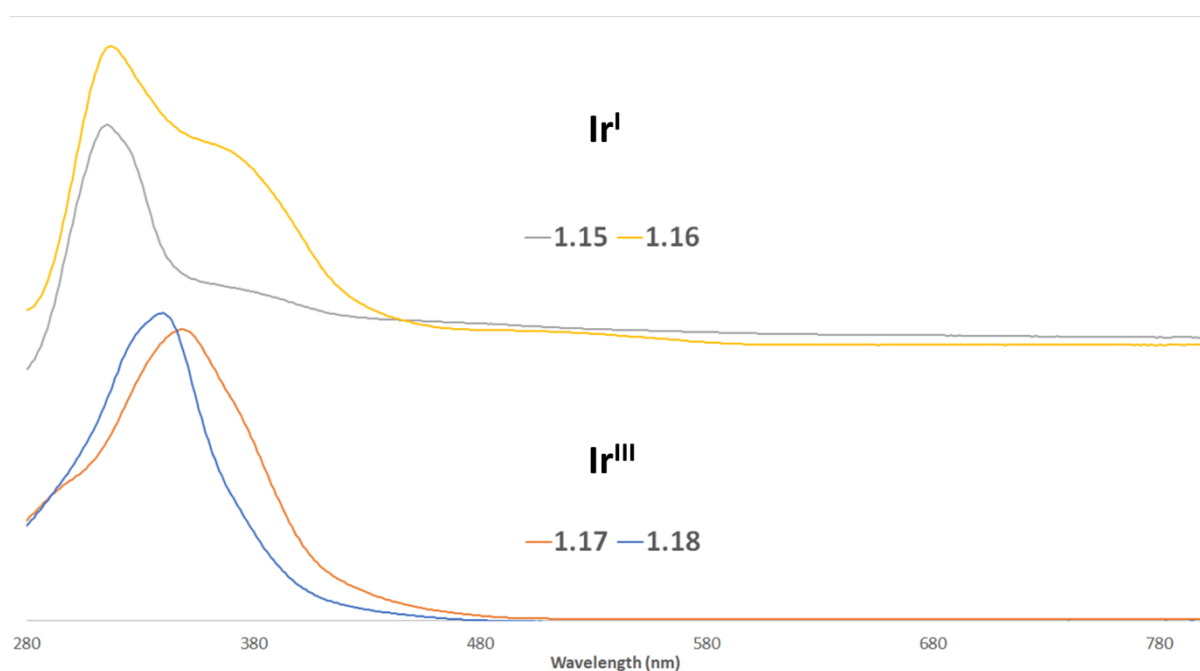
Figure 1.15: Overlay of UV-Visible spectra of 1.15-1.18 in DCM.
