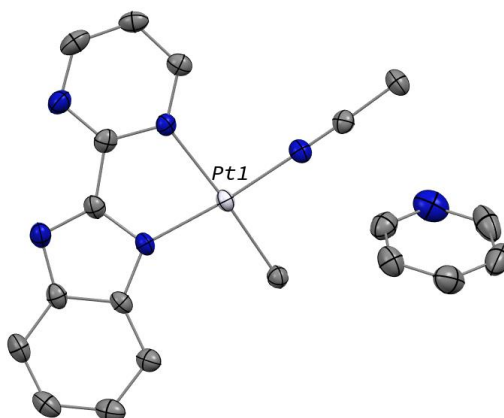
Figure 1.10: ORTEP of 1.14 . The pyridine molecule co-crystallises with the complex. The hydrogen atoms are omitted for clarity.
