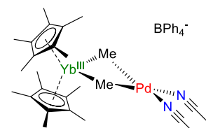
YbPdBPh 4
