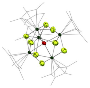
Figure 2.31: ORTEP of a side-product following the addition of pentafluoropyridine to 2.7 .
