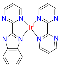
(\text{bimpym})\text{Ir}(\text{bipym})
