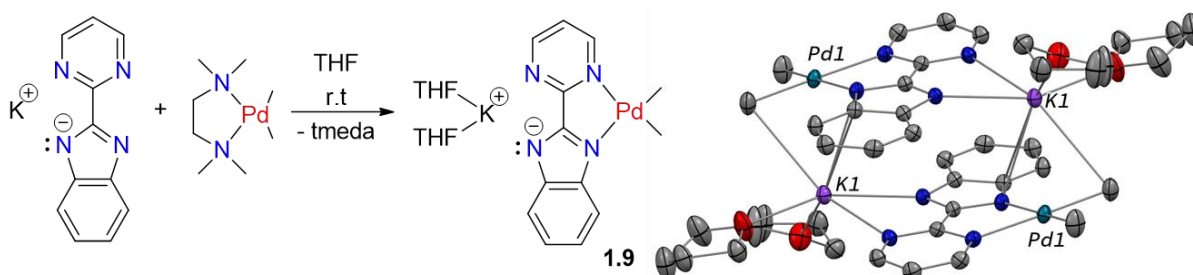
Scheme 1.12: Synthesis and ORTEP of 1.9 . Hydrogen atoms have been hidden for clarity.
