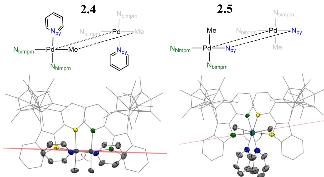
Figure 3.17: Schematic representation and the corresponding simplified ORTEPs of the relative orientations of the pyridine and methyl moieties in the two Pd coordination spheres on 2.4 and 2.5 , viewed from above. Planes were calculated based on the substituents of the Pd centre. In both cases, the maximum available space for an ytterbocene approach would be from below the plane shown in the figure. The angle formed between these two substituents is shown for emphasis. The N atoms of the bimpym ligands closer to the viewer's perspective are shown in green, the ones farther in yellow.
