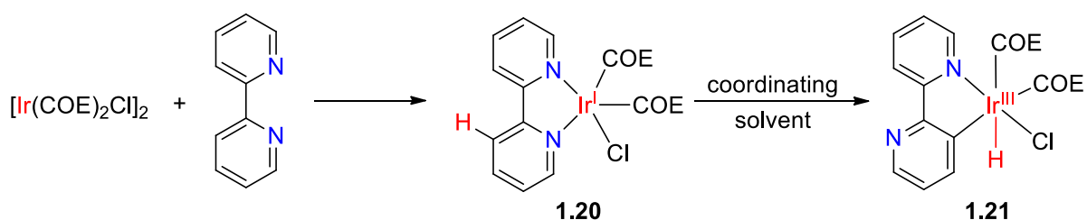
Scheme 1.27: Proposed mechanism for the reaction between bipy and [Ir(COE) 2 Cl] 2 .
