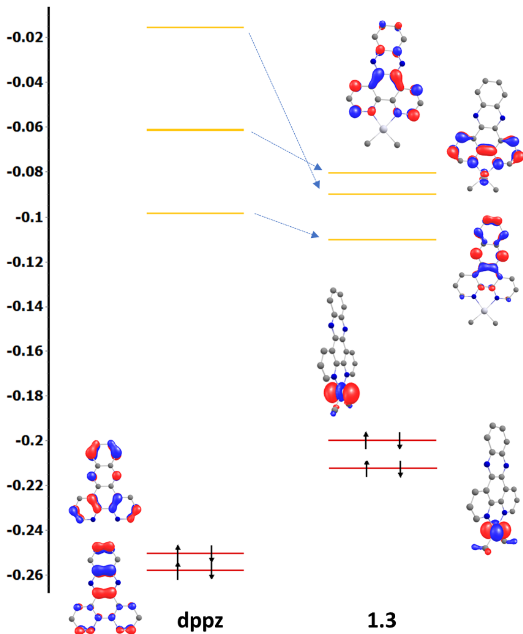
Figure 1.1: MO diagram of dppz and of 1.3 , calculated at the ZORA3 level of theory. The occupied orbitals are designated by the red dashes with arrows, whilst the vacant orbitals are represented by the yellow dashes. The LUMOs of dppz are identical in shape to the ones presented for 1.3 (excluding the TM fragment), but are not presented in the interest of clarity. The energies are given in Eh.
