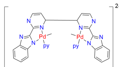
2.5 dian
