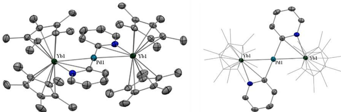
Figure 2.24: ORTEP of 2.6 from two perspectives. The hydrogens are not shown and the Cp* groups are shown in wireframe in the second perspective in the interest of clarity.
