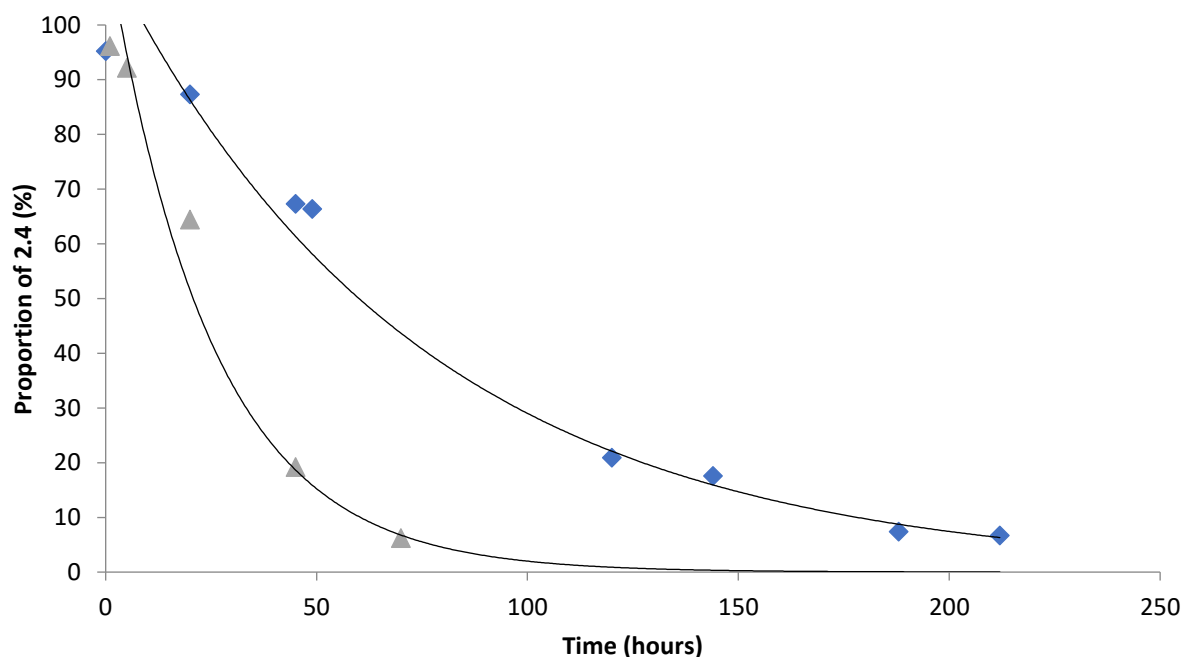
Figure S1: Time evolution (hours) of the clean isomerisation of 2.4 to 2.5 without (blue lozenges) and with stirring (grey triangles).
