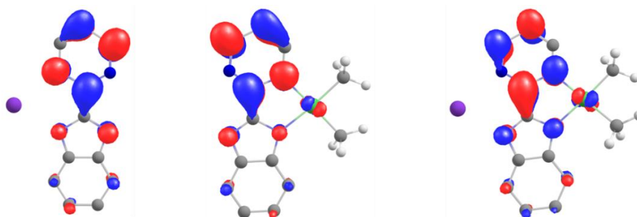
Figure 1.6: The LUMOs of Kbimpym , bimpymNiMe 2 - and KbimpymNiMe 2 , computed at the ZORA3 level of theory.
