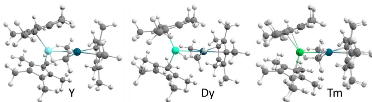
Figure 3.45: Examples of the overlay of the geometries obtained using Loose and Tight convergence criteria.
