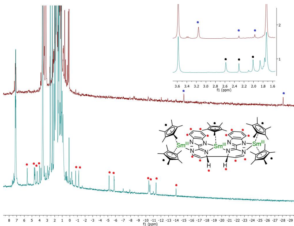
Figure 2.11: ^1H NMR of 2.3 (below) and of the product following recrystallisation of 2.3 (blue dots, above) in Et_2O .
