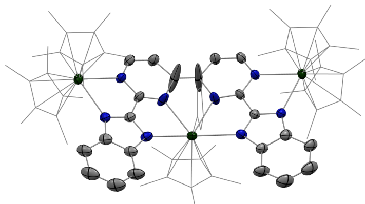
Figure 2.10: ORTEP of 2.3 . The Cp^* co-ligands and the THF coordinated to the central Sm are set in wireframe for clarity.
