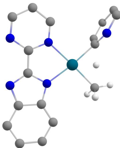
Figure 3.7: Structure of 1.12-TS , computed at the TS1 level of theory.
