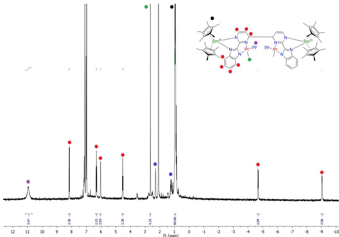
Figure 2.42: 1 H NMR of 2.14 in tol-d 8 . Residual solvent peaks of toluene and pentane are designated by the blue dots.
