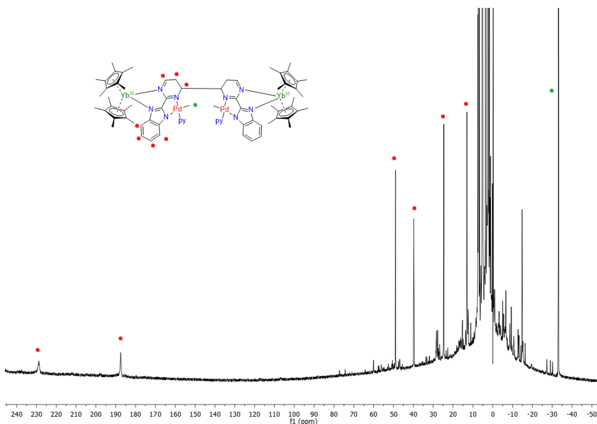
Figure 2.34: ^1\text{H} NMR of the main product following the addition of ytterbocene to 1.12 in the presence of an excess of lutidine.
