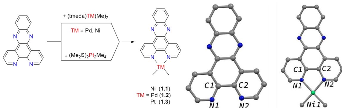
Scheme 1.5: Synthesis of (\text{dppz})\text{TMMe}_2 complexes 1.1-1.3 and ORTEP of \text{dppz}^{42} and of \text{dppzTMMe}_2 -type complexes ( 1.1 shown here). The numbering scheme shown here is used throughout the chapter.
