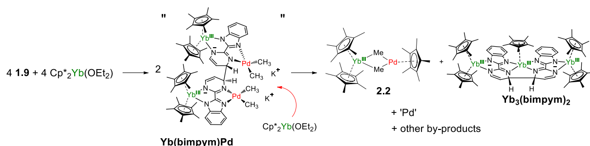
Scheme 2.3: Two propositions for the reaction mechanism. The second one, which involves the interaction with another ytterbocene molecule, is shown with the red arrow.
