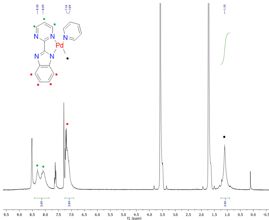
Figure 1.9: ^1\text{H} NMR of complex 1.12 in \text{THF-d}_8 at 333 K.
