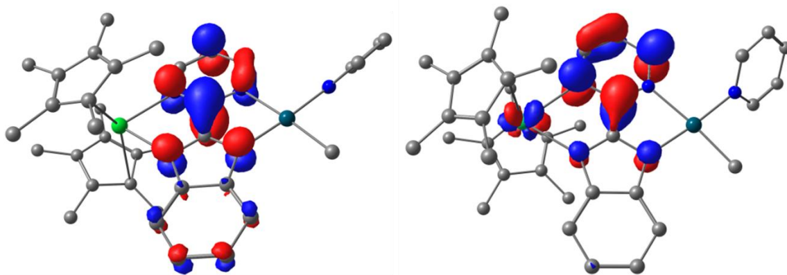
Figure 3.20: Alpha SOMO on the computed heterobimetallic adducts 1.12-Yb (left) and 1.12-Sm (right).
