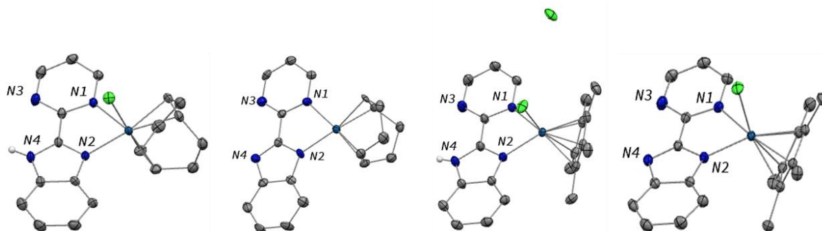
Figure 1.14: ORTEP of complexes 1.15-1.18 . All the hydrogen atoms (except for the ligand proton in 1.15 and 1.17 ) are omitted for clarity. The labelling on the nitrogen atoms is adopted for the rest of the section.
