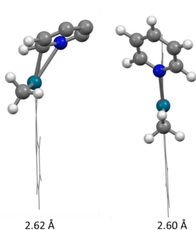
Figure 3.6: The evolution of the optimised geometries upon the reduction of the \text{Pd-N}_{\text{py}} distance, when the coordination mode of the pyridine switches towards coordination by the N atom. The bimpym ligand is shown in wireframe and only the most significant hydrogen atoms are shown.
