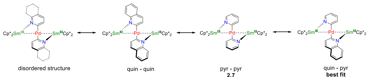
Scheme 3.12: All the potential structures of 2.8 , based on the interpretation and resolution of the structural disorder.
