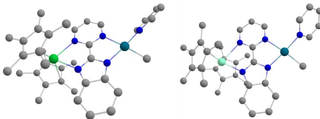
Figure 3.19: Structures of 1.12-Yb and 1.12-Sm , obtained at the ZORA1 level of theory.
