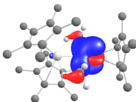
Figure 3.50: Pd 4d-dominated orbital found in all the complexes of the computed REPd series.
