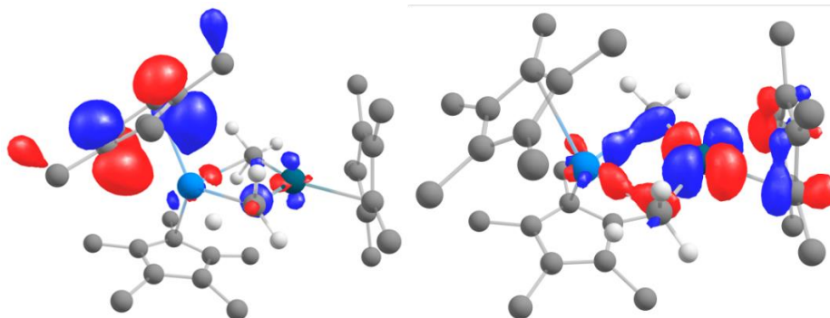
Figure 3.47: Preview of the CASSCF orbitals of UPd , where both metals participate.
