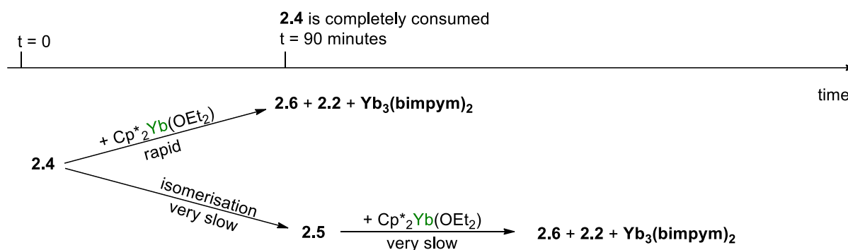
Scheme 3.9: Schematic representation of the timeline of the reaction. The reactivity of the initial quantity of 2.5 is neglected.
