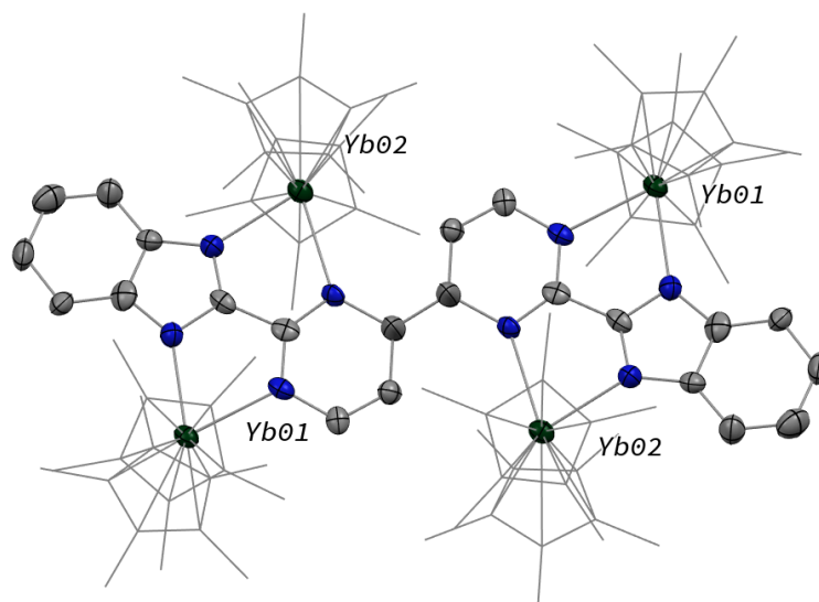
Figure 3.15: ORTEP of 3.2 , isolated in the later crystallisation fractions after the addition of ytterbocene to 1.12 .
