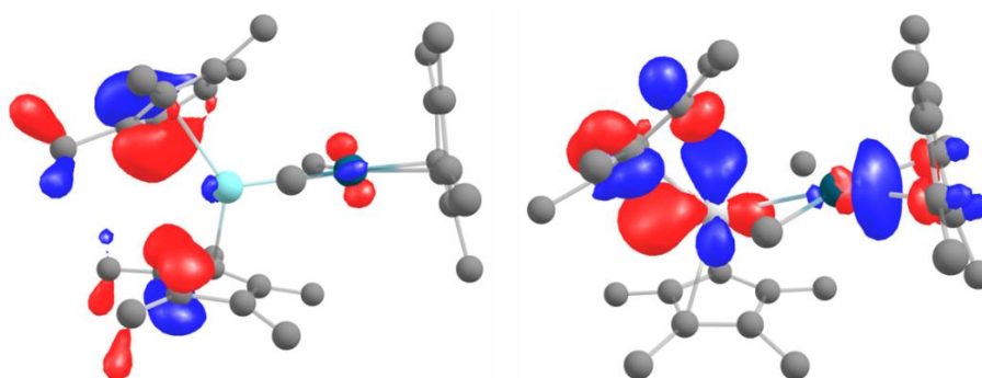
Figure 3.46: Examples of CASSCF orbitals of group 3 complexes, showing Pd-dominated interactions with the bridging methyls and an orbital in the active space with contributions from unoccupied orbitals of the Sc centre.
