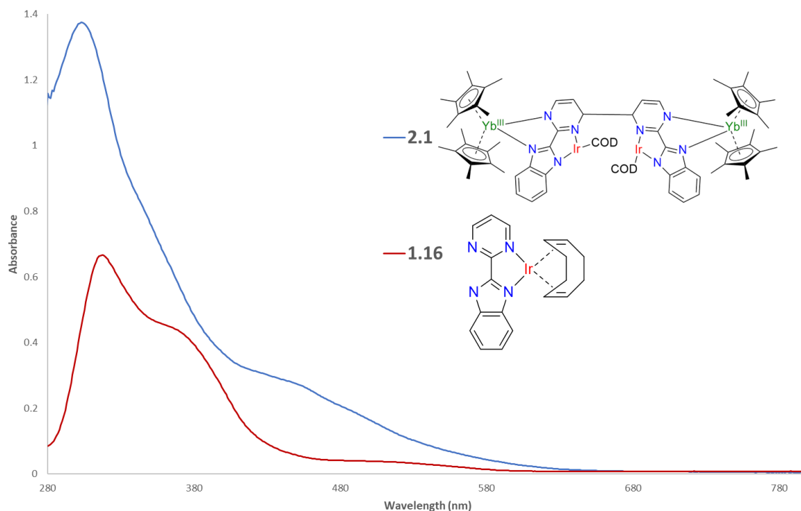
Figure 2.3: UV-Visible spectra of the (bimpym)IrCOD complexes 1.16 and 2.1 .
