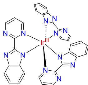
\text{Ir}(\text{bimpym})_3
