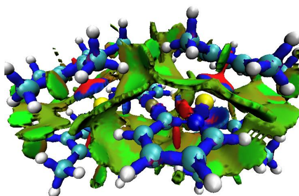
Figure 3.35: NCI plot of 2.7 . Colour-code: repulsive forces – red, covalent interaction – blue, non-covalent interaction – green.
