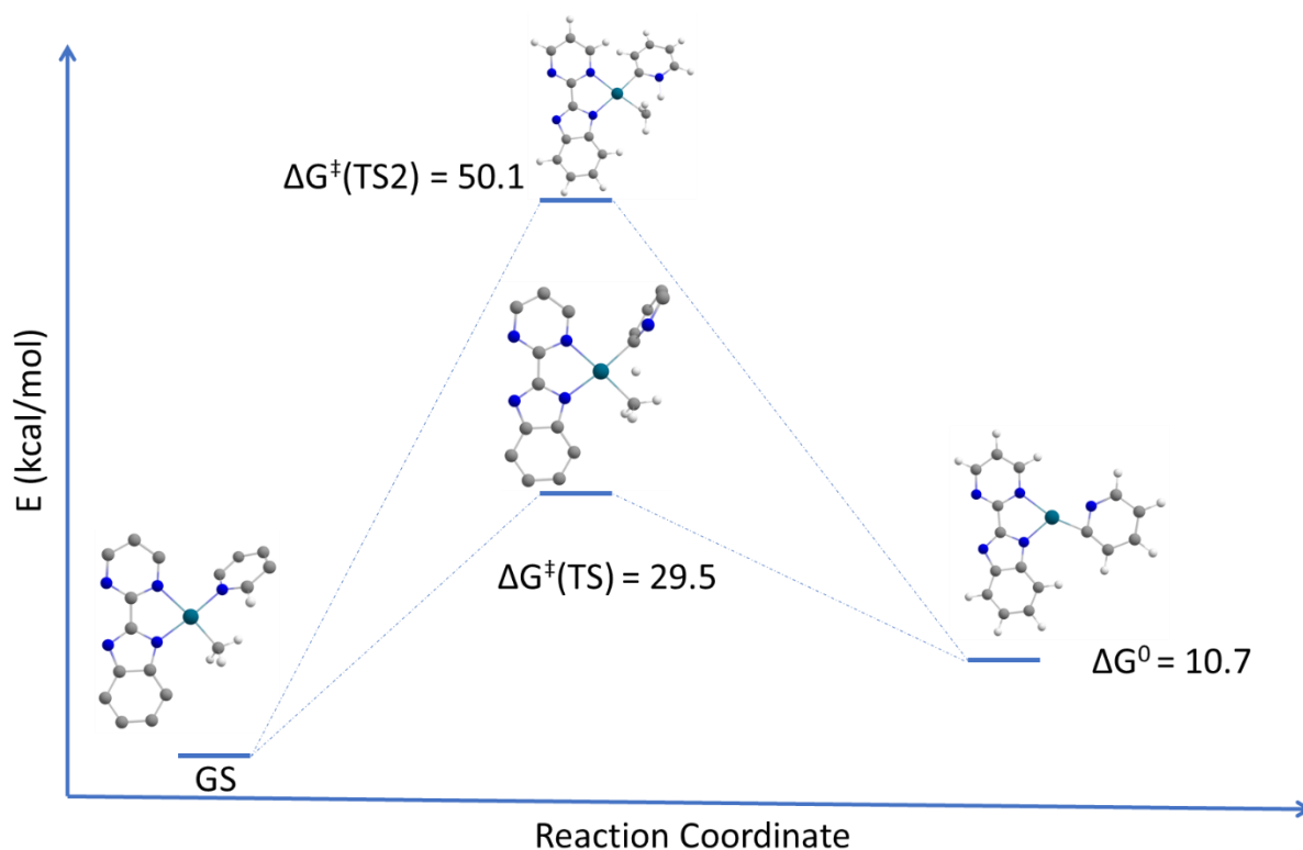
Figure 3.10: Schematic representation of the two computed TS with respect to the energy of the transformation. The relative energies of the computed states are not up to scale.
