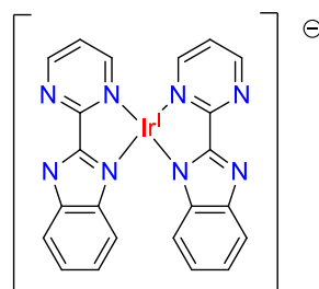
[(\text{bimpym})_2\text{Ir}]^-
