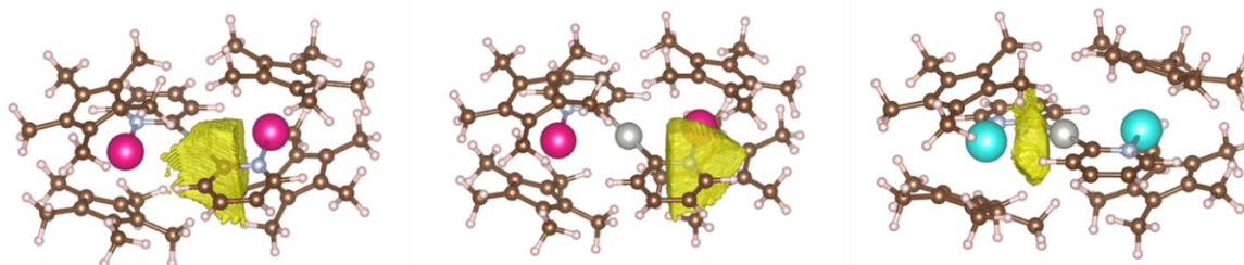
Figure 3.33: Main ELF valence basins found for the trimetallic complexes, illustrating the Pd-C pyr bond (left), Ln-N pyr (centre, both computed for 2.7 ) and the Yb-Pd interaction (right, only found for 2.6 ).
