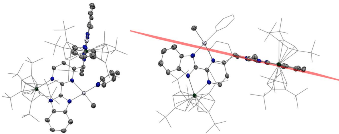
Figure 2.41: ORTEP of 2.15 . The hydrogen atoms are hidden and the Cp ttt groups are set in wireframe for clarity. The lack of deviation from planarity on the pyrimidine moiety is demonstrated by the neat arrangement within the plane formed by its composing atoms.
