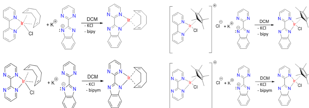
Scheme 1.25: Ligand substitution reactions with (L)IrCODCl and (L)IrCp*Cl 2 (L = bipy, bipyridine).
