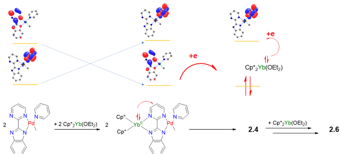
Scheme 2.8: Schematic representation of the electronic perturbation and subsequent population of the main vacant orbitals of 1.12 upon the addition of ytterbocene. The orbitals of 1.12 are used as visual references in the heterobimetallic adducts.
