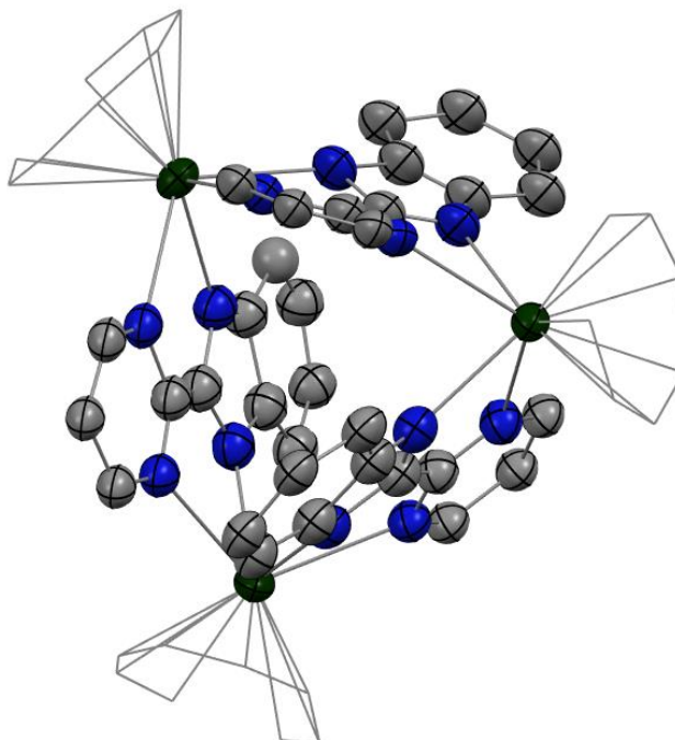
Figure 1.8: ORTEP of 1.11 . The COT ligands are shown in wireframe to avoid clutter.
