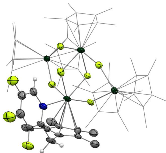
Figure 2.39: ORTEP of 2.12 . The Cp* co-ligands are set in wireframe in the interest of clarity.
