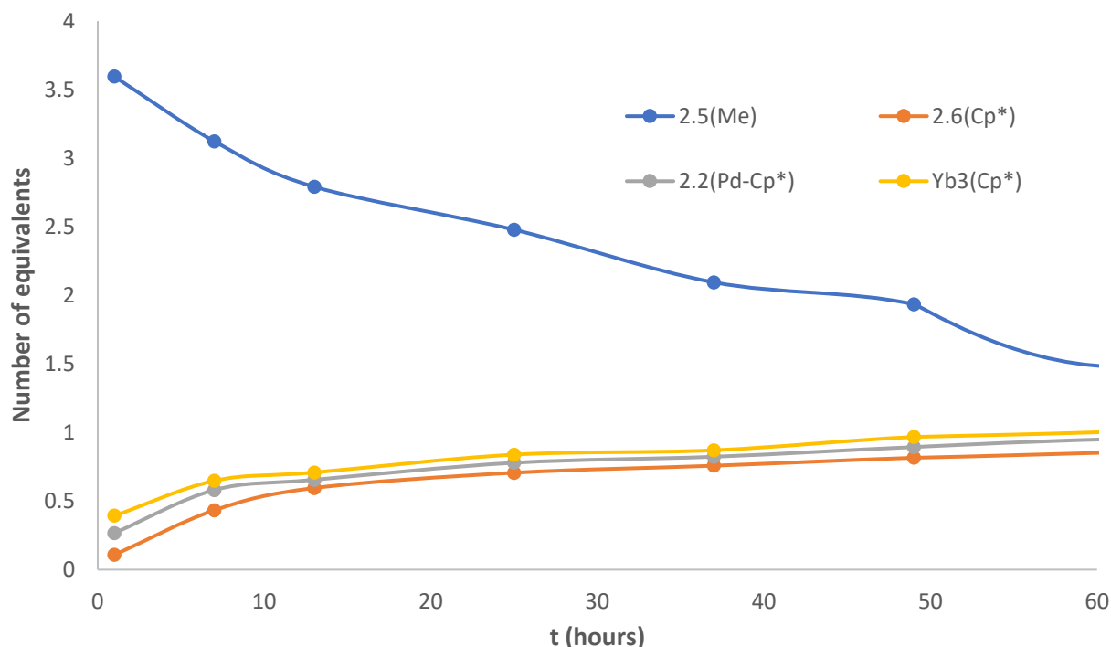
Figure 3.14: Kinetic study of the reaction between 2.5 and an excess of ytterbocene in tol-d 8 . The number of equivalents of each species was calculated with respect to an internal reference. Cp* 2 Yb(OEt 2 ) could not be reliably integrated at all times and is not included. Yb 3 (bimpym) 2 was shortened to “Yb3” in the interest of clarity.
