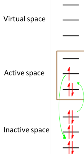
Figure 3.29: Principle of orbital permutations at the CASSCF level.
