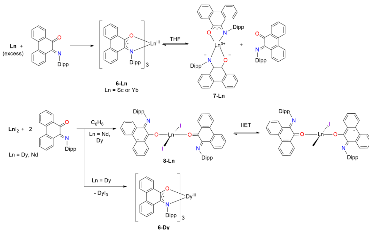
Scheme 3: Formation and reactivity of Ln-based compounds with iminoquinones. 123
