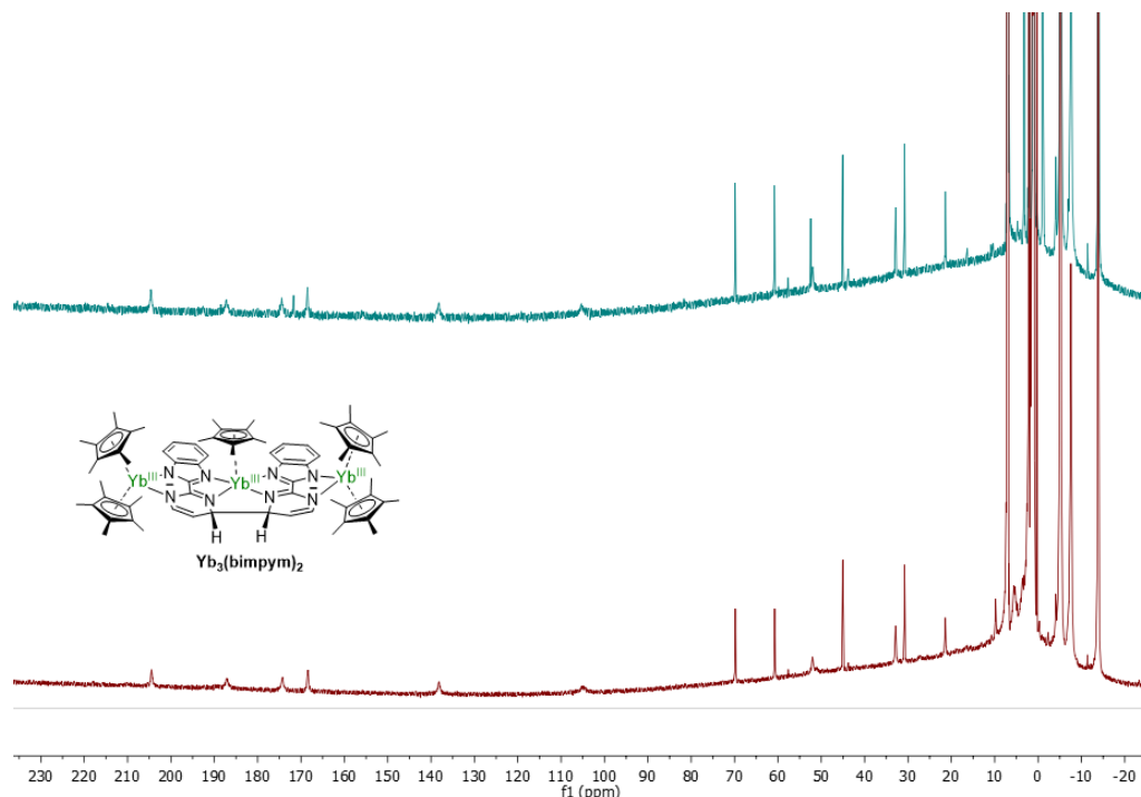
Figure 2.5: Overlay of the spectra of Yb_3(bimpym)_2 and of the second product of the reaction between 1.8 and ytterbocene.
