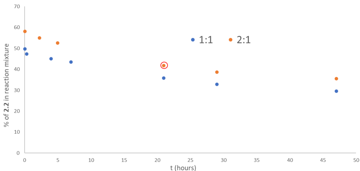
Figure 2.12: Evolution of the proportion of 2.2 with respect to Yb_3(bimpym)_2 in the reaction mixture over time, following in situ reactions with one and two equivalents of ytterbocene. No more ytterbocene could be distinctly identified after 21h (circled in red) in the case of the 2:1 reaction.
