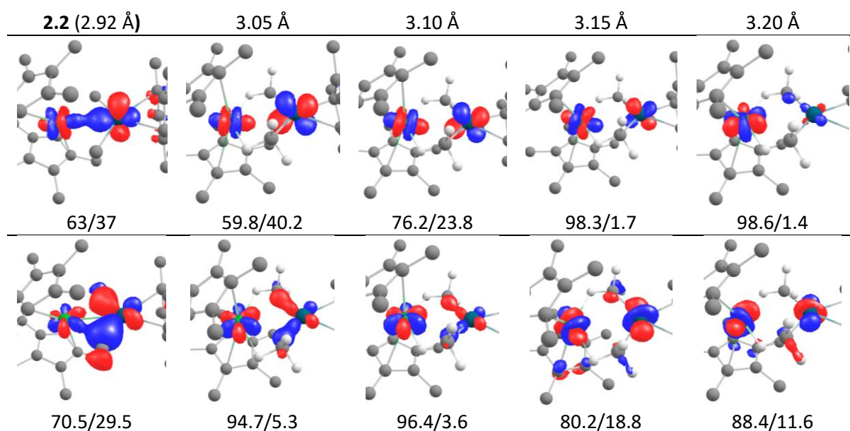
Figure 3.36: Evolution of two CASSCF orbitals across the lengthening of the bond and their relative Yb/Pd contributions (in %). The upper line shows the orbital bearing an interaction between the Pd 4d z 2 and the Yb 4f orbitals and the bottom line shows the methyl-bridged orbital. The Cp* co-ligands are cropped and the complex where d(Yb-Pd) = 3.00 Å is not shown for clarity.
