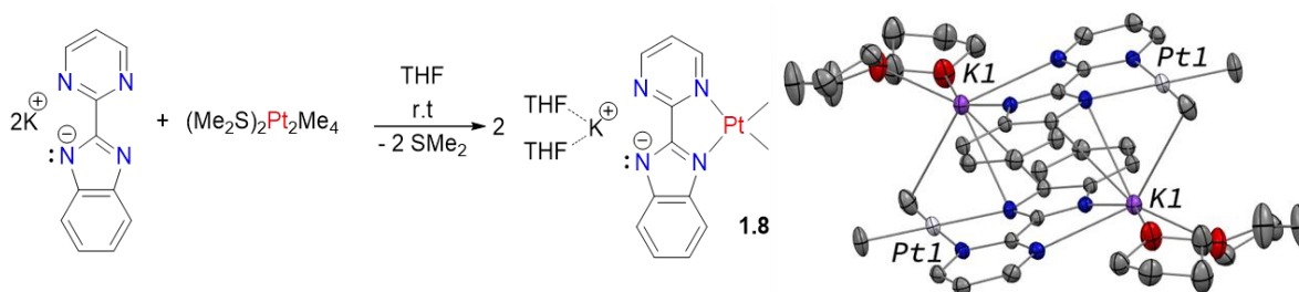
Scheme 1.11: Synthesis and ORTEP of 1.8 . Hydrogen atoms have been hidden for clarity.
