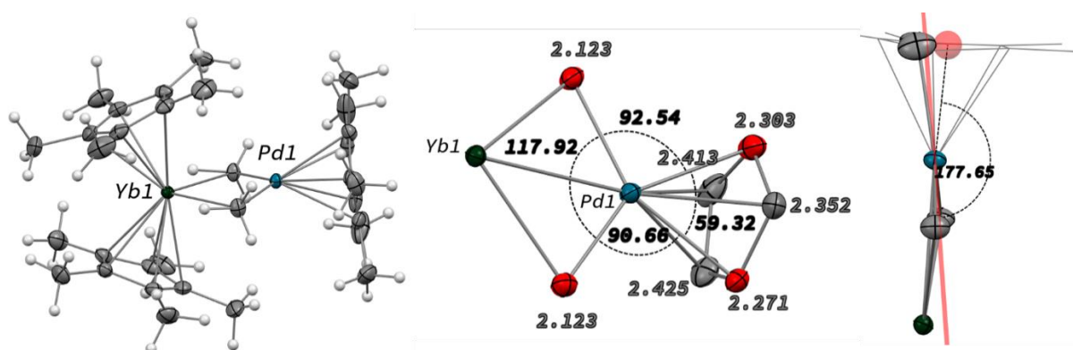
Figure 2.6: Left: ORTEP of 2.2 . Centre: coordination environment of the Pd II , including bond distances and angles between the four coordinating atoms defining the square plane (the composing atoms are shown in red). Right: perspective of the distorted square planar environment, along with the angle formed by Yb, Pd and the centroid of the Cp*.
