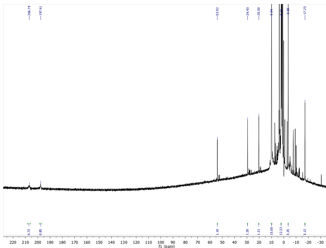
Figure 2.8: ^1H NMR in THF-d_8 of the reaction mixture, following the addition of ytterbocene to 1.9 in THF.
