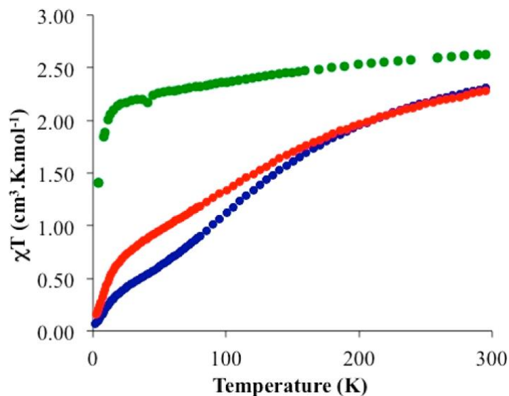
Figure 3.52: Evolution of \chi T over T(K) for a series of Cp^*_2Yb(RAL)PdMe_2 -type complexes. Figure reprinted from ref 65.
