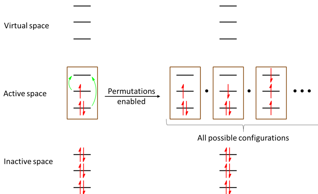
Figure 8: Representation of the principle of multireference CASSCF computations.
