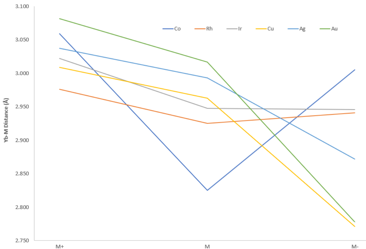
Figure 3.43: Evolution of the Yb-TM distance as a function of the metal charge.
