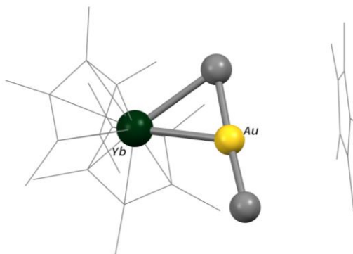
Figure 3.42: Computed geometry of \text{YbAu}^- , which deviate from 2.2 's structure.
