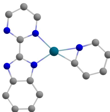
Figure 3.9: Structure of 1.12- \eta^2 , computed at the ZORA1 level of theory.
