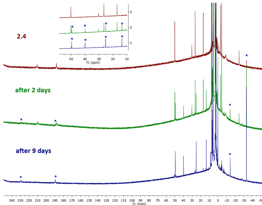
Figure 2.17: Evolution of 2.4 to 2.5 (blue dots), studied by ^1\text{H} NMR in \text{tol}-d_8 .
