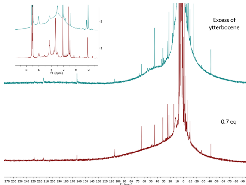
Figure 2.1: In-situ addition of different quantities of ytterbocene to 1.18 in \text{tol-d}_8 , followed by ^1\text{H} NMR.
