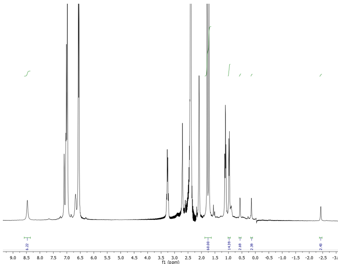
Figure 2.36: ^1\text{H} NMR spectrum in \text{tol-}d_8 of the formed product after the addition of samarocene to 1.12 and free lutidine.
