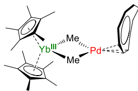
YbPdCNT
