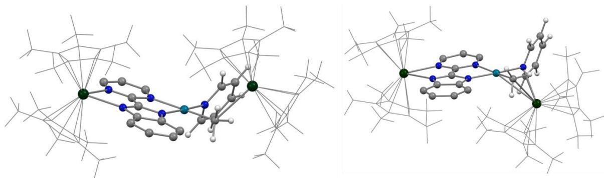
Figure 3.23: Optimised structures of 1.12-Yb 2 and 1.12-Sm 2 . The Cp* co-ligands are shown in wireframe and the majority of H atoms are hidden for clarity.
