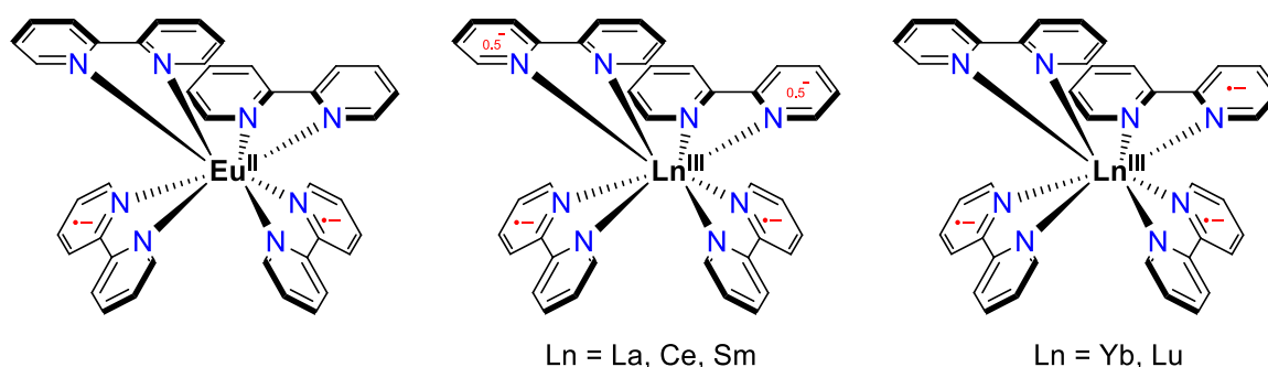
Figure 4: Electronic structures of the [Ln(bipy_4)] compounds with known crystal structures.
