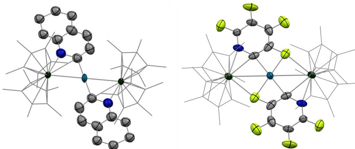
Figure 2.37: ORTEP of 2.8 and 2.9 . The H atoms are hidden and the Cp* co-ligands are shown in wireframe for clarity.
