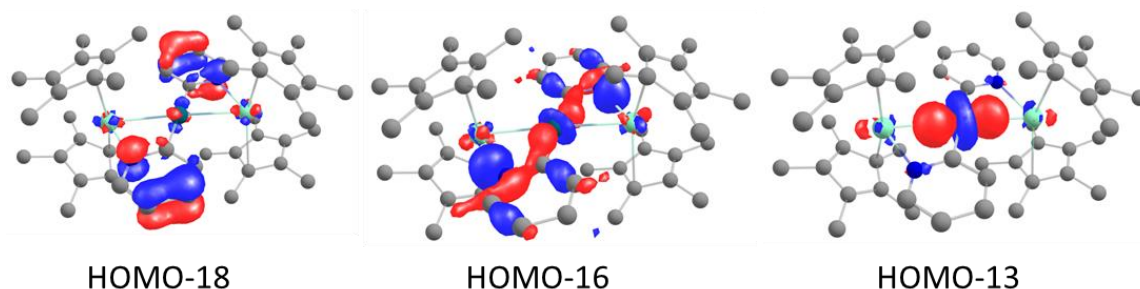
Figure 3.26: Selection of orbitals of 2.7 , computed at the ZORA3 level, containing contributions from both metals.
