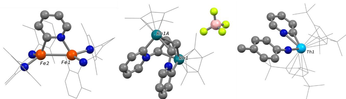
Figure 3.4: Ball and stick representations of some of the examples of organometallic complexes where pyridyl moieties are coordinated. The majority of hydrocarbons are set in wireframe and the hydrogens are not shown for clarity. Colour code for the non-labelled atoms: N – blue, B – pink, F – bright yellow.
