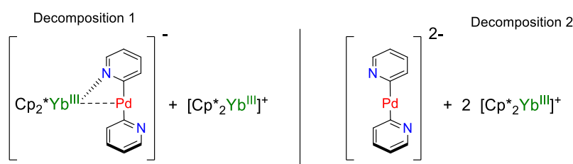
Scheme 3.13: The two proposed decomposition schemes for the EDA analyses.
