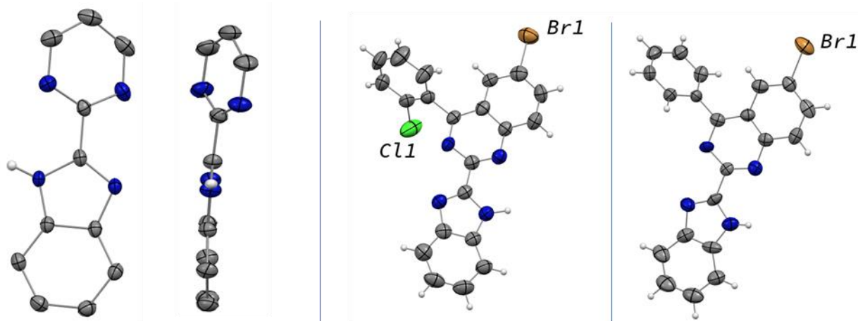
Figure 1.4: Crystal structures of Hbimpym -based systems – Hbimpym (left), Hbimpym-ClBr (centre) and Hbimpym-Br (right). The derived structures were published in a private communication and are available on the CCDC database under the deposition numbers 993427 and 993428.
