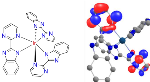
Figure 1.17: Structure and hybridised vacant orbital of Ir(bimpym) 3 .
