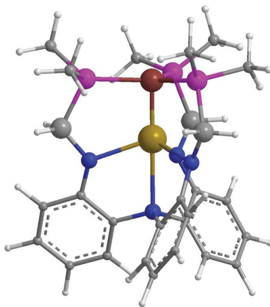
Figure 3.3: Representation of the \{N(o-[NCH_2P(CH_3)_2]C_6H_4)_3\}^{3-} ligand in a heterobimetallic adduct. 32 Colour code: P – purple, N – blue, TM – red, RE – yellow, C – grey, H – white.
