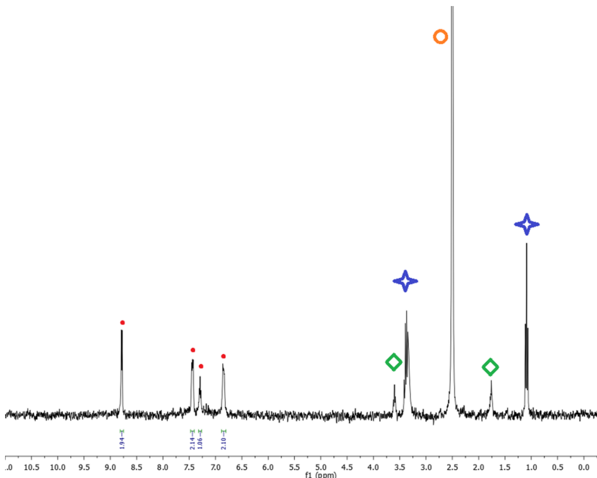
Figure 1.20: ^1\text{H} NMR of the product of the addition of two equivalents of Kbimpym to [\text{Ir}(\text{COE})_2\text{Cl}]_2 in \text{DMSO}-d_6 . The product signals are designated by red dots, the solvent peak by the orange circle, THF – green lozenge and \text{Et}_2\text{O} – blue four-pointed star.
