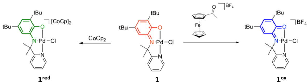
Scheme 2: The chemical transformations yielding the iminoquinone ligand via oxidation (right) or the aminophenolate ligand via reduction (left), starting from the iminosemiquinonato ligand. Adapted from ref 88.
