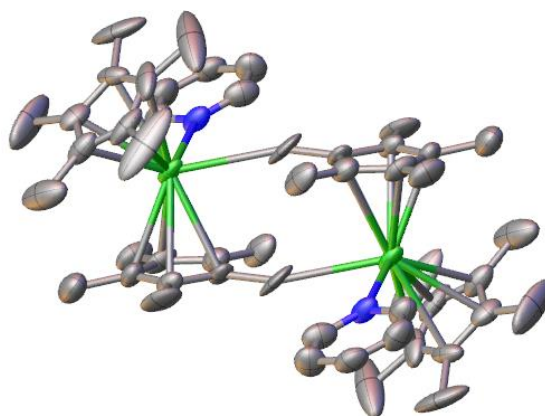
Figure 2.23: ORTEP of the \text{Cp}^*_2\text{Eu}(\text{pyr}) complex and its symmetry-generated interaction with a second molecule.
