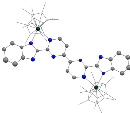
Figure 3.11: ORTEP of 3.1 . The Cp^* co-ligands are displayed in wireframe and the hydrogen atoms are omitted.
