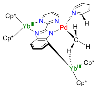
1.12-Yb 2 '
