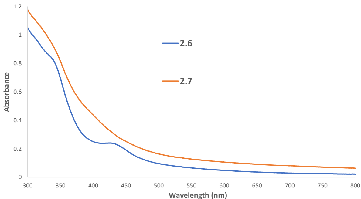
Figure 2.30: UV-Visible data for the trimetallic complexes 2.6 and 2.7 .
