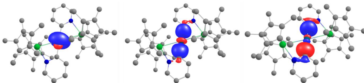
Figure 3.27: Occupied CASSCF orbitals of the active space for 2.6 .
