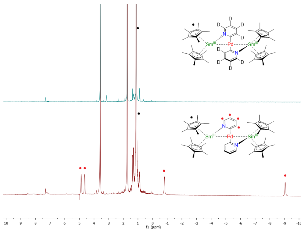
Figure 2.27: ^1\text{H} NMR of 2.7 and 2.7-pyr- d_4 in \text{THF-}d_8 .
