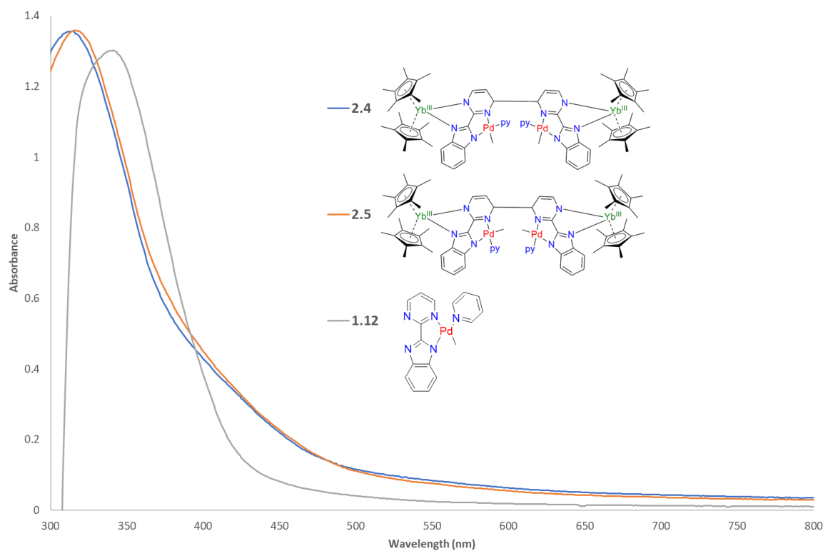
Figure 2.22: UV-Visible spectra of the Pd-pyridine complexes 1.12 , 2.4 and 2.5 .
