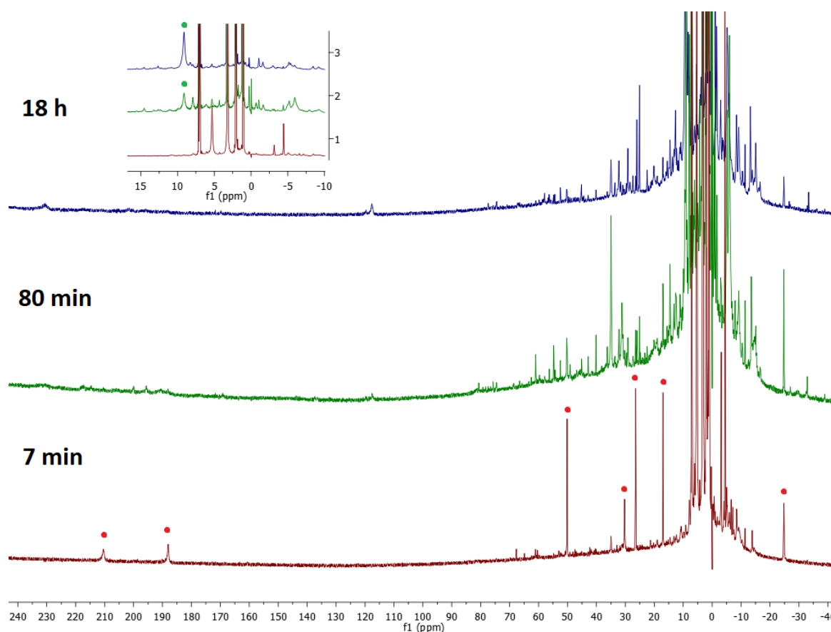
Figure 2.18: ^1\text{H} NMR of the in-situ addition of an equivalent of \text{Cp}^*_2\text{Yb}(\text{OEt})_2 to 1.12 . 2.4 is designated by the red dots. The dominant product formed by the decomposition is designated by the green dot.
