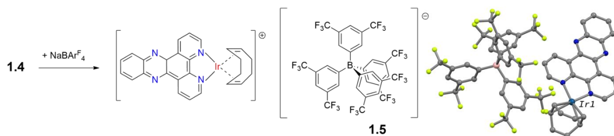
Scheme 1.7: Synthesis and ORTEP of 1.5 .
