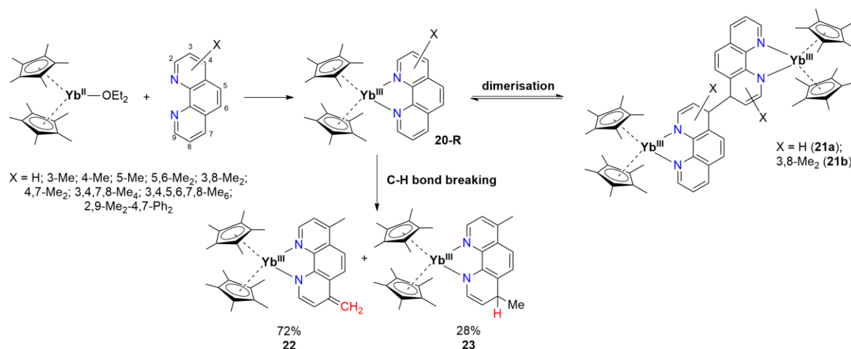
Scheme 11: Formation and reactivity of Yb-phen compounds. The numbering scheme of the substituents is presented as reference.
