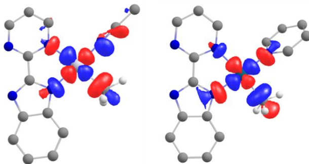
Figure 1.11: Preview of LUMO ab in 1.12 and 1.14 , computed at the ZORA3 level of theory.
