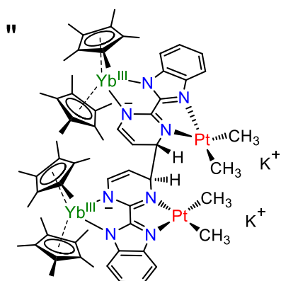
\text{Yb}(\text{bimpym})\text{Pt}
