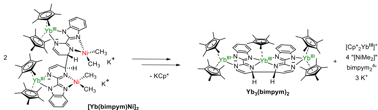
Scheme 2.2: Full account of the main fragments of the reorganisation from [Yb(bimpym)Ni]_2 to Yb_3(bimpym)_2 .
