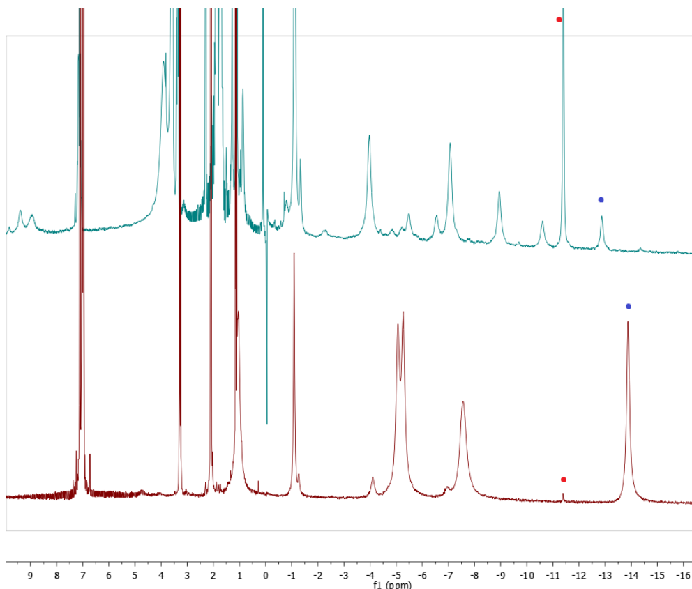
Figure 2.9: Work-up of the reaction leading to the formation of 2.2 . The red dots indicate 2.2 , while the blue ones indicate Yb_3(bimpym)_2 . The ^1\text{H} NMR of the solid after the first recrystallisation in Et_2O – in tol-d_8 – is shown below. The ^1\text{H} NMR of the solid formed in subsequent recrystallisation reactions – in THF-d_8 – is shown above.
