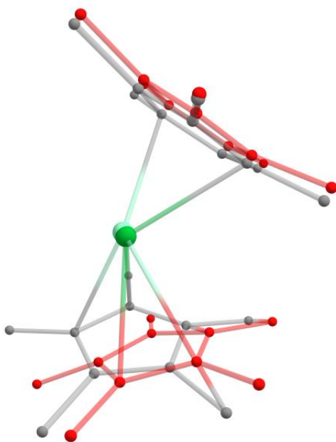
Figure 3.24: Overlay between the second organolanthanide fragment in 1.12-Yb 2 and 1.12-Sm 2 . The C atoms of 1.12-Sm 2 are shown in red.
