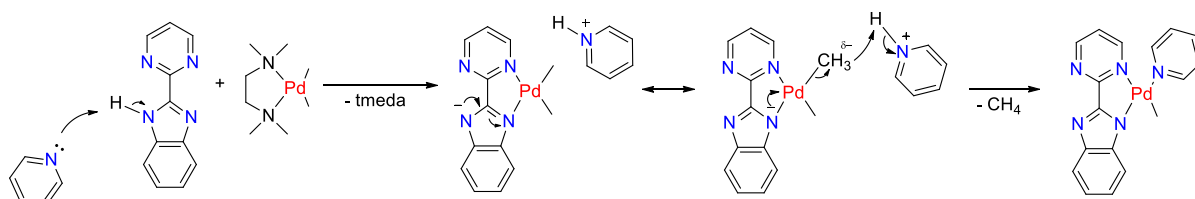
Scheme 1.18: Proposition of the rearrangement mechanism leading to 1.12 .
