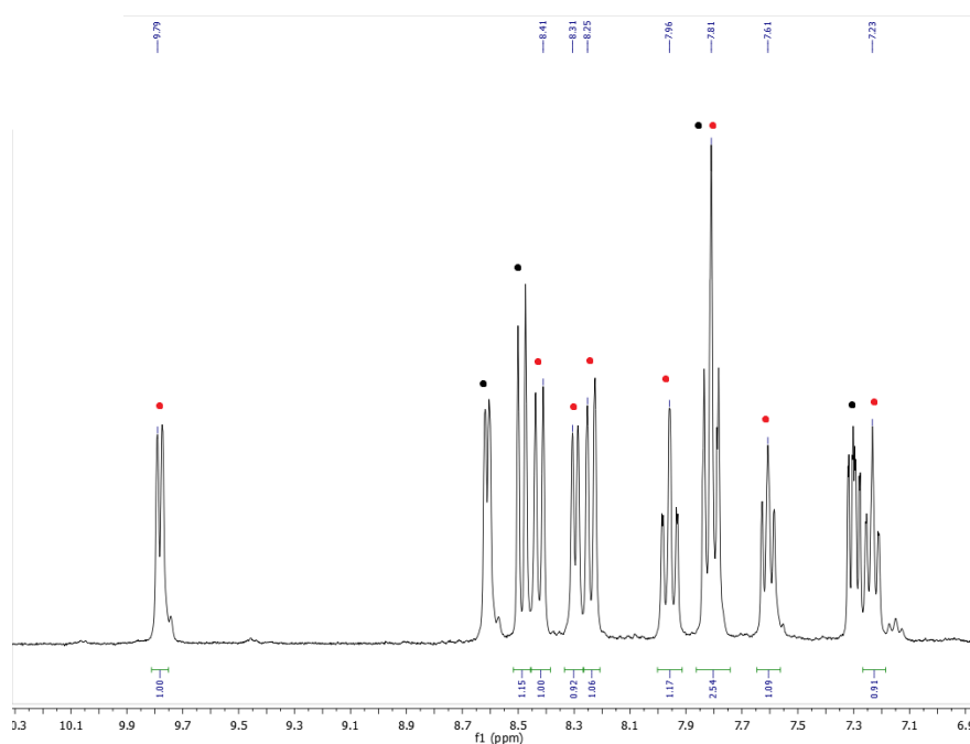
Figure 1.19: In situ ^1\text{H} NMR tracking of the addition of bipy to [\text{Ir}(\text{COE})_2\text{Cl}]_2 – after 15 minutes. Red dots indicate the formed product, black – free bipy.
