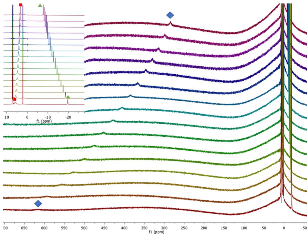
Figure 2.14: Variable temperature ^1H NMR acquisitions for 2.2 . The blue lozenge designates the methyl peak, the red square the YbCp* and the green triangle the PdCp*.
