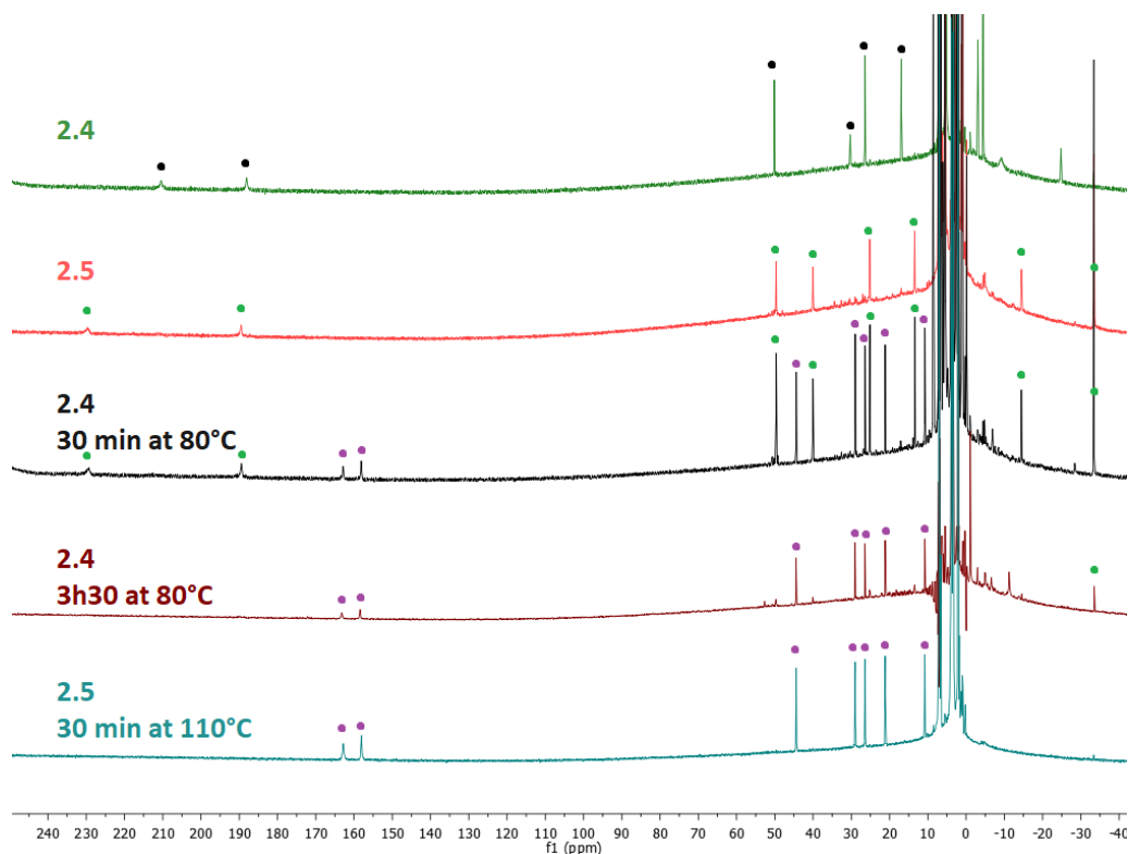
Figure 2.21: High temperature induced evolution of 2.4 and 2.5 towards an unknown compound. Black dots indicate 2.4 , green dots – 2.5 and purple dots – the unknown complex.
