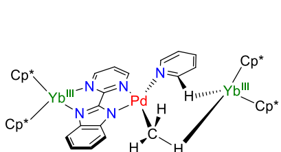
1.12-Yb 2
