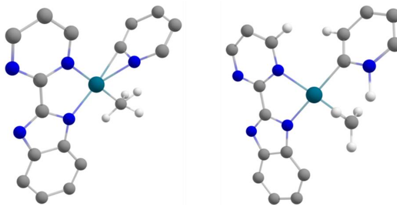
Figure 3.8: Starting geometry (left) and optimised geometry (right) of 1.12-TS2 . The majority of the H atoms were hidden for clarity. On the TS, the H that are left indicate the steric hindrance between the pyridyl moiety and the bimpym ligand.
