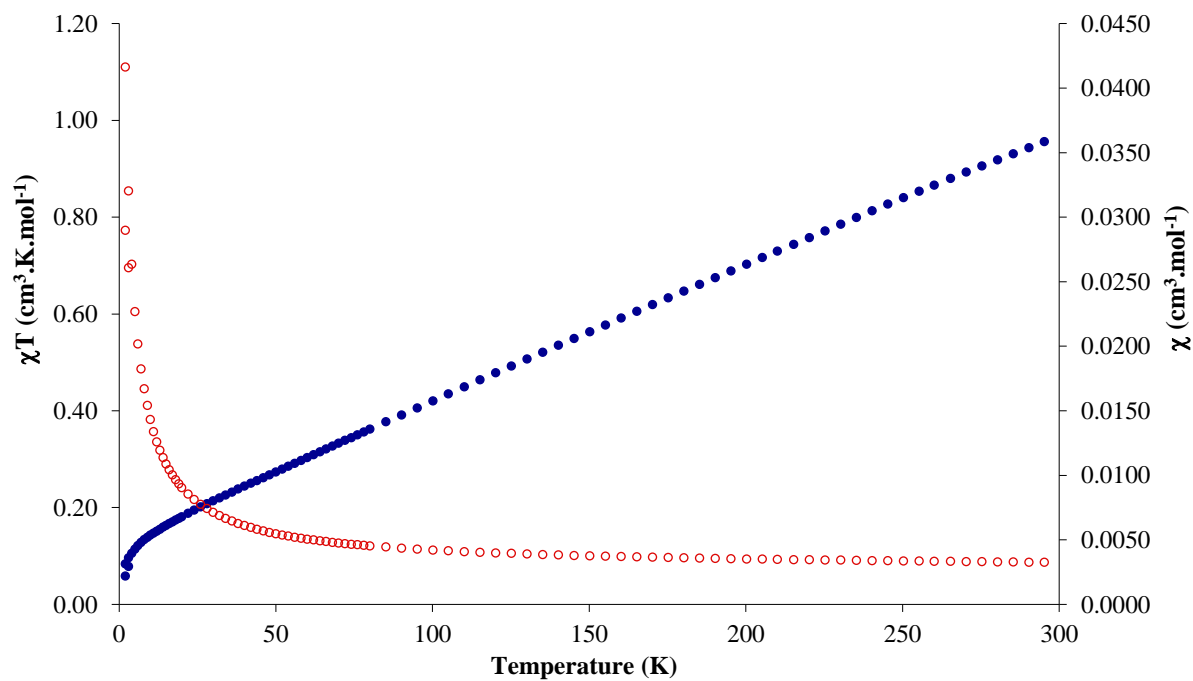
Figure S2: Magnetic susceptibility and the \chi T product for 2.7.
