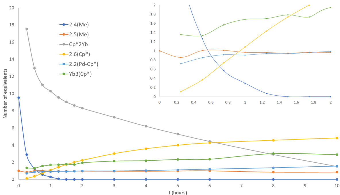
Figure 3.13: Kinetic study of the reaction between 2.4 and an excess of ytterbocene in toluene. t_0 is the scan prior to the addition of ytterbocene, included to show the relative proportions of 2.4 and 2.5 in the initial mixture. The inset shows the evolution of the formed species within the first 2 hours of the reaction. \text{Yb}_3(\text{bimpym})_2 was shortened to “Yb3” in the interest of clarity.
