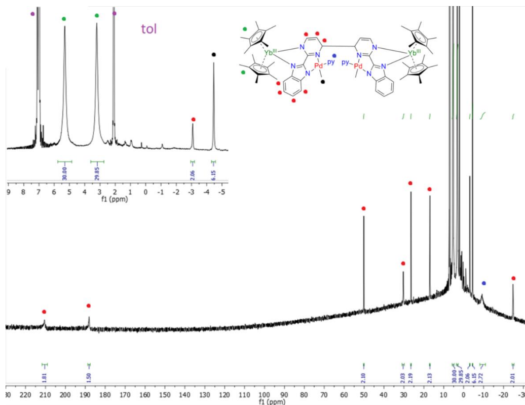
Figure 2.16: ^1\text{H} NMR of 2.4 in \text{tol-d}_8 at r.t.
