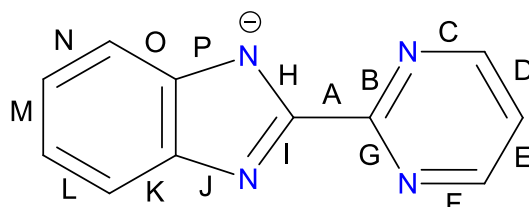
Scheme 1.14: Main bond labelling in bimpym -based ligands.
