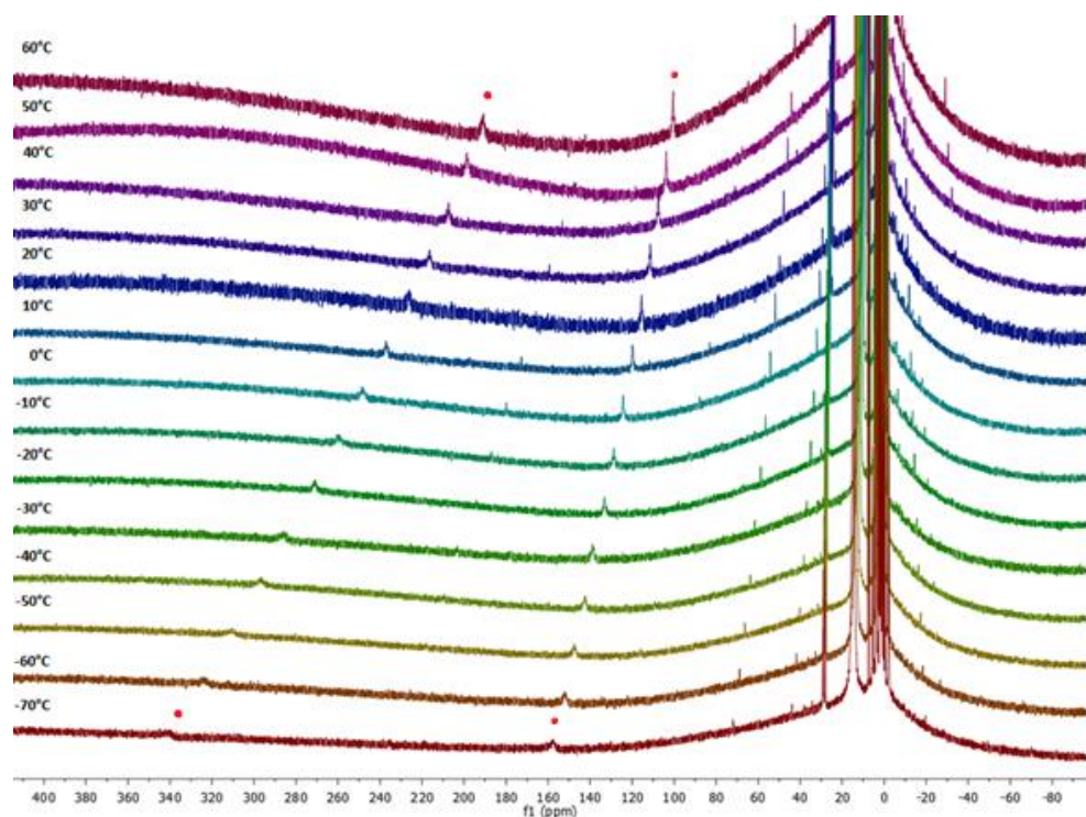
Figure 2.28: Variable temperature ^1\text{H} NMR of 2.6 in \text{THF-}d_8 . Red dots correspond to the pyridyl.
