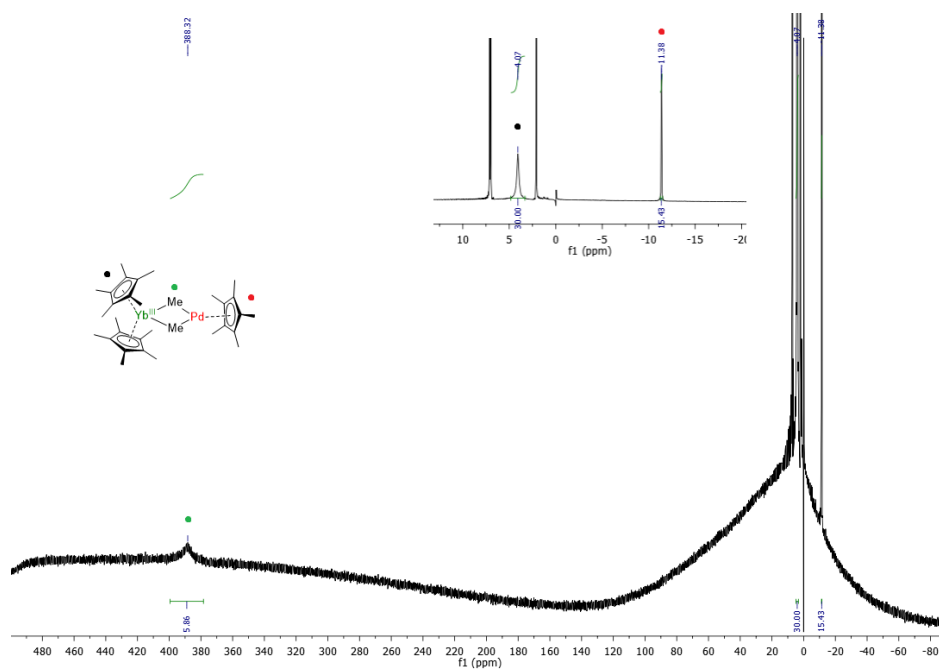
Figure 2.7: ^1H NMR of 2.2 in tol-d_8 .
