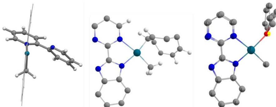
Figure 1.12: Computed complexes analogous to 1.12 with bipy (left), COD (centre) and the overlay (right) between thiophene (the S atom is in yellow and the others are crossed) and furan (atoms not crossed). All complexes were computed at the ZORA1 level of theory.
