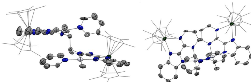
Figure 2.40: ORTEP of 2.14 . The hydrogen atoms are not shown and the Cp* co-ligands are set in wireframe for clarity.
