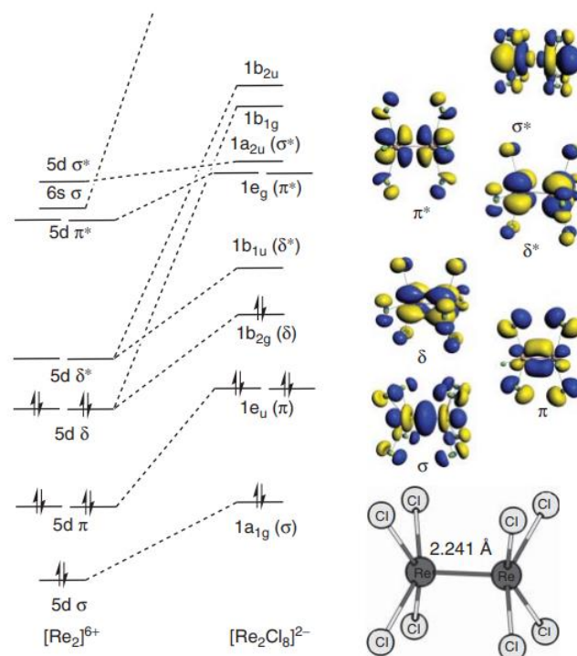
Figure 3.2: Adaptation of Cotton's proposed 8 electronic structure of the [\text{Re}_2\text{Cl}_8]^{2-} architecture. 2
