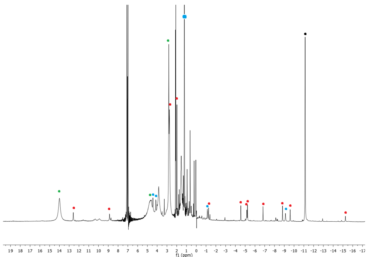
Figure 3.18: ^1\text{H} NMR of the reaction between 2.4 and samarocene. The signals of 2.7 are designated by blue dots, free samarocene – green, assumed H_{\text{bimpym}} – red. The black dot designates the signal very close to that of the Pd-Cp* of 2.2 .
