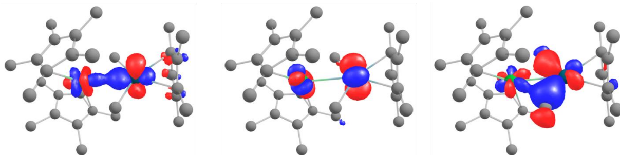
Figure 3.32: Preview of some of the CASSCF orbitals of 2.2 that contain contributions from both metal centres.
