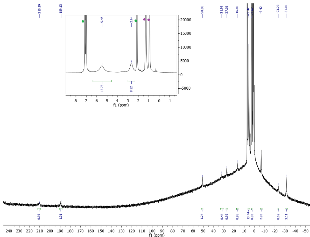
Figure 2.4: ^1H NMR of the red crystals issued from the reaction between 1.8 and ytterbocene. The green dots in the inset correspond to solvent peaks; the purple ones to n-pentane.
