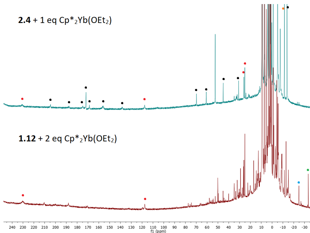
Figure 3.12: Comparison between the in situ reactions of 2.4 and 1.12 with ytterbocene after approximately 18h. Colour code: red – 2.6 ; black – \text{Yb}_3(\text{bimpym})_2 ; orange – 2.2 ; blue – 2.4 ; green – 2.5 .
