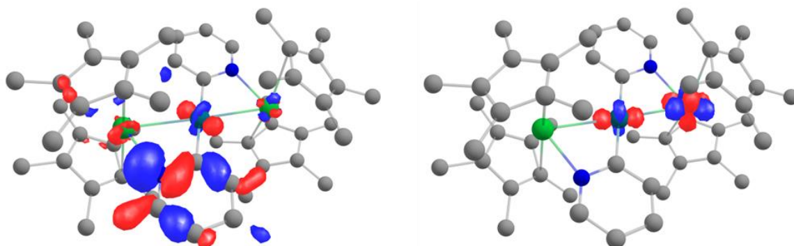
Figure 3.28: CASSCF-generated orbitals of 2.6 , which contain contributions from both the Pd and the Yb metal centres.
