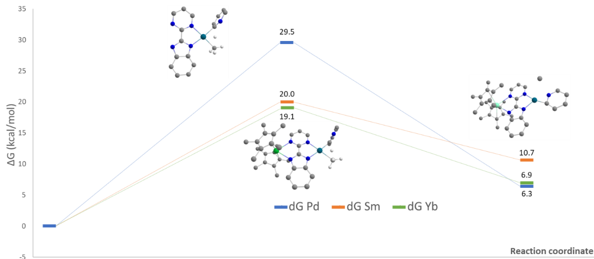
Figure 3.22: Computed Gibbs Free Energy profile, at the TS1 level of theory, of the C-H activation on 1.12 -based structures.
