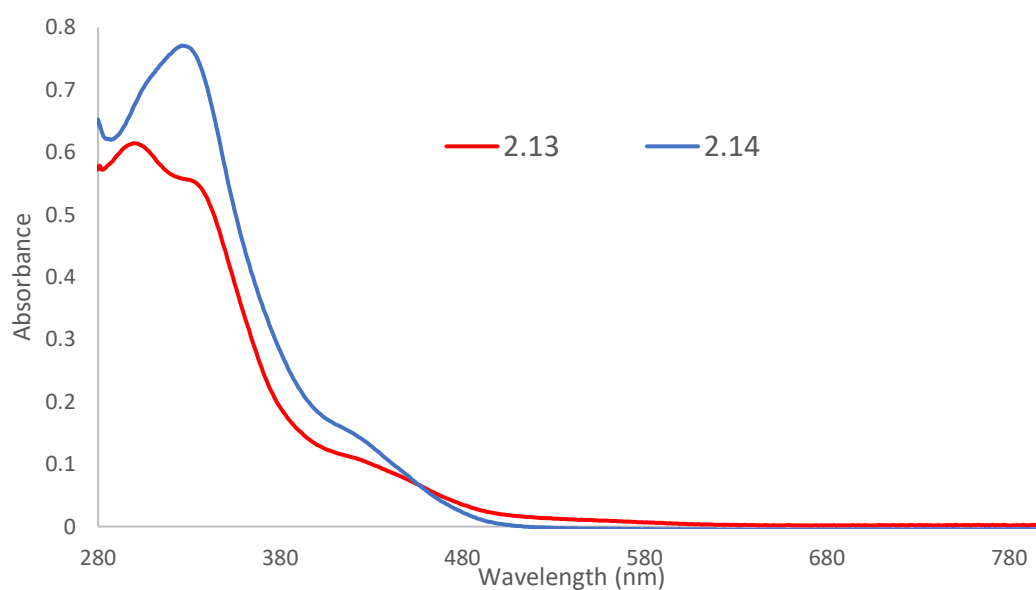
Figure 2.43: UV-Visible spectra of 2.13 and 2.14 .
