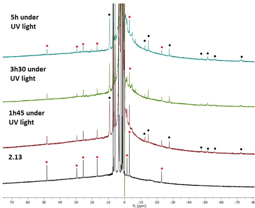
Figure 2.45: Evolution of the mixture containing 2.13 and ytterbocene under UV light after different periods of time. The peaks of 2.13 are designated by the red dots, whilst the new signals are designated by the black dots.
