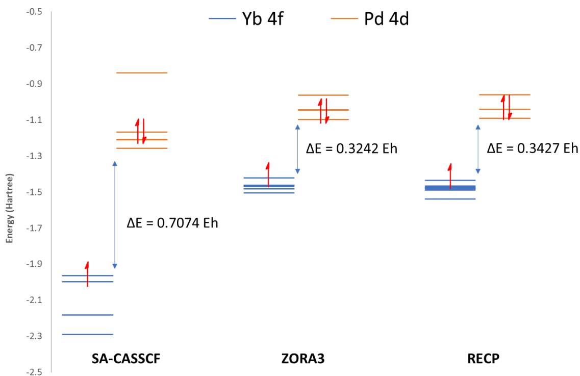
Figure 3.51: Energy levels of the Yb III 4f (blue) and Pd II 4d orbitals, computed at multiple levels of theory. In the interest of clarity, only the electrons of the SOMO/HOMO are shown.
