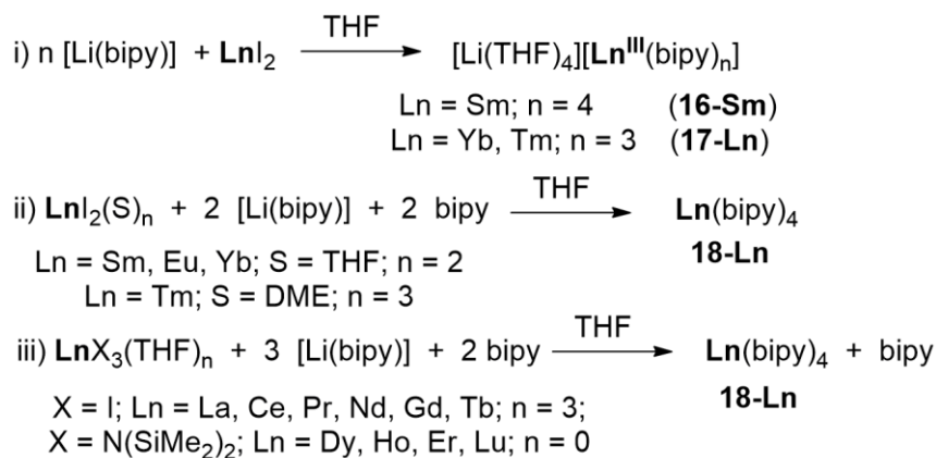
Scheme 7: Preparation of neutral or anionic Ln(bipy) 4 complexes. 129–132
