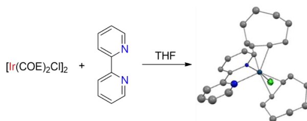
Scheme 1.26: Addition of bipy to [\text{Ir}(\text{COE})_2\text{Cl}]_2 and the ORTEP of the resulting structure.
