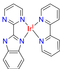
(\text{bimpym})\text{Ir}(\text{bipy})
