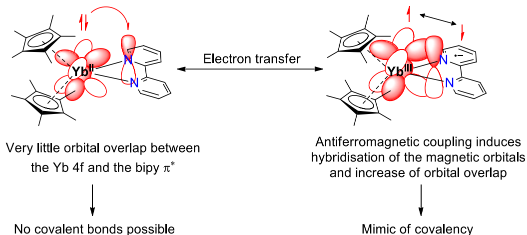
Scheme 9: Representation of the formation of the closed-shell singlet upon electron transfer in the \text{Cp}^*_2\text{Yb}(\text{bipy}) complex.
