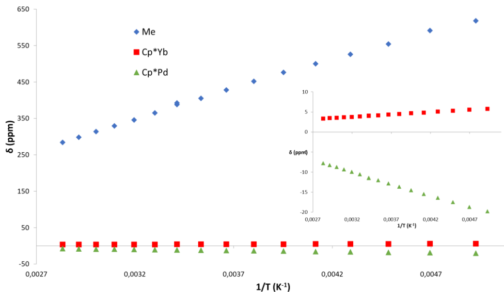
Figure 2.13: Variable temperature ^1H NMR of 2.2 – \delta over 1/T . The evolution of the signals near 0 ppm is shown in the inset.
