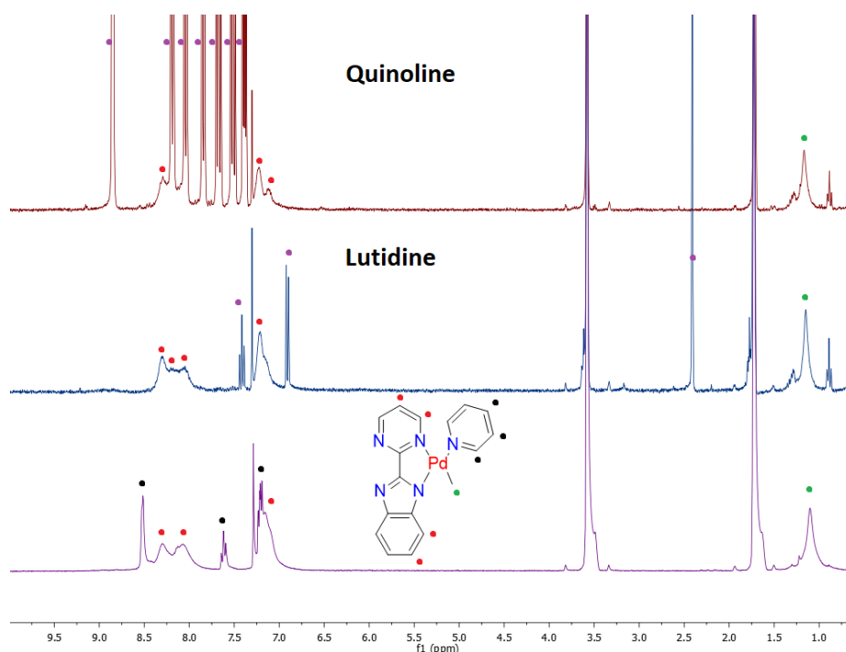
Figure 2.32: ^1\text{H} NMR of 1.12 and the lutidine and quinoline precursors in \text{THF-d}_8 . The red dots indicate the bimpym peaks, black dots – pyridine, green – methyl and purple – pyridine analogue peaks.
