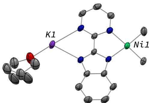
Figure 1.3: ORTEP of K(bimpym)NiMe 2 . Hydrogen atoms have been hidden for clarity. The THF molecule present in the crystal structure is disordered.
