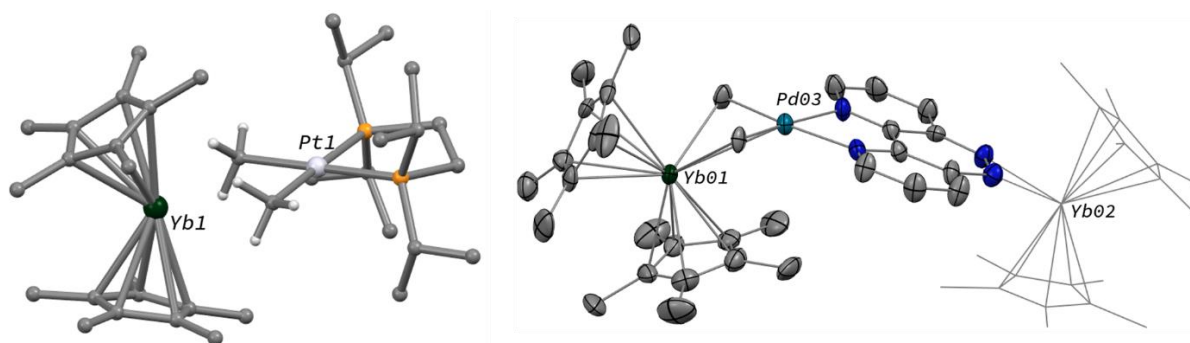
Figure 3.16: ORTEP of two complexes where \text{Cp}^*_2\text{Yb} fragments coordinate methyl moieties. 60,61
