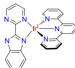
(\text{bimpym})\text{Ir}(\text{terpy})
