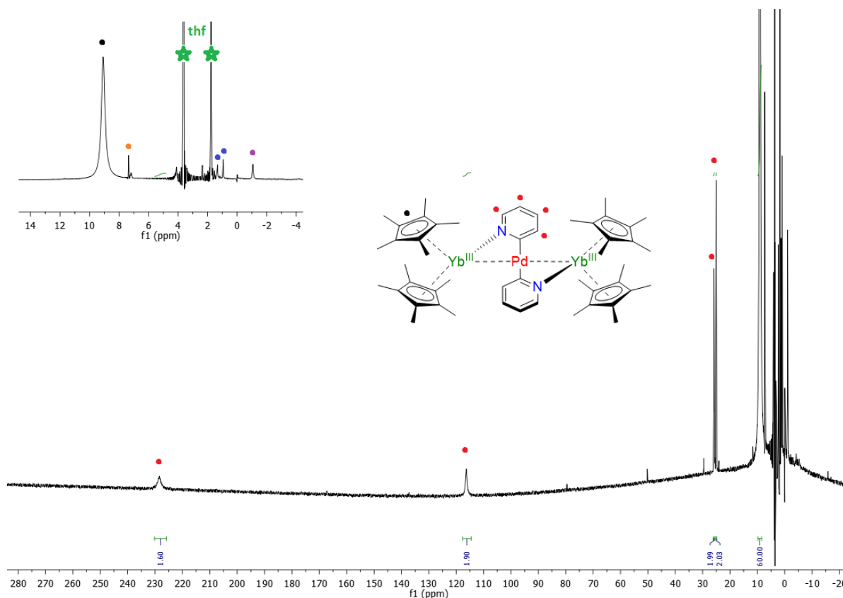
Figure 2.26: ^1\text{H} NMR of complex 2.6 in \text{THF-d}_8 at 293 K. Red and black dots indicate the pyridyl peaks and the \text{Cp}^* peak. The trace impurities have the following colours: blue – H grease, orange – residual toluene and purple – unknown impurity.
