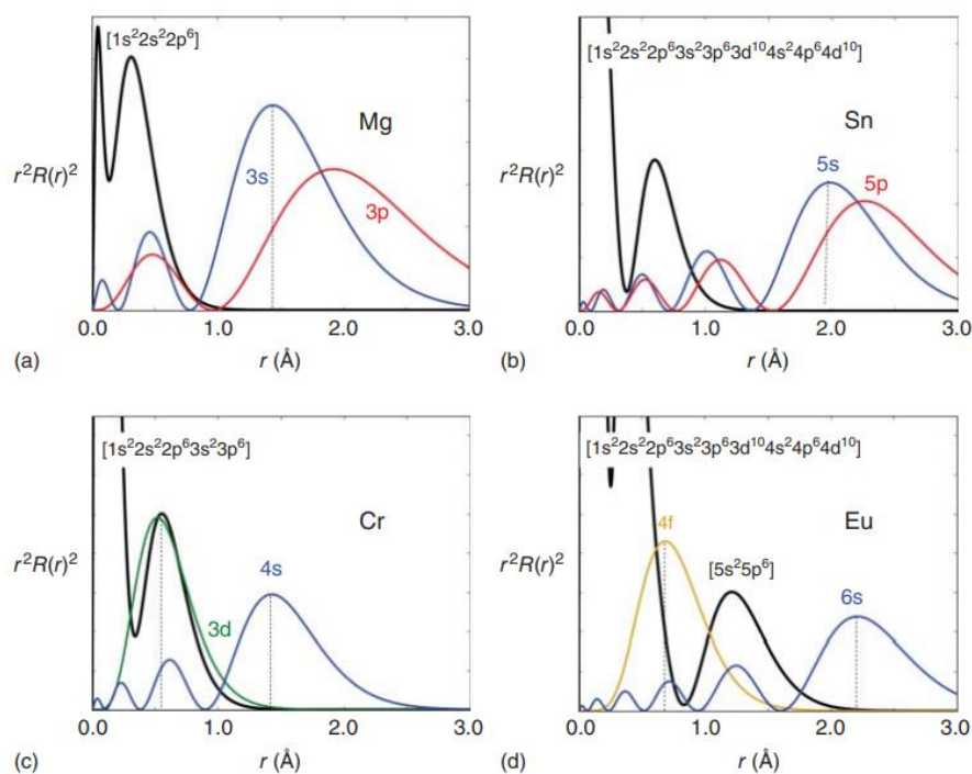
Figure 3.1: Radial distribution functions of the valence orbitals in the (a) s-(Mg), (b) p-(Sn), (c) d-(Cr), and (d) f-(Eu) blocks of the periodic table. Black lines correspond to the core density. Reprinted from ref 2.
