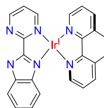
(\text{bimpym})\text{Ir}(3,3'\text{-bipy})
