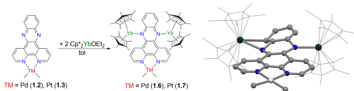
Scheme 1.8: Synthesis of 1.6 and 1.7 and the ORTEP of 1.7 . The Cp* co-ligands are drawn in wireframe and the hydrogen atoms are omitted for clarity.
