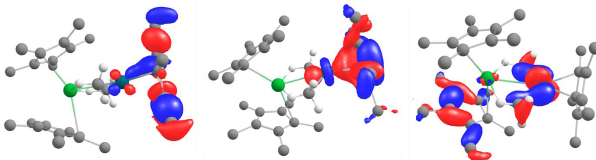
Figure 3.31: Involvement of Pd 4d electrons in bonding interactions, below the active space.
