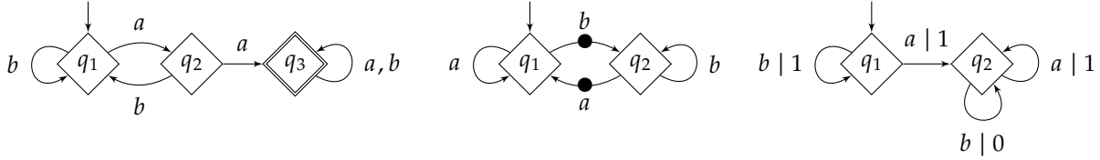
Figure 2.7: Three kinds of deterministic automata considered in this thesis. We use diamonds to represent automaton states (as for memory states). The initial state is indicated with an ingoing arrow. Final states (in F ) of DFAs are represented with a double border. Büchi transitions (in B ) of Büchi automata are decorated with a bullet \bullet . A transition of a parity automaton from q to q' with label c \mid k means that \delta(q, c) = q' and p(q, c) = k .
