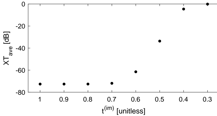
FIGURE 5.13: The average total cross-talk X_{ave} predicted by CMT model for Fermat multi-core fibers with different taper ratios.
