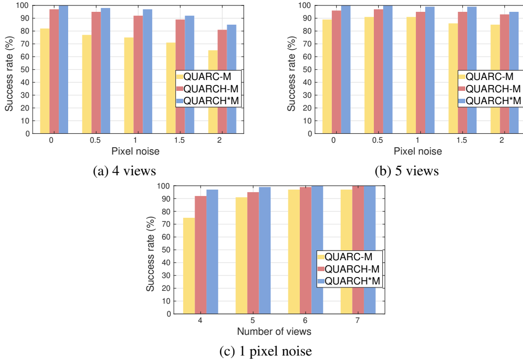
Figure 4.6: Benefits of QUARCH and the LMI-constrained optimization. QUARCH*M denotes our algorithm. QUARCH-M and QUARC-M are its variants using an unconstrained optimization. QUARC-M uses a QUARC plane as initialization.
