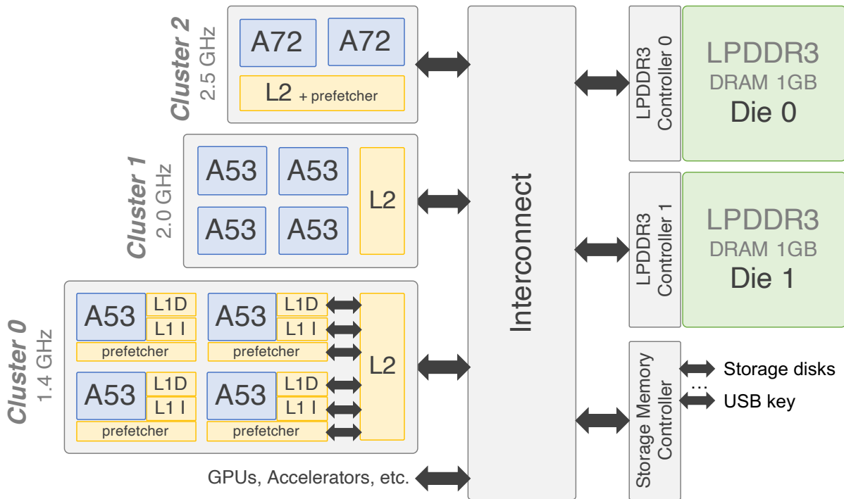
Figure 2.2: Heterogeneous multi-core architecture of the MediaTek Helio X20.
