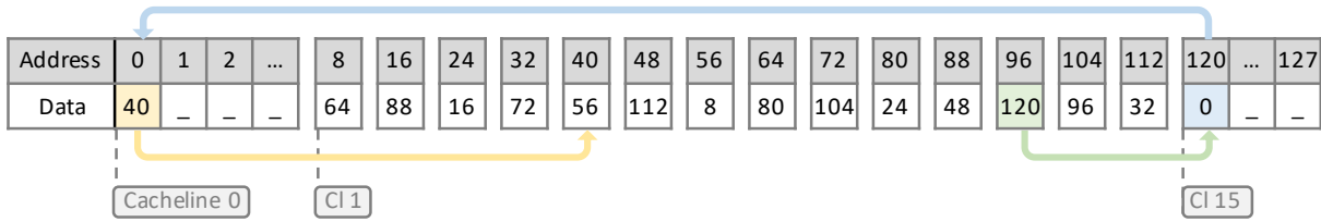
Figure 5.7: Microbenchmark pointer chasing implementation.
