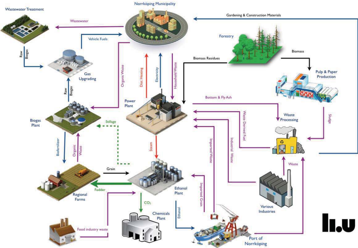
Figure 2. The Händelö industrial symbiosis network. Source: LiU (2020).
