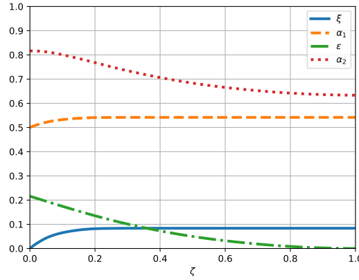
Figure 3.1: Variation of \epsilon , \xi , \alpha_1 and \alpha_2 with respect to the parameter \zeta . The closer \zeta is to 0 the lower the reward of the unwanted couples (e_{i^\star}, e_{i^\star}) and (e_{j^\star}, e_{j^\star}) , the closer \zeta is to 1 the higher the rewards of the unwanted couples. The dimension d of the arm-set is 10 (which gives linear reward with unknown parameter \theta_\star of dimension 100). The plotted curve represents the average value of the parameters over 100 different matrices \mathbf{M}_\star initiated randomly with positive values.
