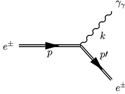
Figure 2.4: Strong field Feynman diagram of the nonlinear Compton scattering process.
