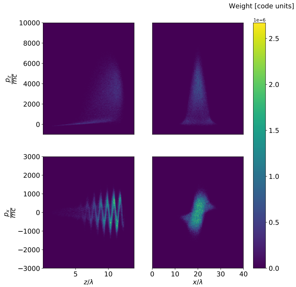
Figure 5.8: Phase space of the created positrons at the end of the simulation, for a CP gaussian beam with a_0 = 2000/\sqrt{2} and \gamma_\gamma = 400 . The axis of propagation of the beam is z .
