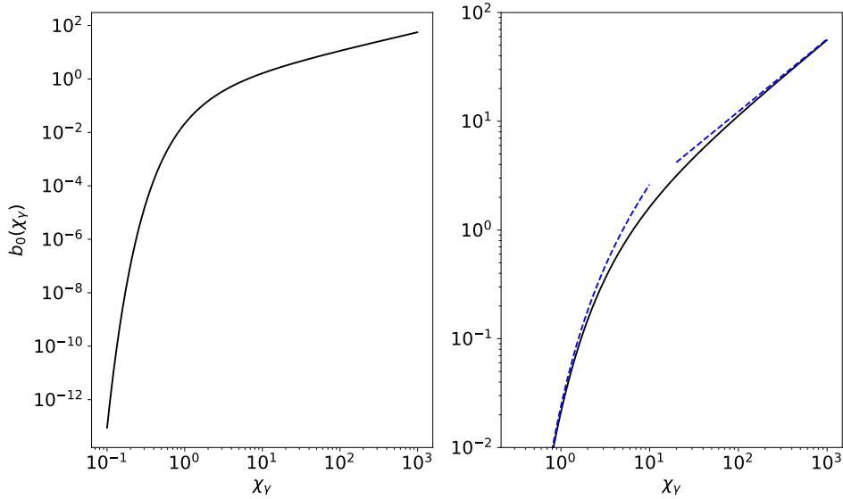
Figure 2.3: (a) Dependence of b_0(\chi_\gamma) on the photon quantum parameter \chi_\gamma as defined by Eq. (2.44). (b) Zoom on the region where b_0 > 0.01 , the blue dashed lines are representing its asymptotic behaviour given by Eqs. (2.45) and (2.46)
