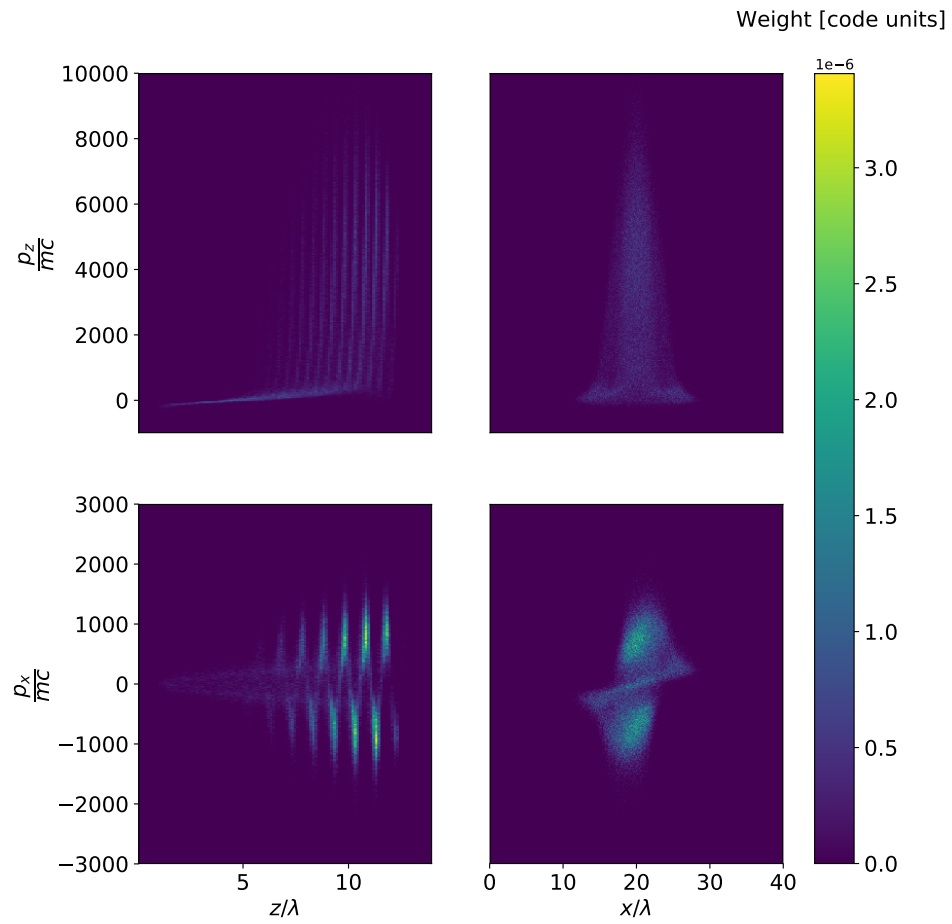
Figure 5.6: Phase space of the created positrons at the end of the simulation, for a LP gaussian beam with a_0 = 2000 and \gamma_\gamma = 400 . The axis of propagation of the beam is z and the beam is polarised along x .
