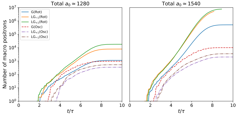
Figure 7.10: Number of positrons as a function of time in the simulations for the different field configurations with two LG beams, for two different total intensities at focus a_{0,tot} \simeq 1280 (left) and a_{0,tot} \simeq 1540 (right).
