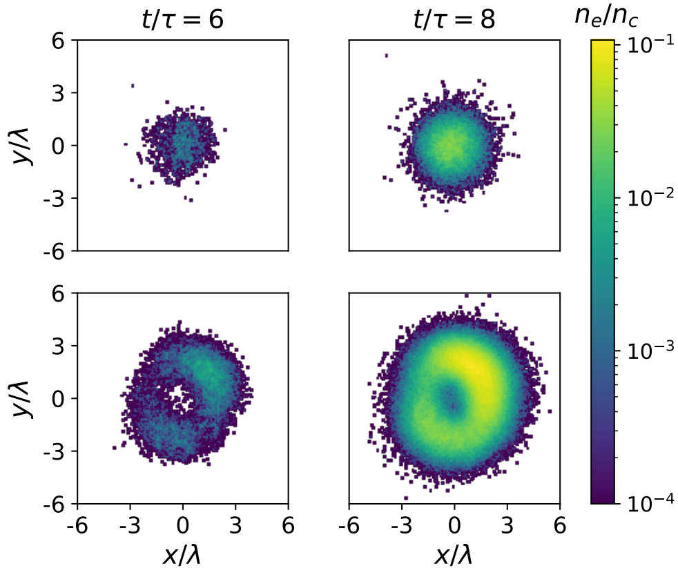
Figure 7.11: Density of the positrons at two different times in the focal plane, for the G(Rot) and LG -1 (Rot) cases, with a_{0,tot} = 1540 .
