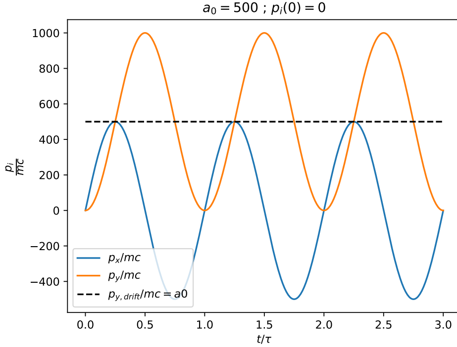
Figure 6.1: Representation of the classical components of the momentum as a function of time, for a positron initially at rest in a rotating electric field. The drift momentum, orthogonal to the initial direction of the electric field, is represented in dashed black. The field amplitude is a_0 = 500 .
